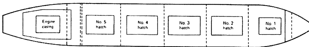
(b) Plan
