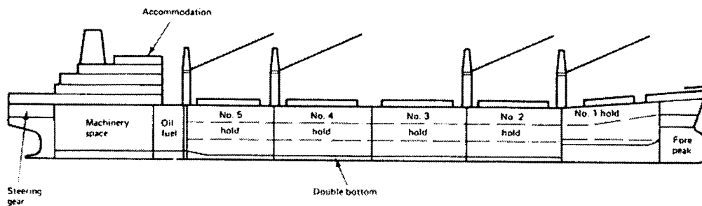
(a) Elevation
