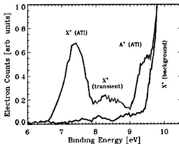
Figure 7. Photoelectron spectrum of transient wave packet in dissociating \text{Br}_2 .
