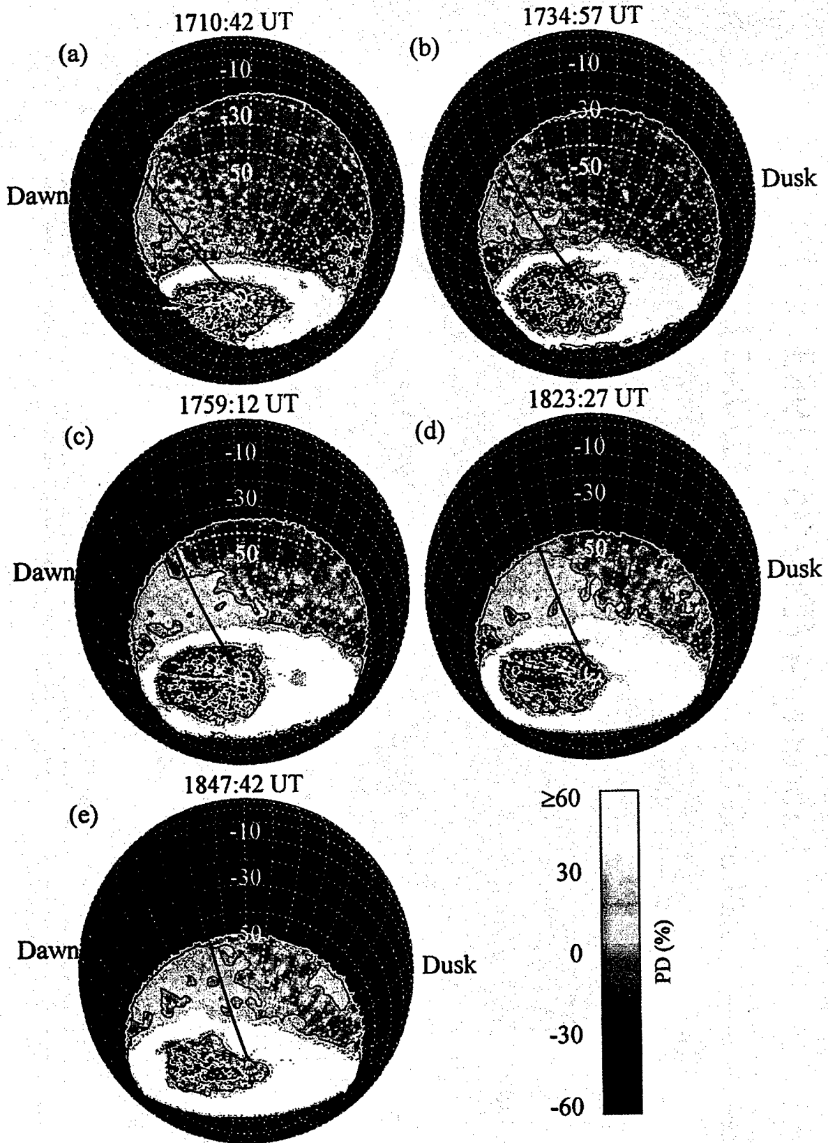
Plate 2. PD values for storm onset. Plotted PD values are from images smoothed with a 3x3 pixel moving filter. The dark line indicates 120°W geographic longitude, the meridian selected for particular study in later discussion. The noon-midnight meridian bisects each image vertically, with the morning sector to the left.
