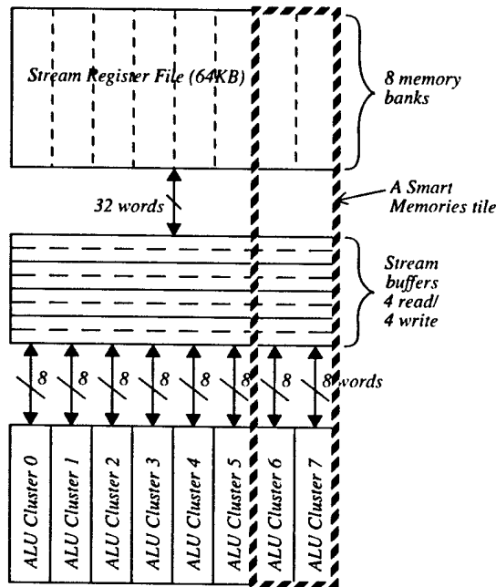
Figure 8. Imagine architecture
