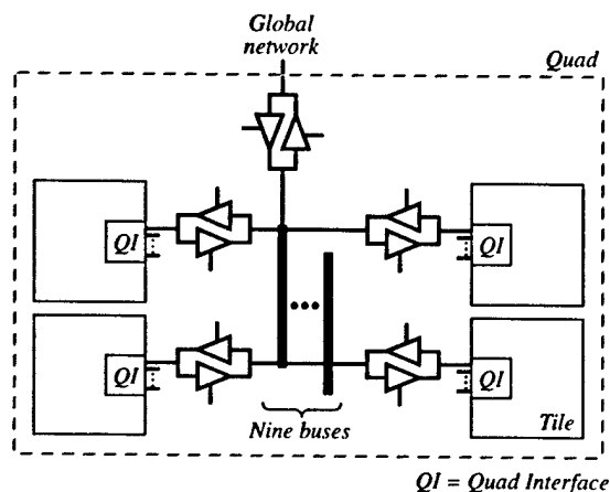
Figure 5. Quad interconnection network
