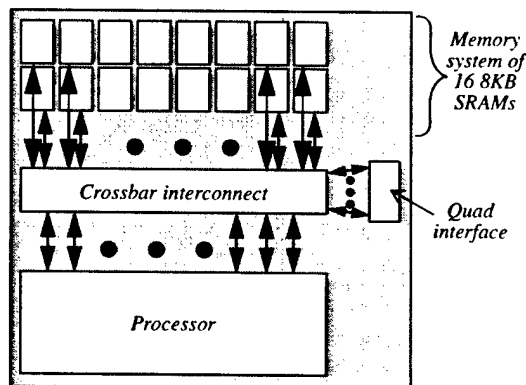
Figure 2. Tile floorplan
