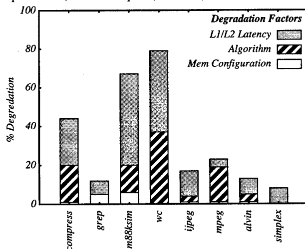
Figure 12. Performance degradation
