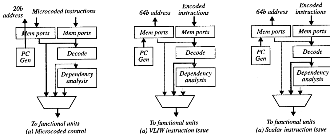
Figure 7. Instruction path
