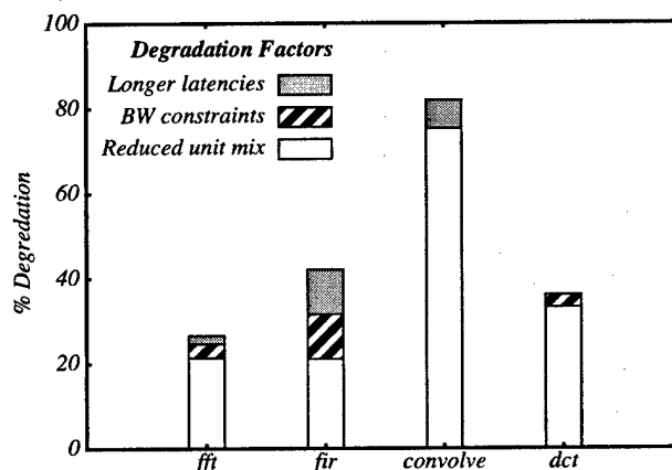
Figure 9. Performance degradation
