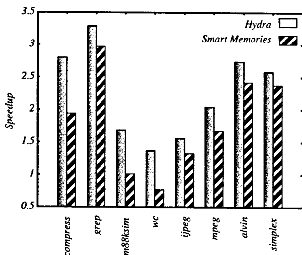
Figure 13. Speedup
