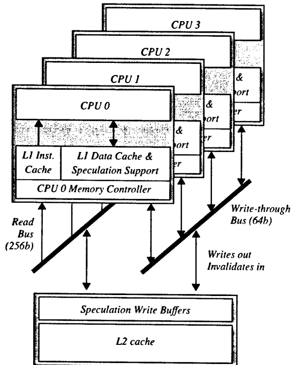
Figure 10. Hydra architecture
