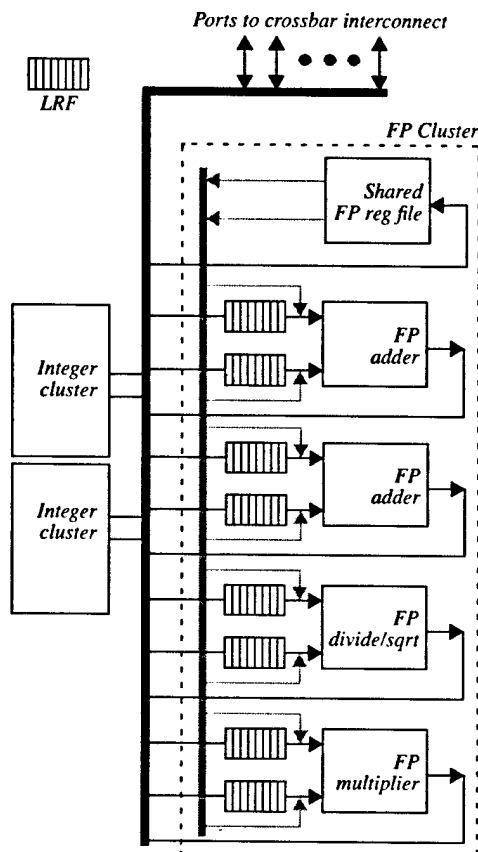
Figure 6. Smart Memories compute resources
