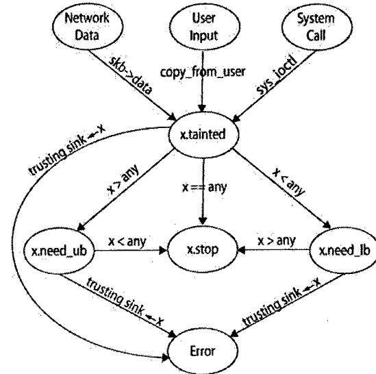
Figure 3: Approximate range checker.
