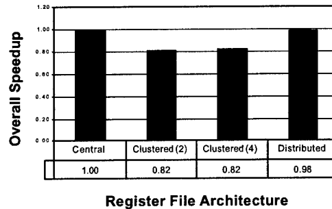
FIGURE 29. Overall Speedup vs. Register File Architecture
