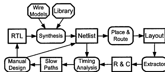
Figure 1: Flow of automated design
