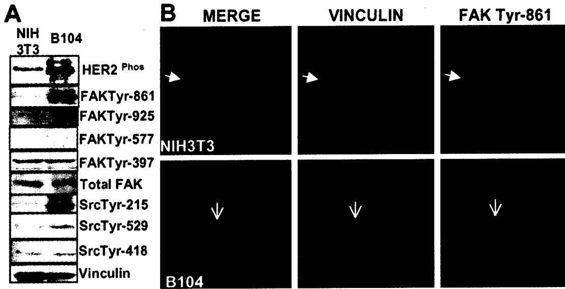
Fig. 3. Analysis of signaling pathways in NIH 3T3 cells expressing constitutively activated HER2. A: Western blot analysis. NIH 3T3 cells and B104 cells (NIH 3T3 cells expressing activated HER2) [13] were lysed and analyzed using phospho-specific antibodies against the indicated molecules. B: Confocal microscopy analysis. The status and localization of FAK Tyr-861 was studied in NIH 3T3 cells and B104 cells. FAK Tyr-861 is shown in red and vinculin, a marker of focal adhesions, is shown in green. Thick arrows point to localization of FAK Tyr-861 in dot-like focal adhesions in NIH 3T3 cells. Empty arrows point to the cytoplasmic localization of FAK Tyr-861.
