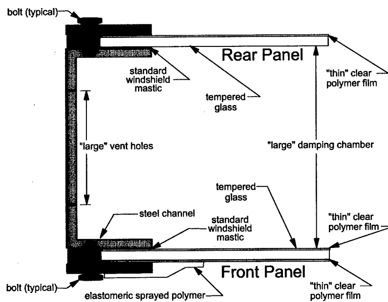
Figure 4. First Generation Window, Design 4.
