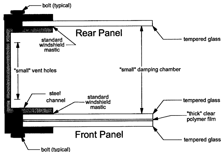
Figure 1. First Generation Window, Design 1.
