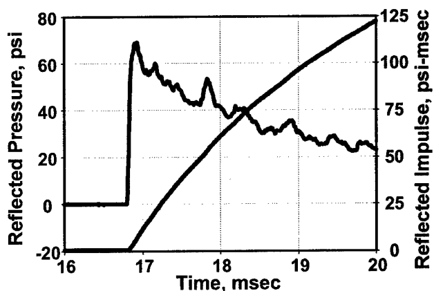
Figure 8. Typical P-I Curve, front gauge.
