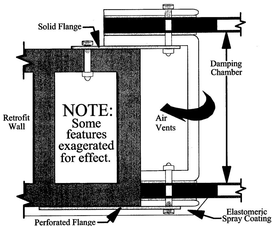
Figure 17. Second Generation Window, Anchor Design 5.
