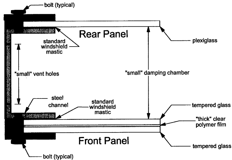
Figure 2. First Generation Window, Design 2.
