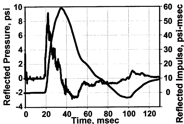
Figure 10. Typical P-I Curve, back gauge.
