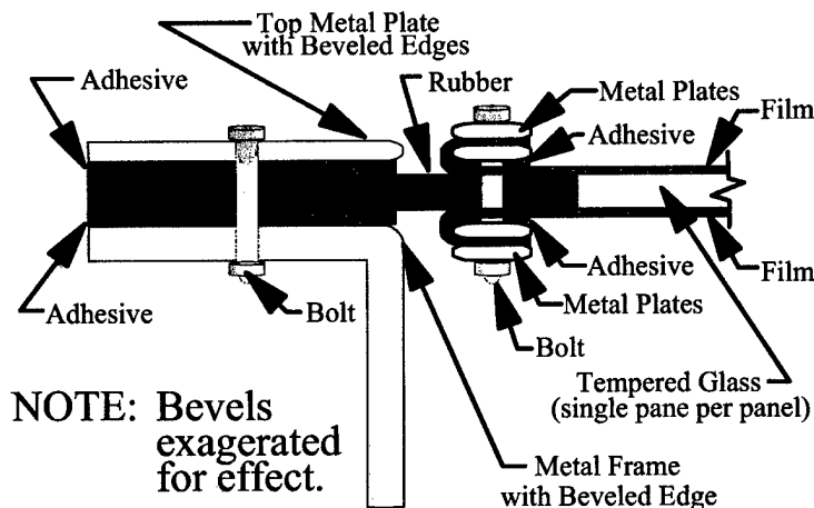
Figure 15. Second Generation Window, Anchor Design 4.
