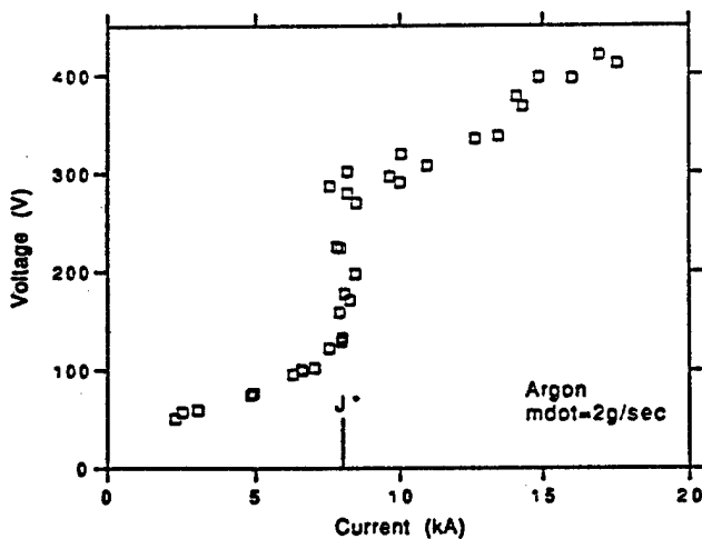
Fig. 7 Voltage-Current Characteristic
