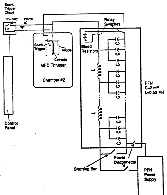
Fig. 3 Electrical System
