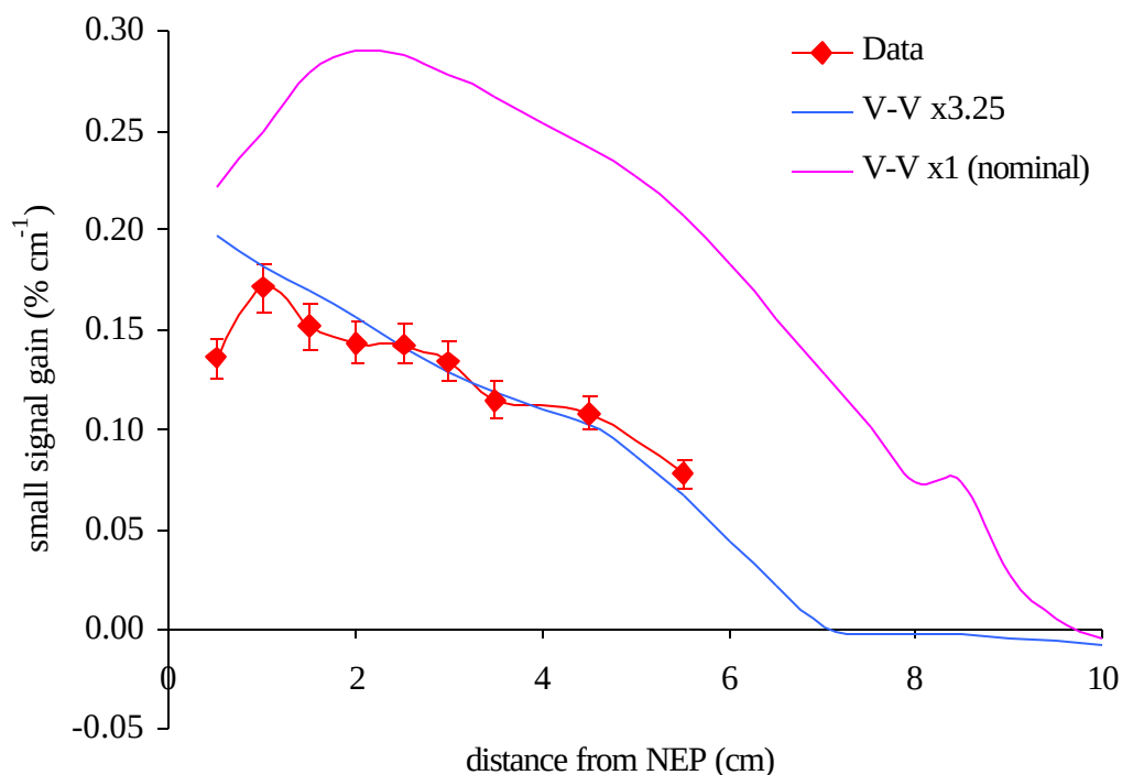
Figure 5.70 Measured and predicted peak gain with V-V rate constant adjustment for the ( F_2=2 , H_2= 27 ) flow conditions. Error bars represent 6% bias and 0.002 \text{ \% cm}^{-1} precision uncertainties.
