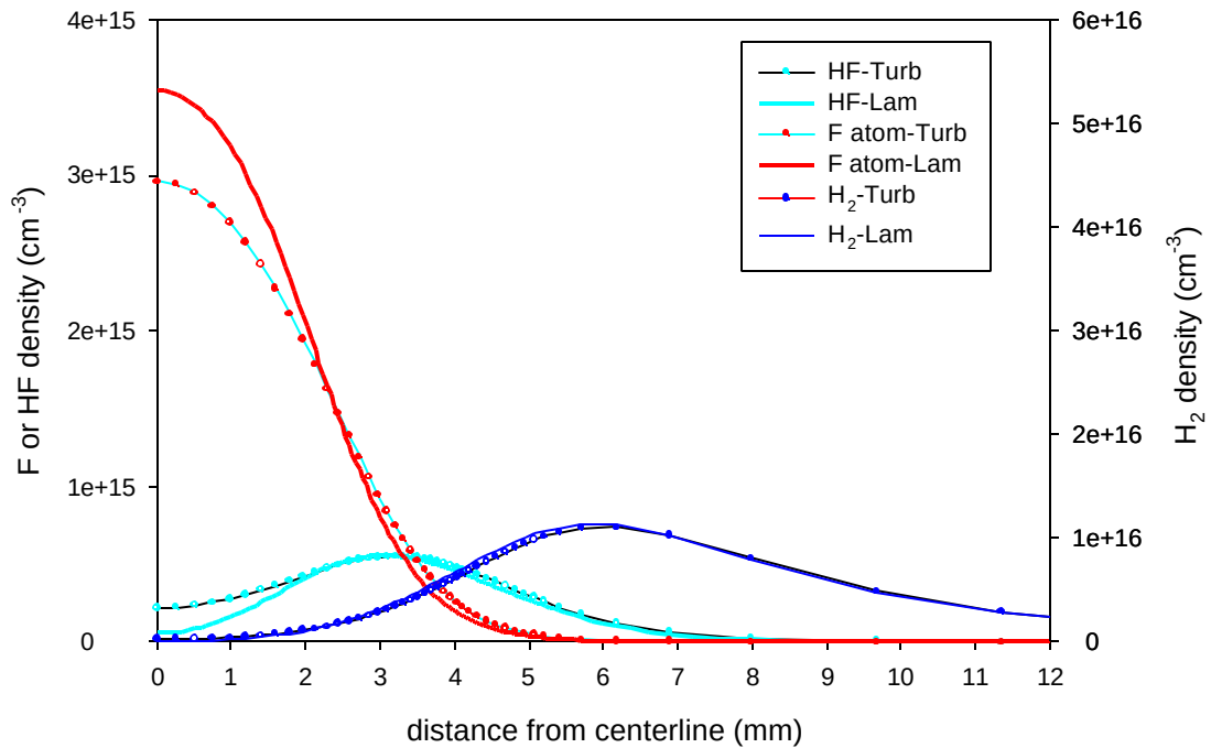
Figure 5.30 Predicted vertical concentration profiles 6.0 cm downstream of the NEP for the ( F_2=2 , H_2=10 ) flow conditions. Turbulent modeling case has 1% initial turbulence intensity.
