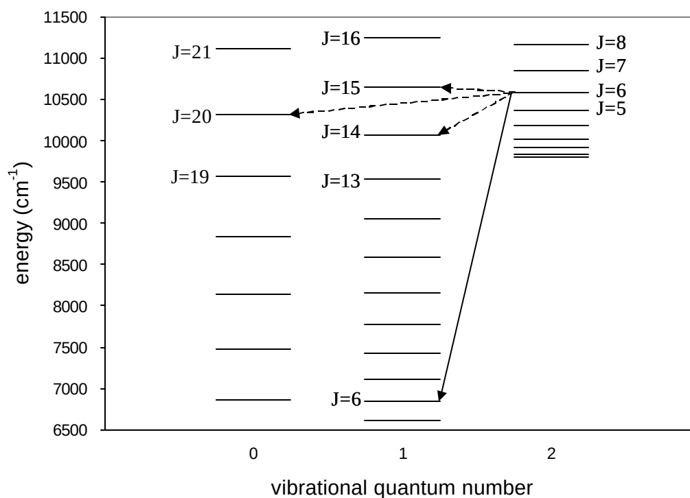
Figure 2.6 \text{HF}(v) + \text{HF}? \text{HF}(v-1) + \text{HF} energy transfer routes. Solid arrow represents “true” V-T energy relaxation process. Broken arrows represent near-resonant V-R energy transfer.
