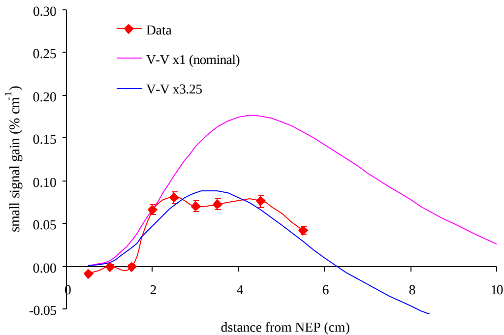
Figure 5.73 Measured and predicted centerline gain with V-V rate constant adjustment for the ( F_2=3 , H_2=10 ) flow conditions. Error bars represent 6% bias and 0.002 \text{ } \% \text{ cm}^{-1} precision uncertainties.
