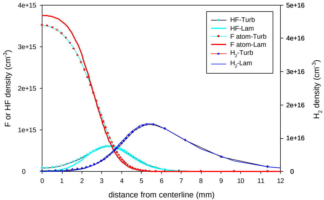
Figure 5.29 Predicted vertical concentration profiles 4.0 cm downstream of the NEP for the ( F_2=2 , H_2=10 ) flow conditions. Turbulent modeling case has 1% initial turbulence intensity.
