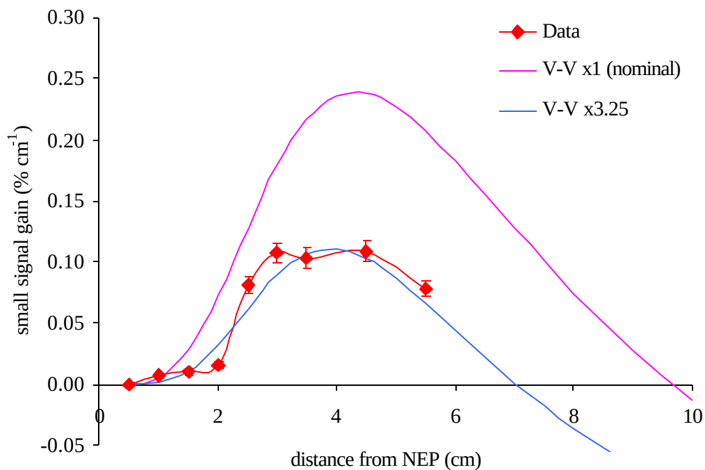
Figure 5.71 Measured and predicted centerline gain with V-V rate constant adjustment for the ( F_2=2 , H_2= 27 ) flow conditions. Error bars represent 6% bias and 0.002 \text{ \% cm}^{-1} precision uncertainties.
