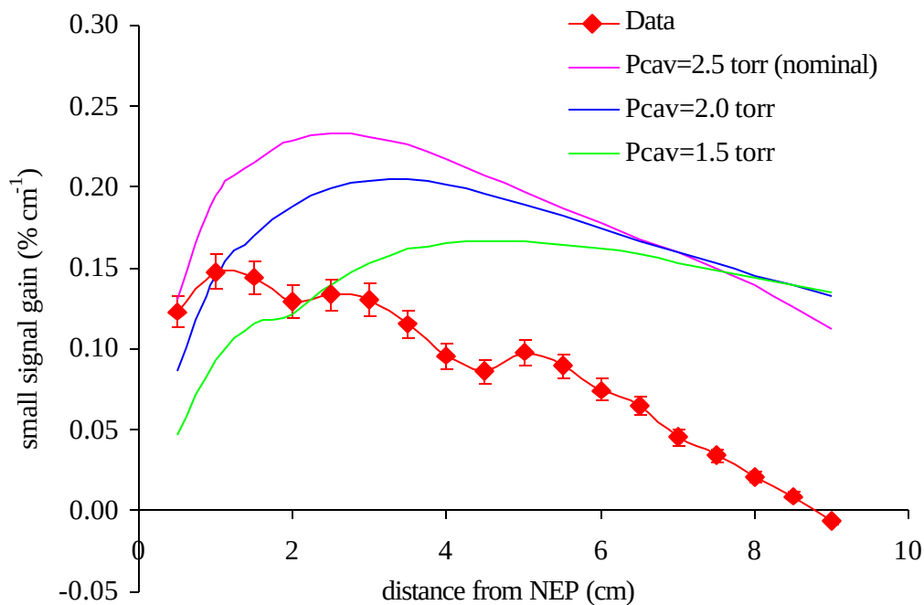
Figure 5.48 Measured and predicted peak gain at different cavity pressures for the (F 2 =2, H 2 =10) flow conditions. Error bars represent 6% bias and 0.002 % cm -1 precision uncertainties.
