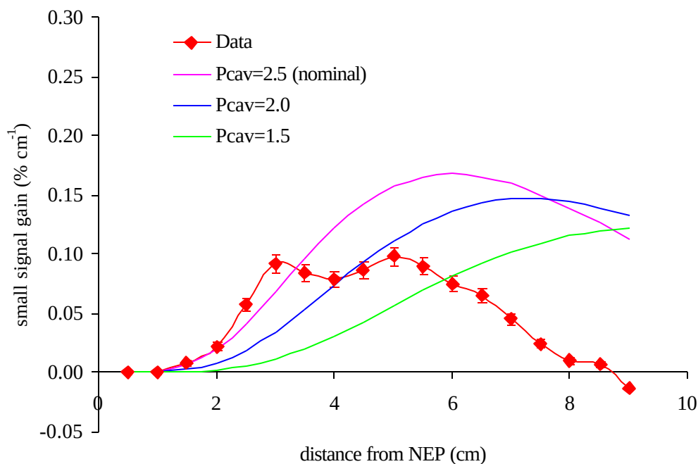
Figure 5.49 Measured and predicted centerline gain at different cavity pressures for the (F 2 =2, H 2 =10) flow conditions. Error bars represent 6% bias and 0.002 % cm -1 precision uncertainties.
