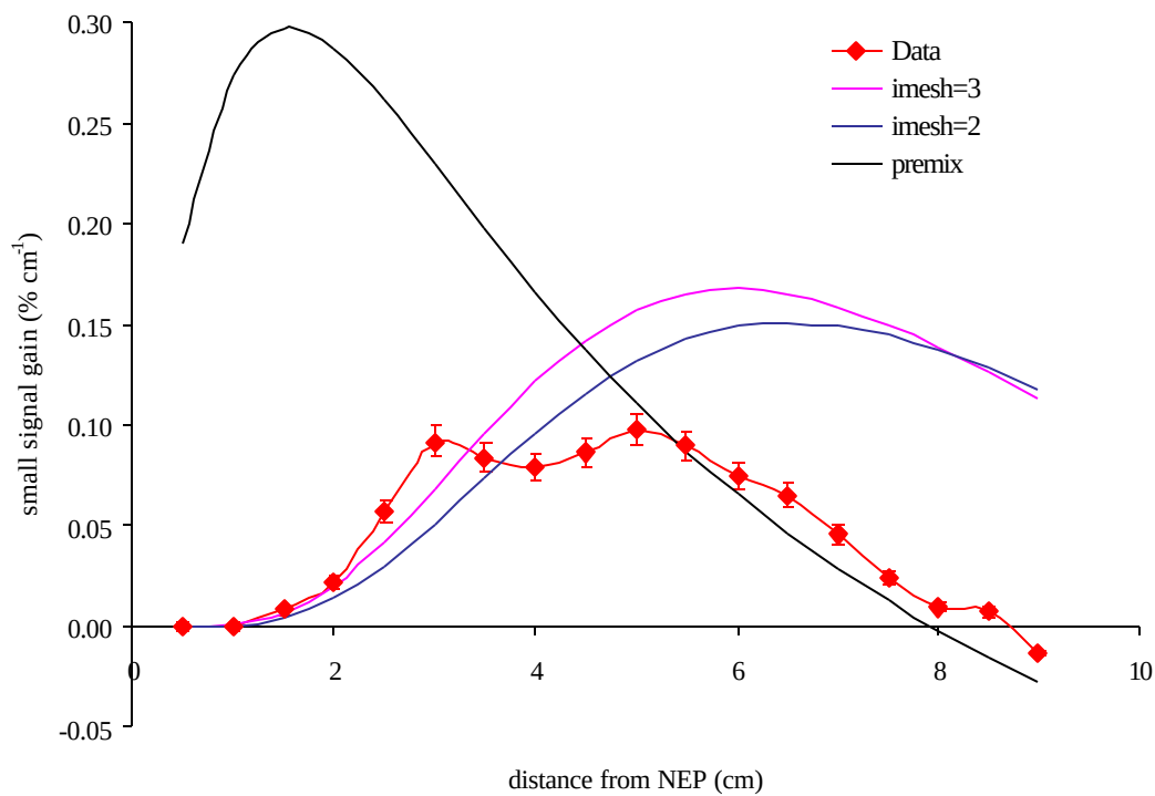
Figure 5.43 Measured and predicted centerline gain for the ( F_2=2 , H_2=10 ) flow conditions. Error bars represent 6% bias and 0.002 \text{ \% cm}^{-1} precision uncertainties.
