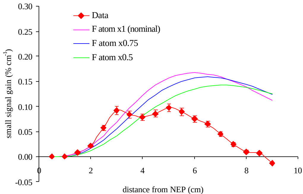
Figure 5.55 Measured and predicted centerline gain at different F atom flow rates for the ( F_2=2 , H_2=10 ) flow conditions. Error bars represent 6% bias and 0.002\text{ }\% \text{ cm}^{-1} precision uncertainties.
