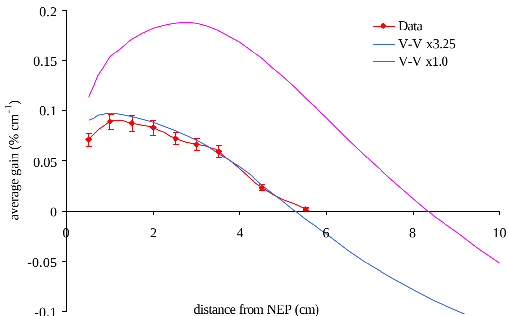
Figure 5.76 Measured and predicted average gain with without V-V rate constant adjustment for the ( F_2=2 , H_2=27 ) flow conditions. The gain is averaged over a region \pm 5 mm from the vertical centerline.
