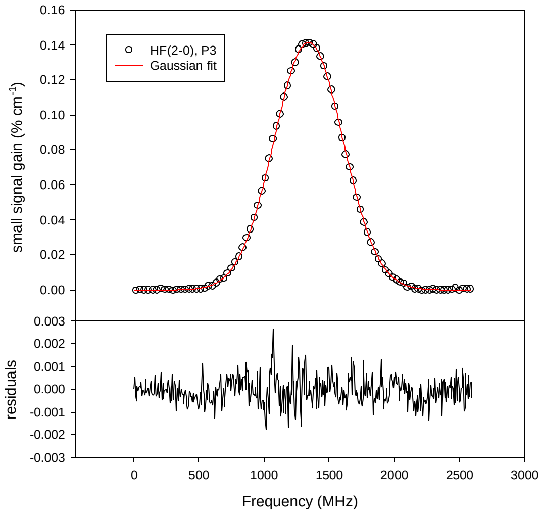
Figure 3.10 Transition lineshape of the P(3) ro-vibrational line of the first HF overtone ( v'=2 , J'=2 , v=0 , J=3 ). The experimental conditions for the upper panel are the ( F_2=2 , H_2=10 ) flow conditions, x = 2.5 cm downstream of the NEP, and z = 0.15 cm above the centerline. For purposes of clarity, only every 5 th data point is shown. The residual plot shown in the lower panel represents the residual difference between all the data and the curve fit and demonstrates that the Gaussian line function adequately fits the entire lineshape.
