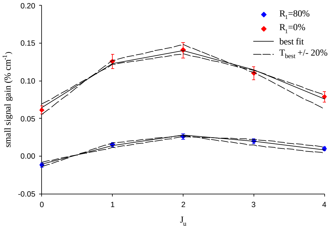
Figure 5.101 P1, P2, P3, P4 and P5 v=2-0 overtone gain distribution under small signal gain conditions ( R_1=0\% ) and saturated conditions ( R_1=80\% ). Data was taken 2.7 cm downstream of the NEP and 3.0 mm above the vertical centerline for the ( F_2=2 , H_2=10 ) flow conditions. The solid curves represent a least squares curve fit to a rotational equilibrium gain distribution with corresponding temperatures of 277 K and 164 K for R_1=0 and 80%, respectively. The dashed lines represent curve fits while holding the temperature fixed at \pm 20\% of the temperature determined from the least squares fit.
