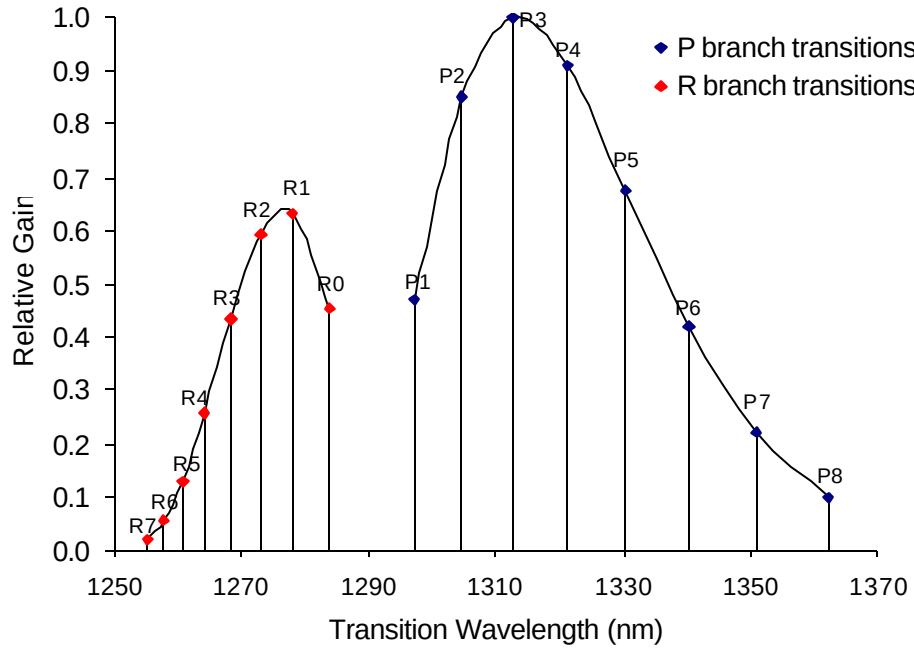
Figure 2.3 Relative gain distribution of HF v=2 to v=0 overtone transition at 300K.
