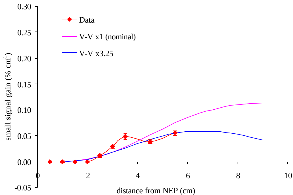
Figure 5.69 Measured and predicted centerline gain with V-V rate constant adjustment for the ( F_2=1 , H_2=5 ) flow conditions. Error bars represent 6% bias and 0.002\text{ }\% \text{ cm}^{-1} precision uncertainties.
