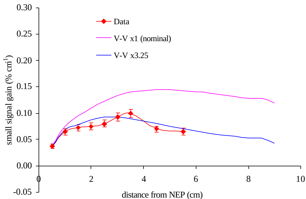
Figure 5.68 Measured and predicted peak gain with V-V rate constant adjustment for the ( F_2=1 , H_2=5 ) flow conditions. Error bars represent 6% bias and 0.002\text{ }\% \text{ cm}^{-1} precision uncertainties.
