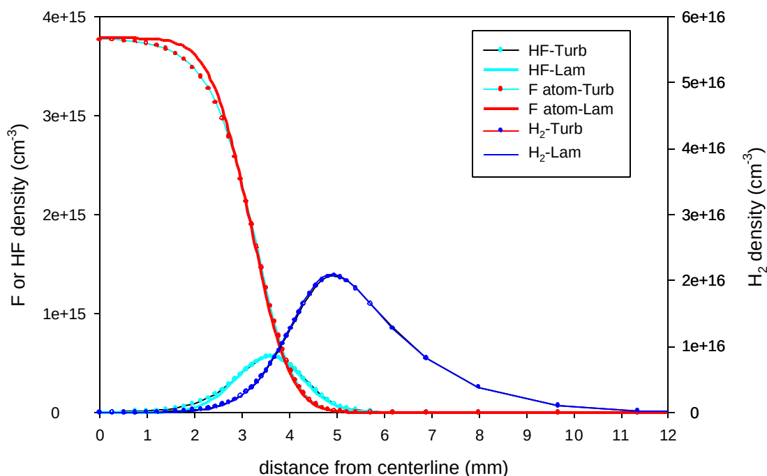
Figure 5.28 Predicted vertical concentration profiles 2.0 cm downstream of the NEP for the ( F_2=2 , H_2=10 ) flow conditions. Turbulent modeling case has 1% initial turbulence intensity.
