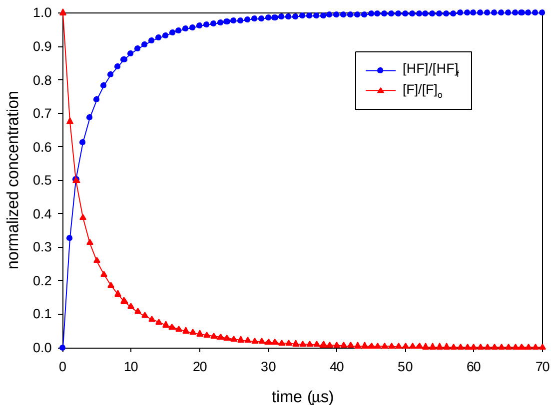
Figure 3.11 Normalized time response of [F] and [HF] for titration reaction F+HCl \rightleftharpoons HF+Cl for F_2 and HCl flow rates of 1 \text{ mmol s}^{-1} and 2.5 \text{ mmol s}^{-1} , respectively. Time for reaction to go to completion < 40 \mu\text{s} .
