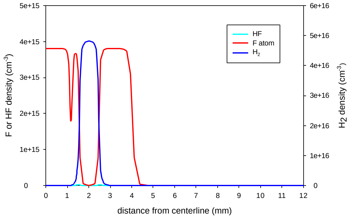
Figure 5.47 Predicted optimized injection scheme concentration profiles 0.025 cm downstream of NEP for ( F_2=2 , H_2=10 ) flow conditions.
