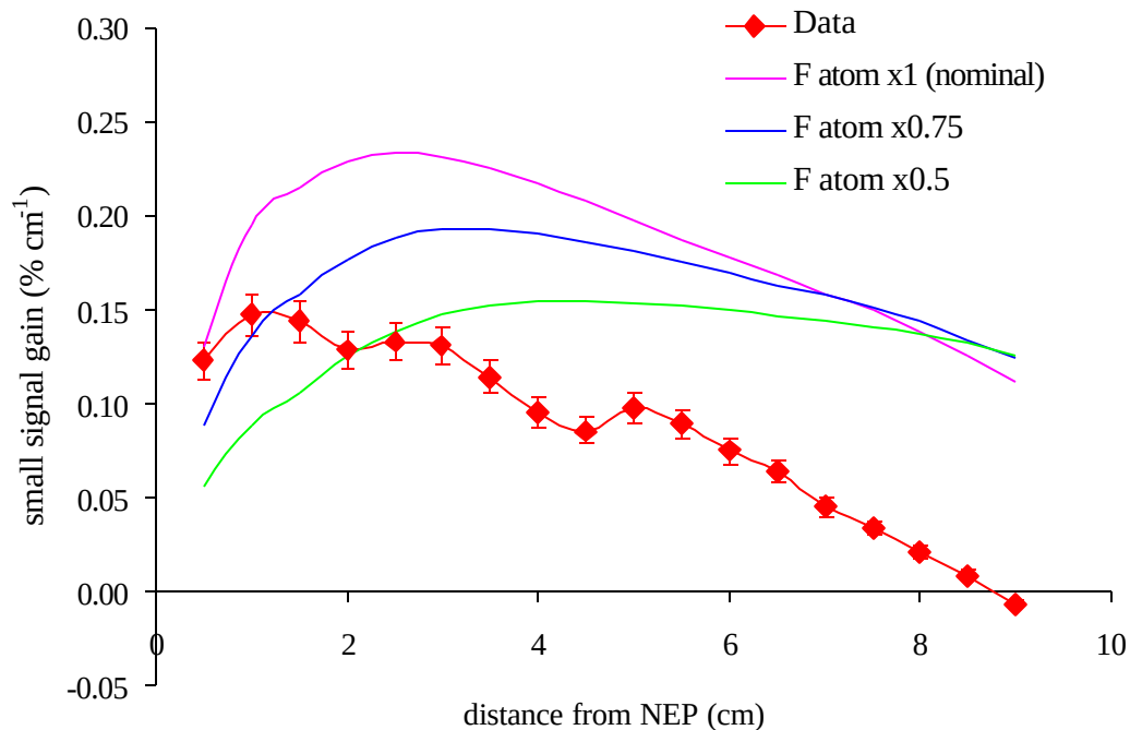
Figure 5.54 Measured and predicted peak gain at different F atom flow rates for the ( F_2=2 , H_2=10 ) flow conditions. Error bars represent 6% bias and 0.002\text{ }\% \text{ cm}^{-1} precision uncertainties.
