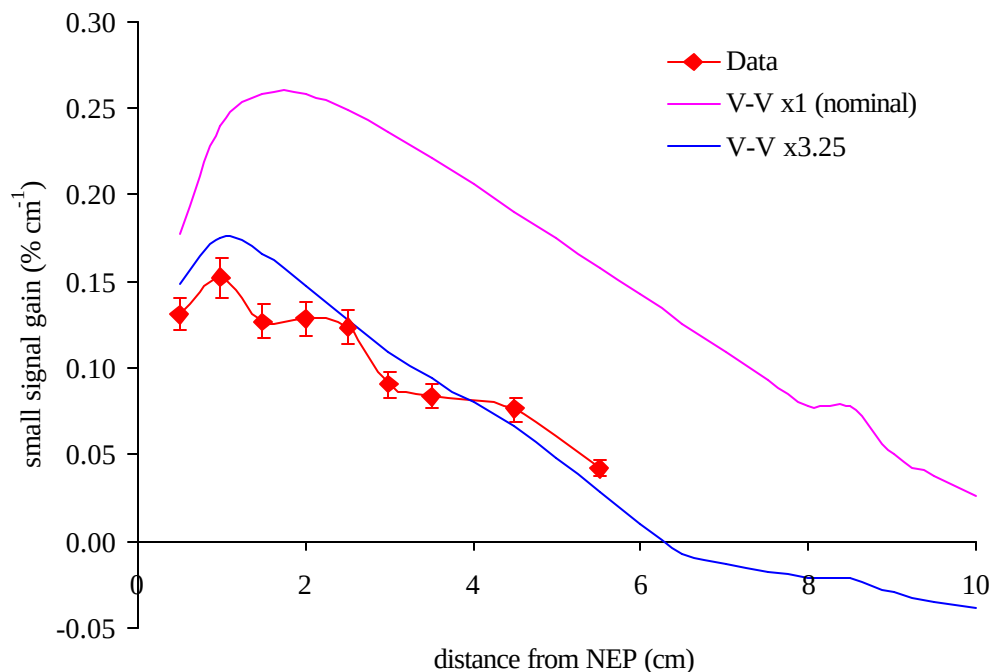
Figure 5.72 Measured and predicted peak gain with V-V rate constant adjustment for the ( F_2=3 , H_2=10 ) flow conditions. Error bars represent 6% bias and 0.002 \text{ } \% \text{ cm}^{-1} precision uncertainties.
