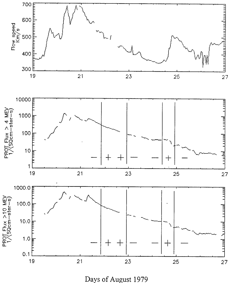
Fig. 16b. The same as Fig. 12 for Aug. 19, 1979 event under multiple change of magnetic field polarity.
