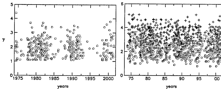
Fig.21b. Temporal variation of \gamma for integral(left panel) and differential (circles: 1-4.6 MeV, crosses: 4.6-25 MeV) channels (right panel)
