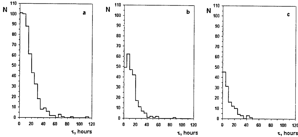
Fig. 3. Distribution of characteristic decay time, \tau , of proton >4 MeV fluxes
