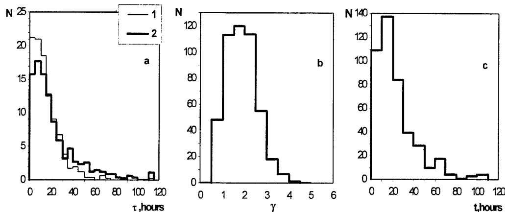
Fig.2a. Comparison of decay time distributions, \tau , of >4 MeV and >10 MeV protons.
