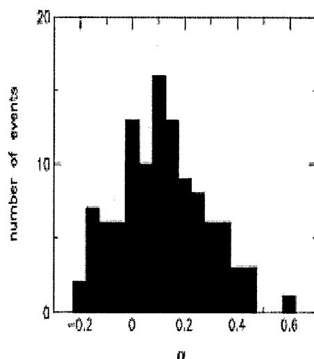
Fig.19 The distribution of the values of \alpha for 109 SEP events
