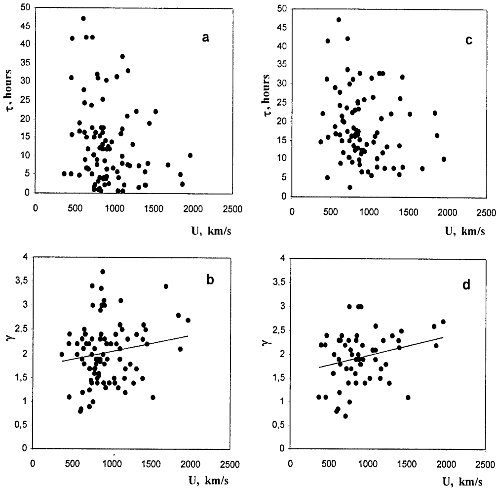
Fig.11. Dependence of characteristic decay time, \tau , and spectral index, \gamma , on the shock speed, U
