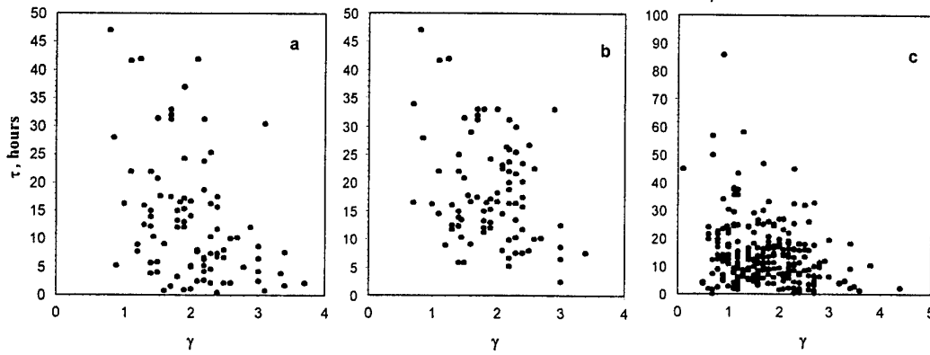
Fig.12. Correlation between proton >4 MeV decay time, \tau , and spectral index, \gamma a – for first criterion b – for second criterion c – without shock
