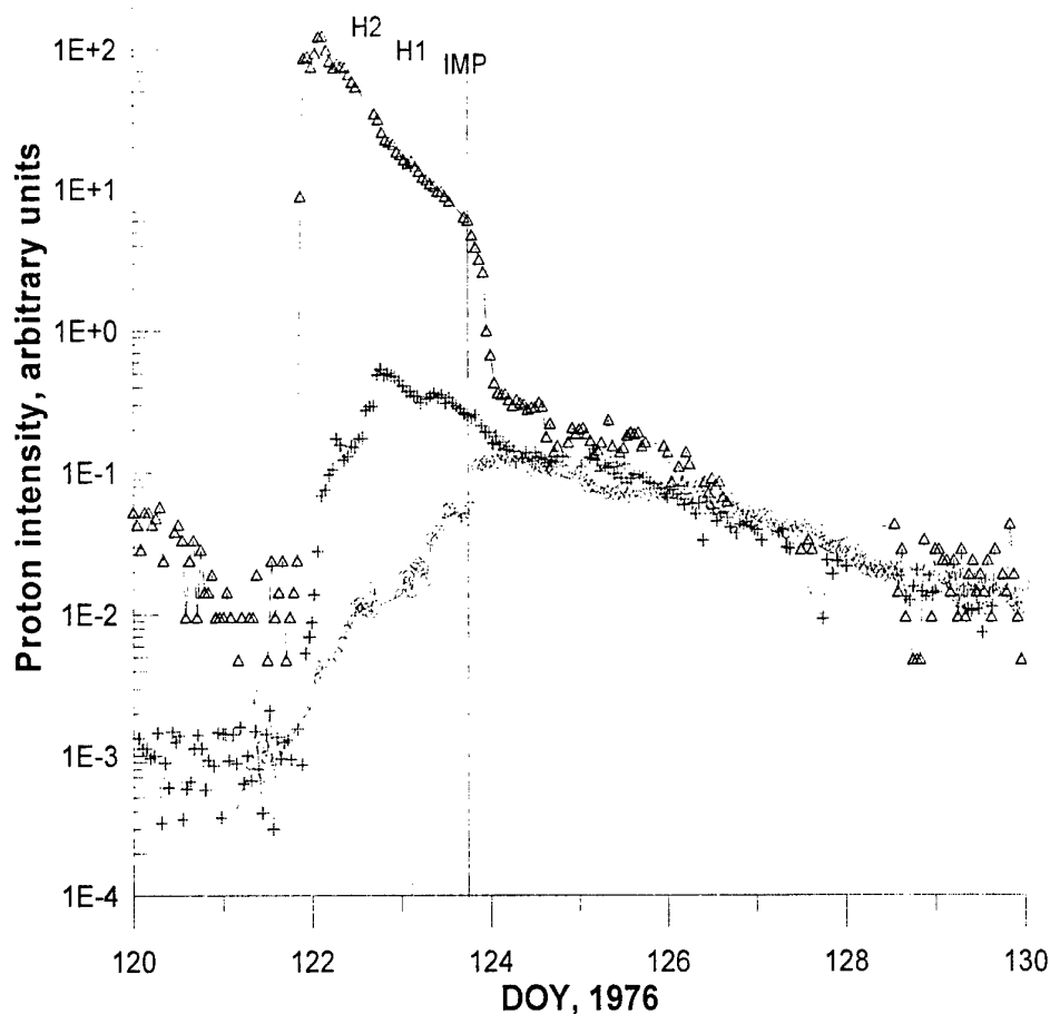
Figure 10. The fluxes of proton in SEP event 30 April 1976
