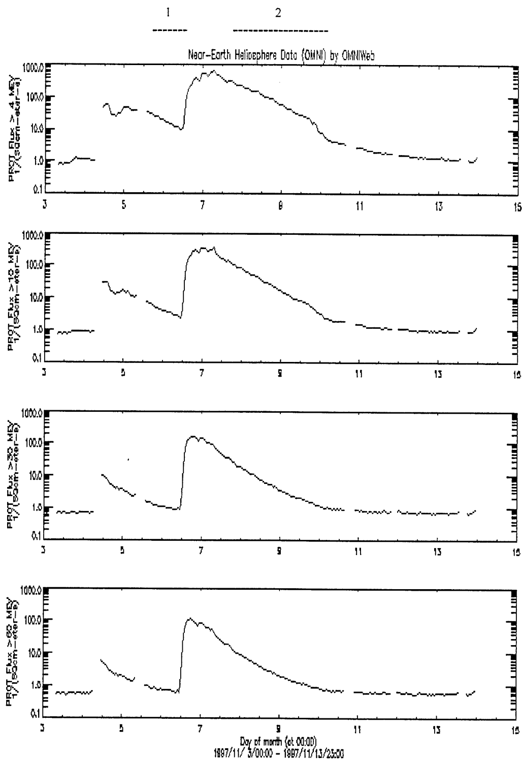
Fig. 1b. Pattern of proton flux time profiles for energies >4 , >10 , >30 and >60 MeV for sequence of events beginning from Nov.3, 1997. Dashed lines in the figure top shows selected intervals of the exponential decay presented in the Table 1A (Attachment).
