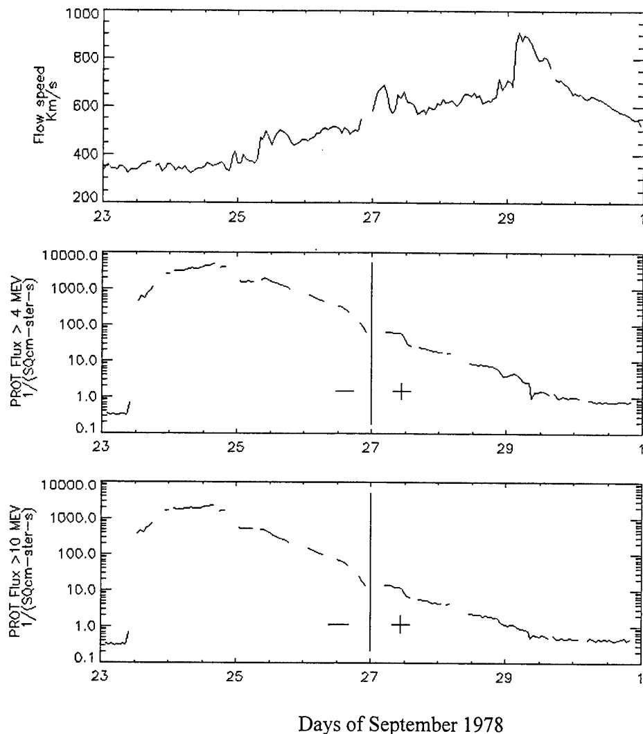
Fig.16a. The pattern of crossing the current sheet during Sept.23, 1978 event. Time-dependences of proton fluxes ( > 4 and > 10 MeV – two lower panels), as well as solar wind speed (upper panel).
