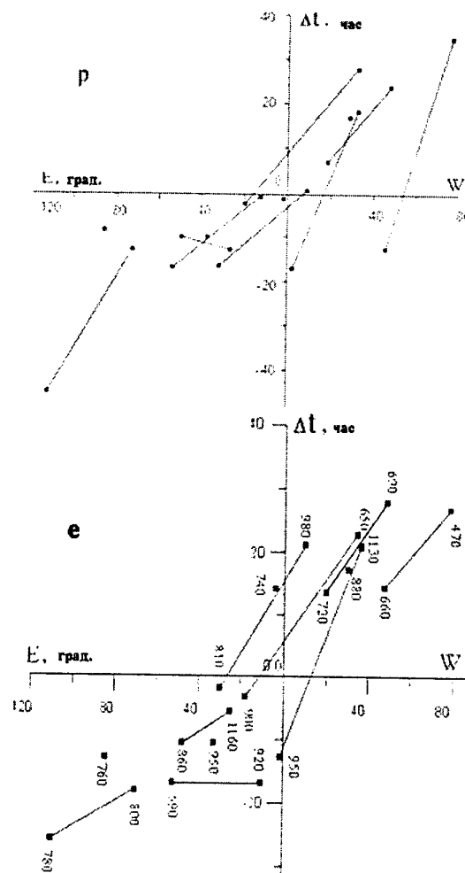
Fig. 9. Delay (negative) and advance (positive) time intervals, \Delta t , of invariance onset relative to the shock arrival versus corresponding heliographic distance, \Delta \lambda , between the s/c and a flare. Straight lines join the points corresponding to simultaneous measurement at Helios 1 and Helios 2 s/c. Figures near the points - transit shock speeds at the observation points
