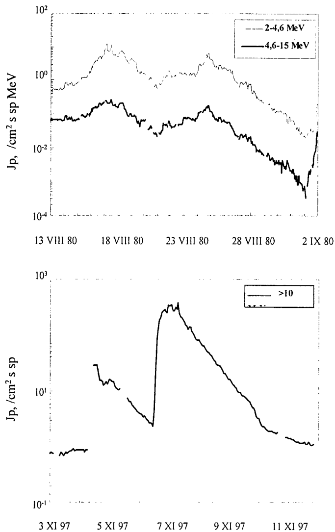
Fig.13. Two patterns of double SEP events (upper panel: the events of August, 15 and 25, 1980; lower panel: the events of November, 4 and 6, 1997) with identical decrease rates of different energy proton fluxes as observed at IMP 8. For the former case \tau equals 32 \pm 2 hrs, for the latter – \tau = 15-17 hrs.
