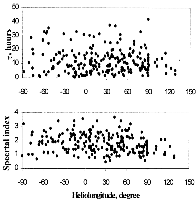
Fig.20. Scatter plots of decay times, \tau (upper) and spectral index, \gamma (lower) versus flare heliolongitude
