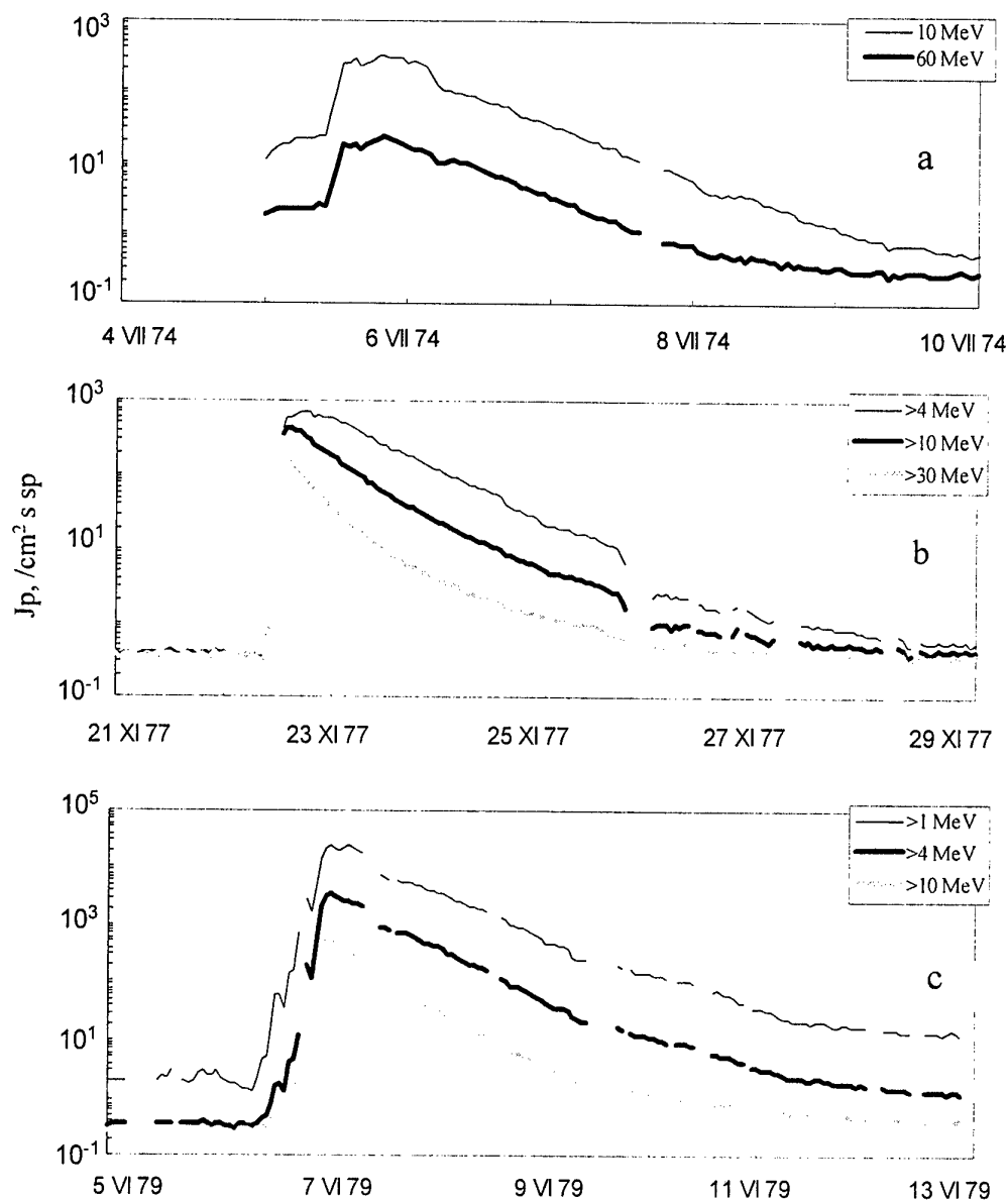
Fig.6. Patterns of different shapes of solar proton fluxes registered at the IMP 8 s/c after their peak values:
