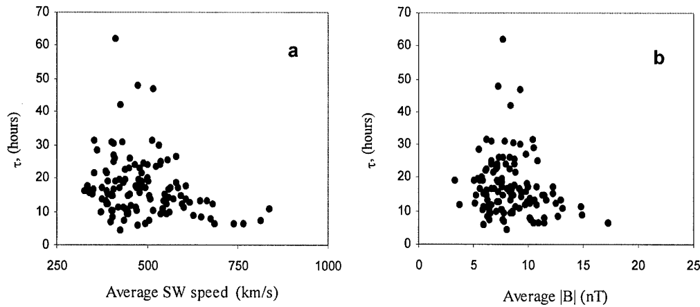
Fig.18. Dependence of the characteristic decay time on average through the event solar wind speed (a), average absolute value of magnetic field, |B| (b).
