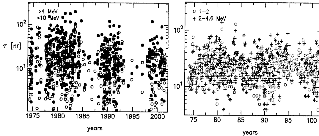
Fig.21a. Temporal variation of \tau for integral channels of protons (left panel) and differential (right panel)
