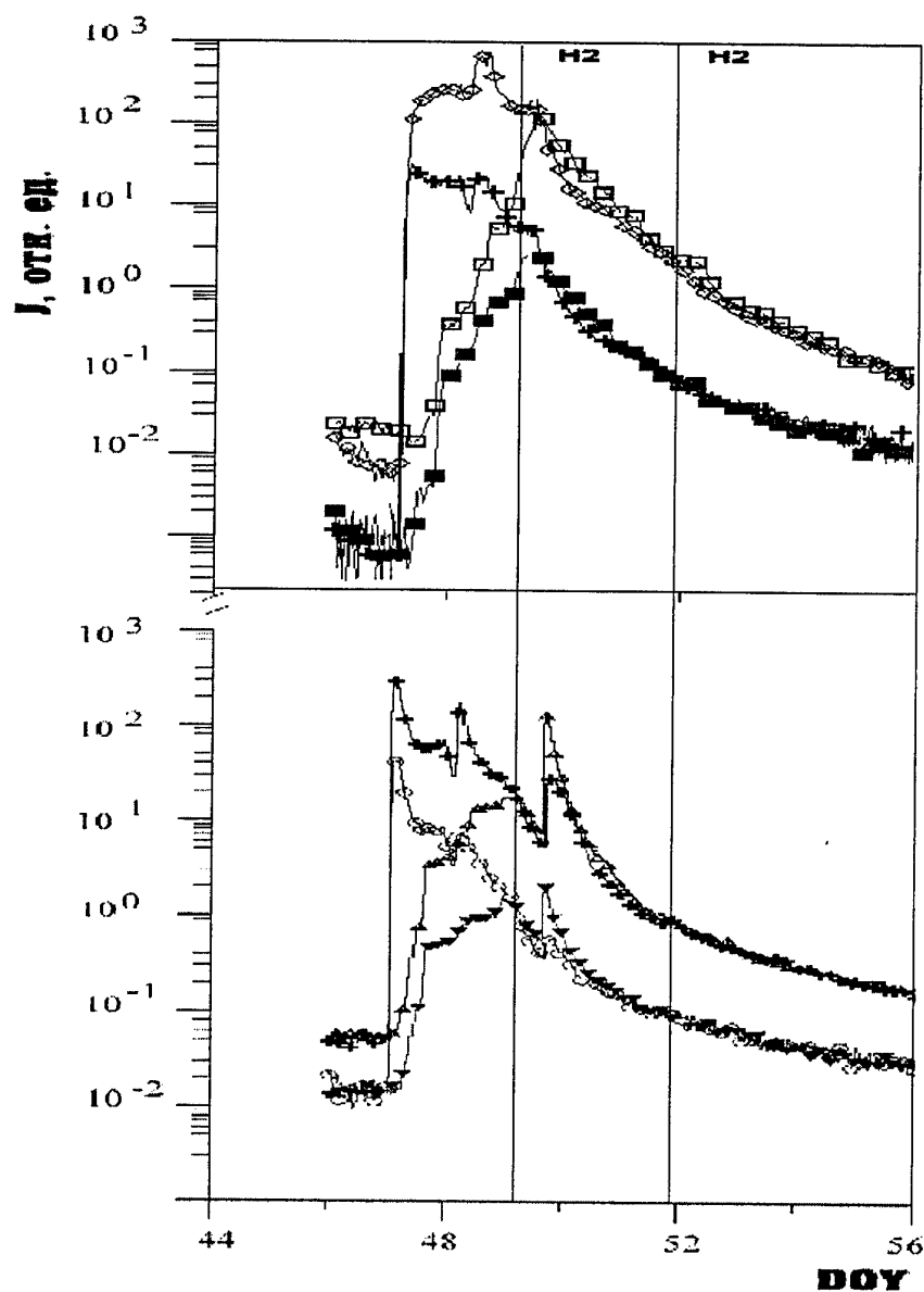
Fig. 8b. The same as fig.8a for Feb.16 (DOY 47), 1979 event
