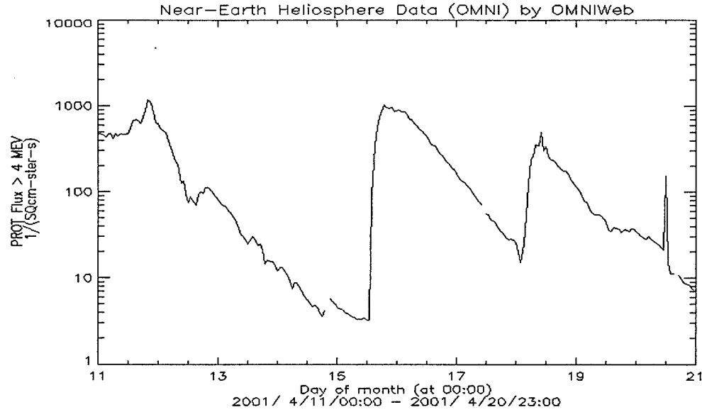
Fig. 14. Pattern of proton flux time profiles for energies >4 MeV for sequence of events beginning from Apr. 9, 2001.
