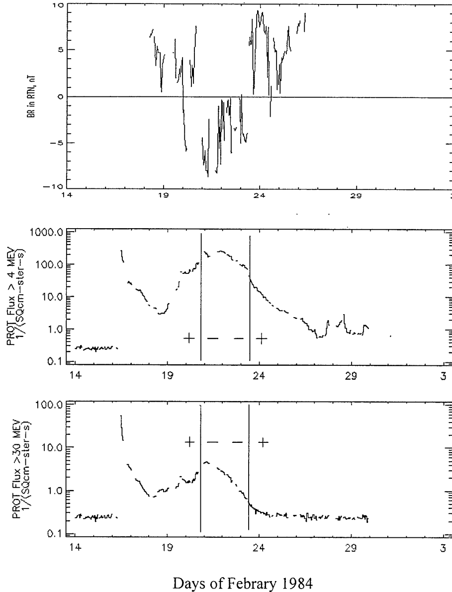
Fig.16c. The pattern of crossing the sector boundaries during two subsequent events in Feb. 1984, which shows no considerable influence on the fluxes of both low (>4 MeV) and high (>30 MeV) energy protons (middle and lower panels). Upper panel represents the direction of the radial component of the interplanetary magnetic field.
