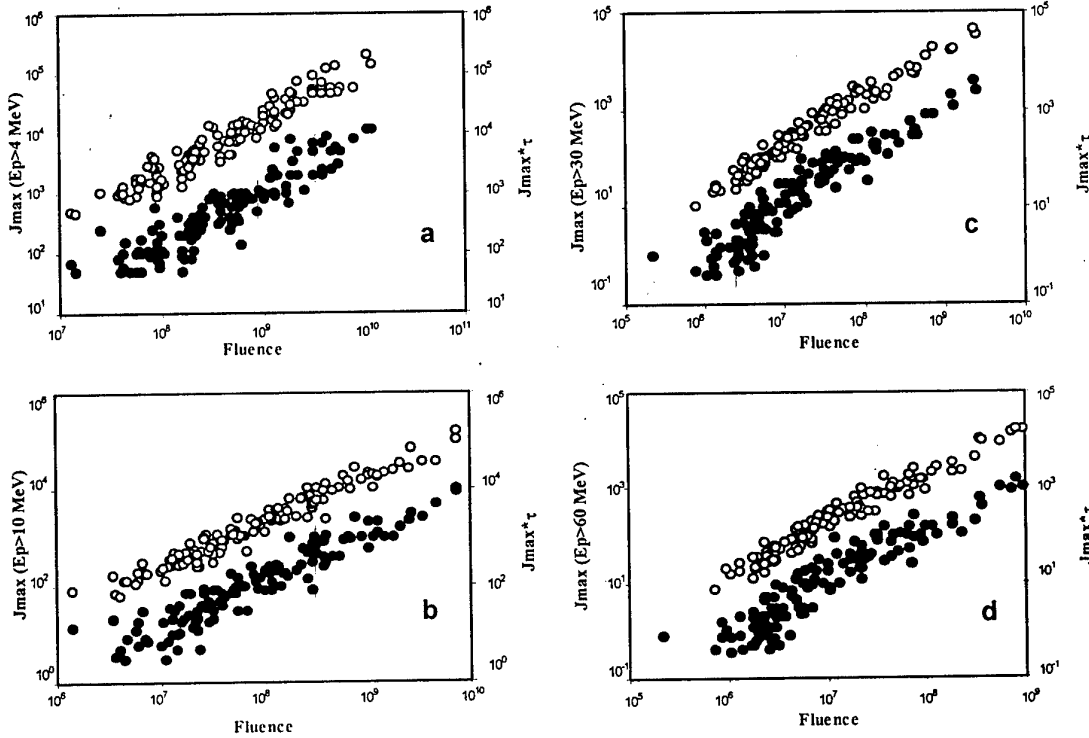
Fig.17. Dependence of proton a) for E_p > 4 MeV, b) E_p > 10 MeV, c) E_p > 30 MeV and d) E_p > 60 MeV fluence through the event on the peak intensity J_{\max}(\bullet) and J_{\max} \cdot \tau (o) and on the product of peak intensity and characteristic decay time
