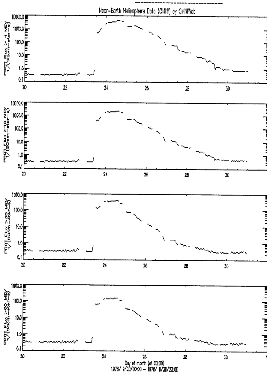
Fig. 1a. Pattern of proton flux time profiles for energies >4 , >10 , >30 and >60 MeV beginning from Sept. 20, 1978. Dashed line in the figure top shows selected interval of the exponential decay presented in the Table 1A (Attachment).
