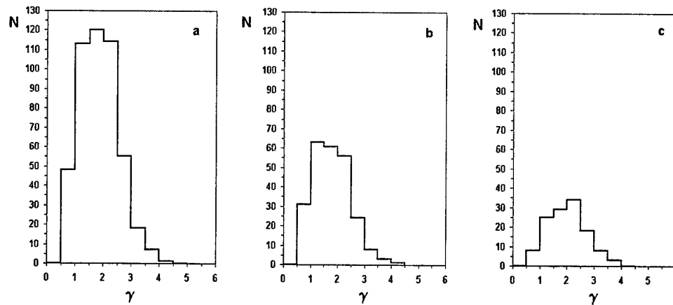
Fig.4. Distribution of proton integral energy spectrum exponents, \gamma , in the energy range 4-60 MeV. The value of exponent, \gamma , relates to the beginnings of exponential decline periods
