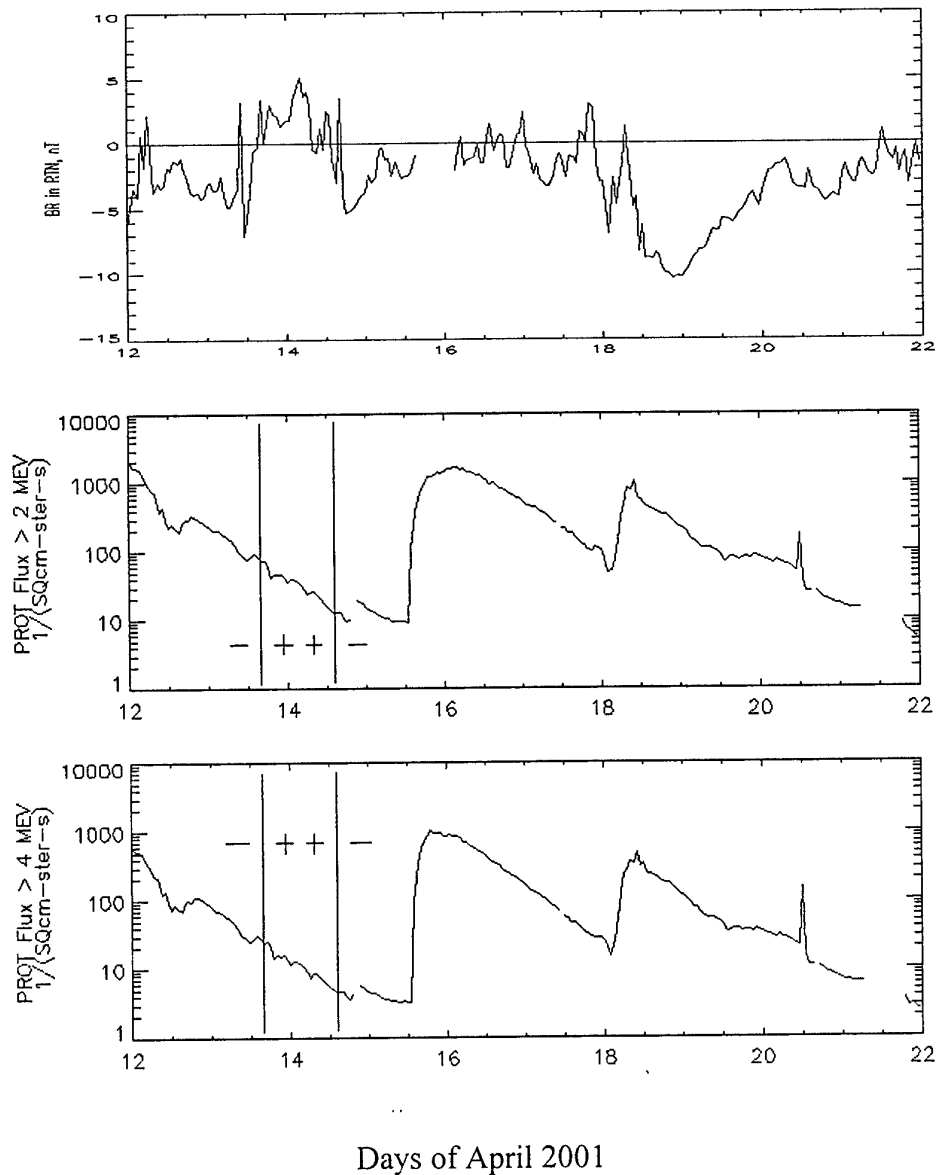
Fig. 16d. The same as Fig.14 for E_p > 2 MeV and E_p > 4 MeV proton fluxes for the sequence of events during April 2001.
