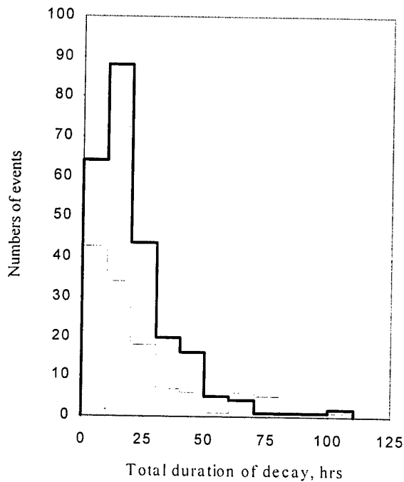
Fig.5. Distributions of total durations of decays - accompanied by shock (thin line) - non-accompanied by shock (solid)
