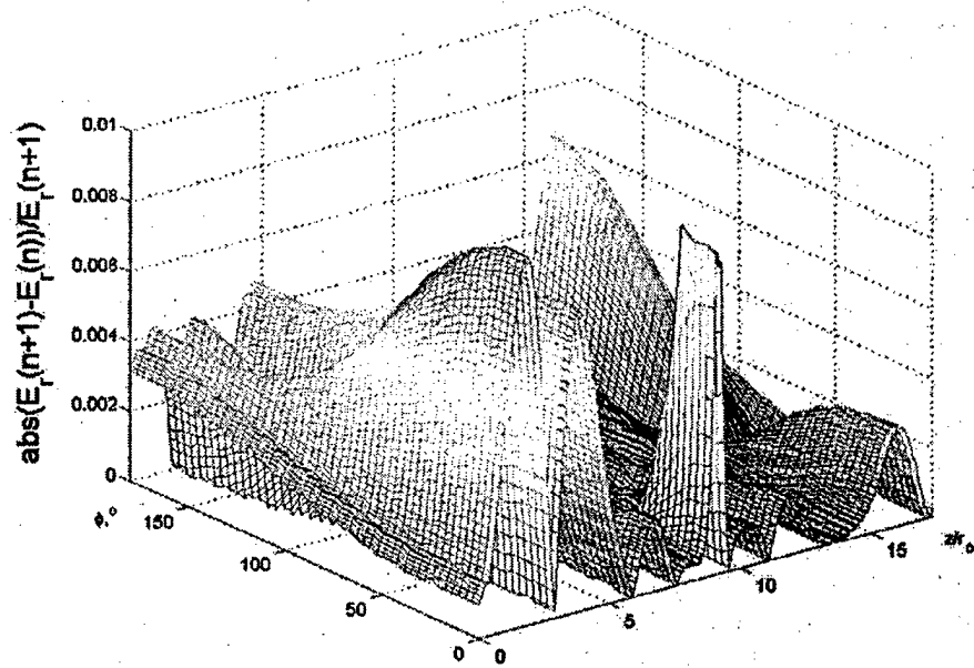
Figure 20. Relative absolute difference between the amplitudes of E_r computed at third and at second periods of the calculation in the \phi z plane closest to the inner conductor of the coaxial line. Calculation parameters: f=5 GHz, r_i=3 mm, r_o=6.9 mm. Parameters of obstacle: h=3 mm, \phi_0=28.2^\circ , l=1.5 mm, \rho=30 \Omega cm obstacle is placed on the inner conductor of the coaxial line.
