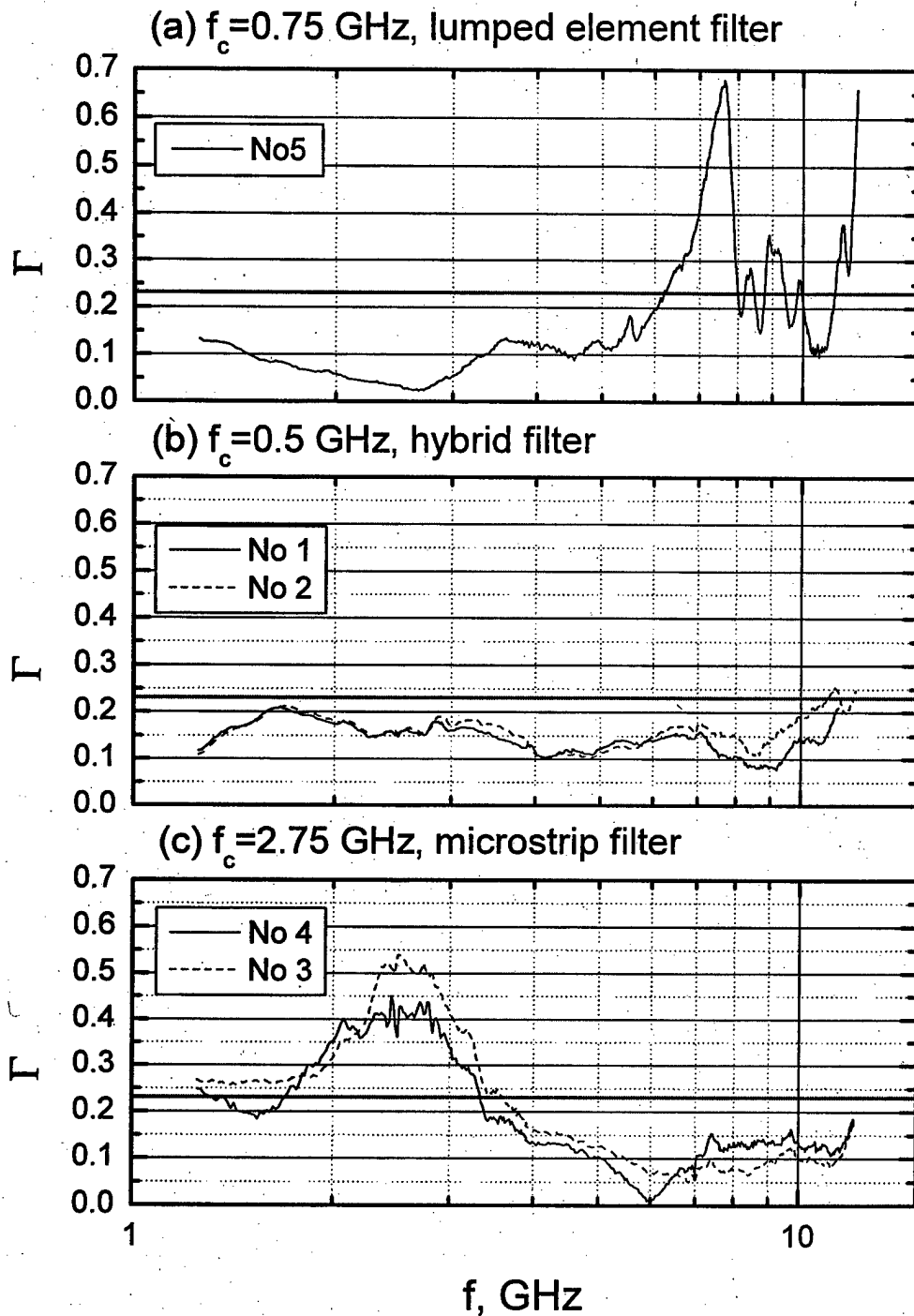
Figure 10. Measured dependencies of reflection coefficient for the CRS with different realizations of 5 elements Butterworth filter: (a) lumped element filter f_c=0.75 GHz, (b) lumped element filter with additional ferrite line as a part of the first inductance of the filter f_c=0.5 GHz, (c) distributed element filter made of the segments of different impedance microstrip line. Solid line in the figure denotes the highest limit of the reflection coefficient allowed by desirable technical specification presented in the Appendix.
