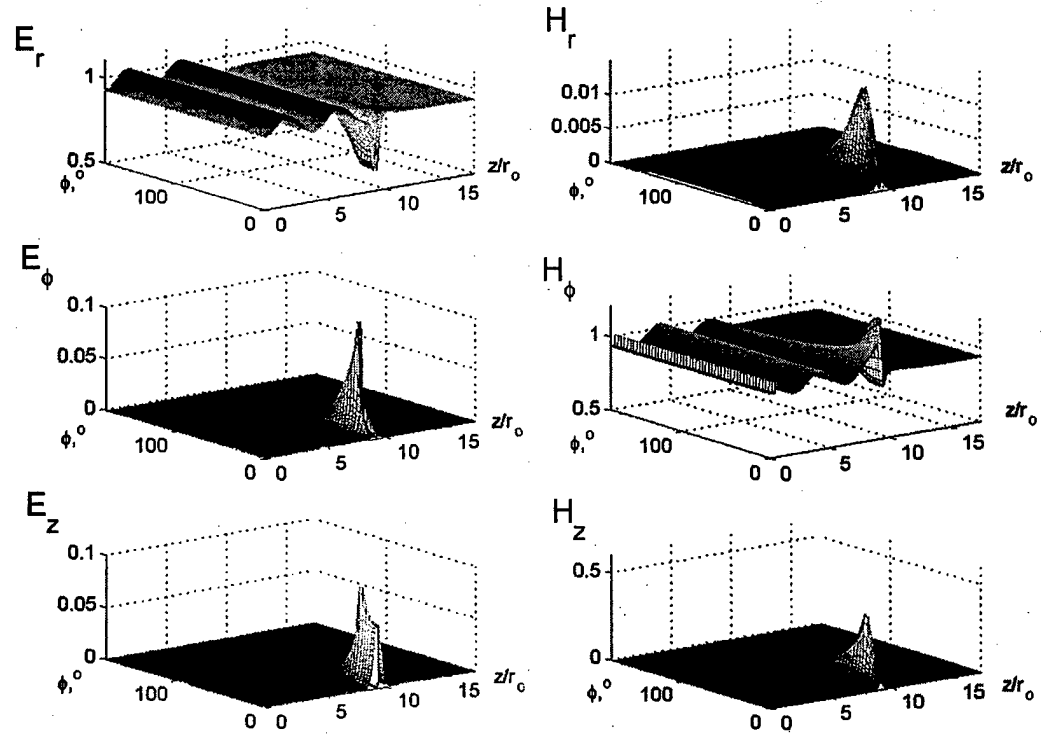
Figure 21. The distribution of the amplitudes of electric and magnetic field components in the \phi z plane closest to the inner conductor of the coaxial line. Calculation parameters and the size of the obstacle are the same as in Figure 20 .
