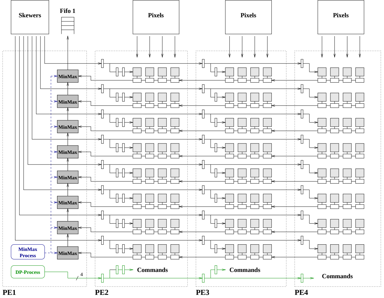
Figure 5: Wildforce Implementation
