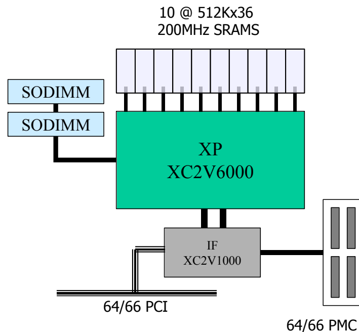
Figure 2-10 Osiris Architecture
