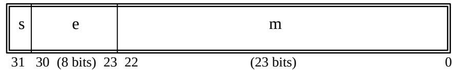
Figure 6 Floating Point Format (32 bits)
