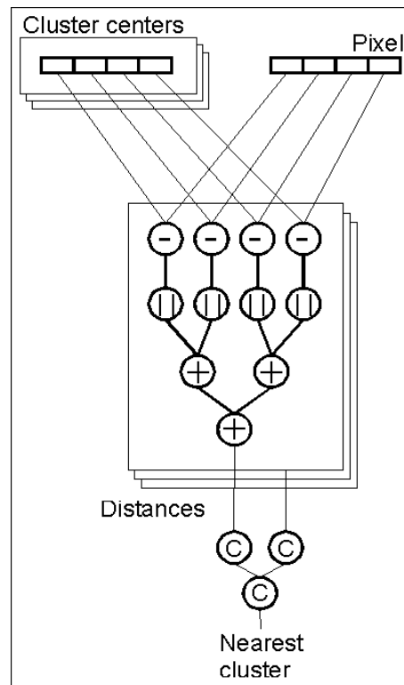
Figure 2. Datapath
