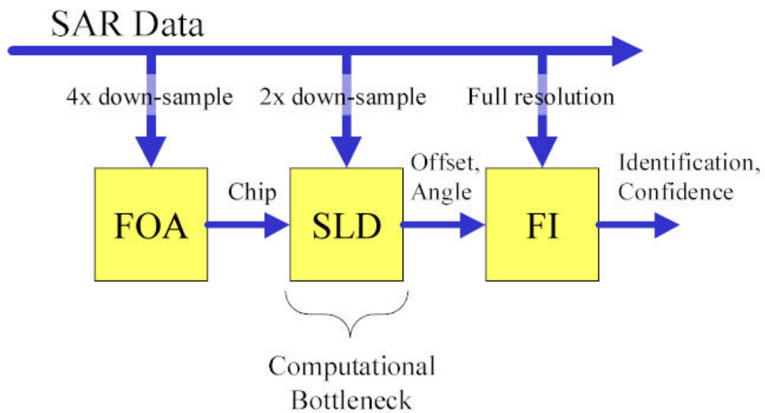
Figure 7. SAR/ATR Algorithm Flow
