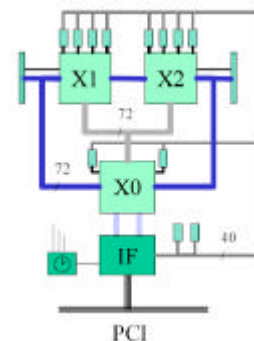
Figure 4. SLAAC Architecture
