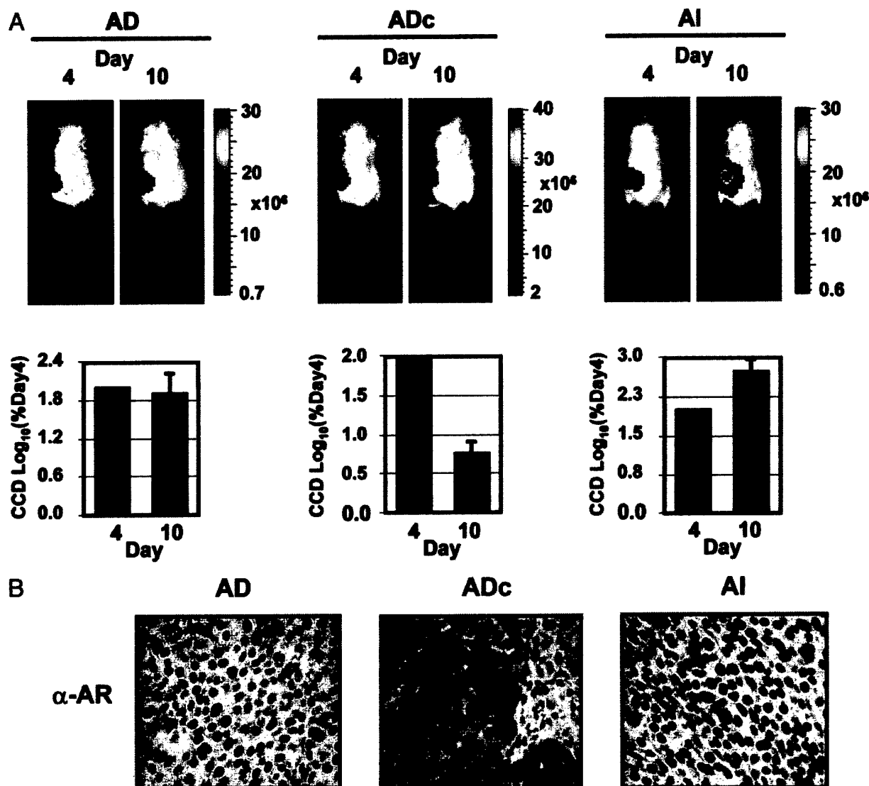
Fig. 3. Imaging AR signaling in LAPC9 tumors. In A, SCID mice implanted with LAPC9 xenografts ( >0.5 cm) were injected with 10^7 pfu of AdTSTA and the mice were imaged every 3–4 days until day 14. Representative mice at day 4 and day 10 after virus injection from the AD group, the castrated (on day 4) AD group (ADc), and the stable AI group. The bar graph summarizes a cohort of three or more and summarizes the log of the percentage change in signal from day 4 (blue bars) to day 10 (purple bars). Day 4 is set at 2 (log 10) in each case. The normalization to percentage change was necessary because there is variation in virus infectivity in different tumors. B shows representative immunohistochemical localization of AR in the AD, ADc, and AI tumors using anti-AR antibodies. AR stains brown against the blue-stained nuclei. For both AD and AI tumors, five high-power fields ( \times 40 ) from multiple sample slides were counted, with an average of 100 cells/field. AR nuclear staining was recorded as percentage of cells counted. For AD tumors, cells with high AR nuclear staining are 33% ( \pm 5\% ), whereas cells with no or very faint AR nuclear staining is 19% ( \pm 6\% ) with the remainder staining at an intermediate intensity. For AI tumors, 30% ( \pm 2.7\% ) of the cells stained intensely, whereas cells with no or very faint AR nuclear staining was 22% ( \pm 3\% ). In conclusion, AR nuclear staining does not differ significantly between AD and AI tumors ( P = 0.3 one tail and 0.7 two tail); bars, \pm SE.
