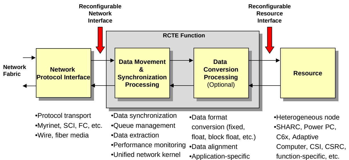
Figure 42. ReConfigurable Transport Engine Concept
