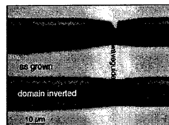
Fig. 2: Periodically poled \text{LiNbO}_3 waveguide device imaged in a confocal luminescence microscope
