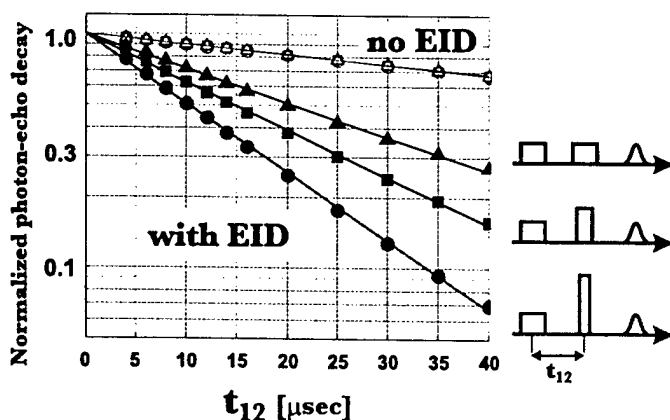
Fig. 1 Simulated photon-echo decay with and without the excitation-induced decay feature turned on (Lorentzian of width \sigma_0=10^{-3} ). Pulse areas are kept constant while the duration of the second pulse is decreased, increasing excitation bandwidth and thus the effects of EID. Lines show exponential fits.
