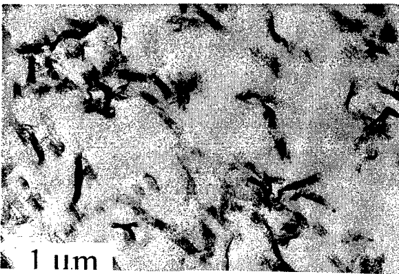
Figure 12. TEM micrographs of composite morphology. a) NC11 no styrene, low power; large aggregates are scattered throughout the sample, and only a few individual (exfoliated) silicate plates are observed; compare Figure 11a b) NC11, styrene, high power; small aggregates are well dispersed, and the exfoliated fraction is higher; compare Figure 11c c) RC11, styrene, high power; compare Figure 11f. Images (b) and (c) are similar, because aggregates of intercalated and as-treated clay are similar. The average aggregate size is slightly smaller in (c), and the degree of exfoliation is greater. Most exfoliated silicate particles are not observed edge on, so they appear as ribbons in these thin sections.
