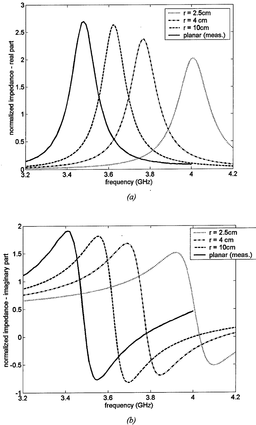
Figure 4.9. Input impedance of a \phi -polarized quasi-rectangular patch printed on a spherical structure for different sphere radii; (a) real part, (b) imaginary part.
