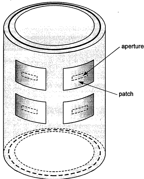
Figure 6.21 – The circular-cylindrical 2x2 aperture-coupled patch array
