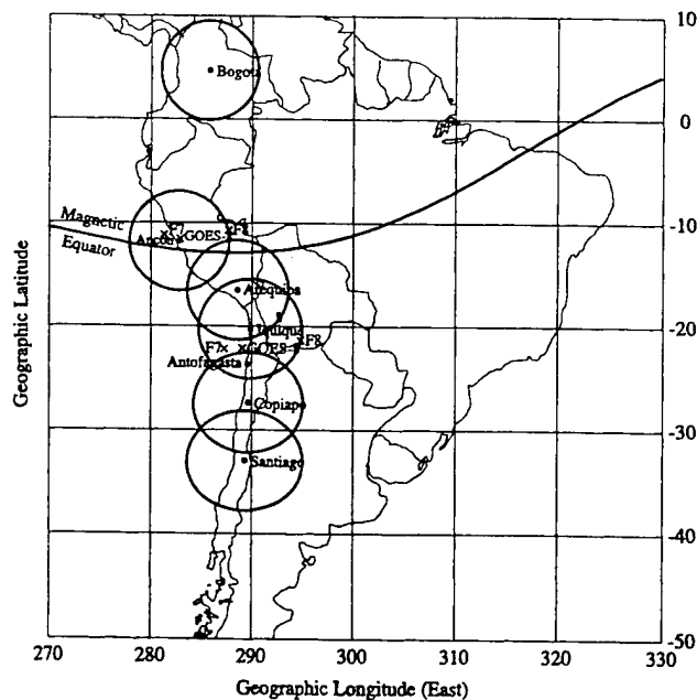
Figure 7. Equatorial array of GPS stations on the west coast of South America providing latitude variation of TEC data. The circles around the stations indicate 30^\circ elevation coverage. Also shown are 350-km ionosphere intersection points to Fleetsat 7 (F7), Fleetsat 8 (F8), and GOES 8 from Ancon, Peru, and Antofagasta, Chile.
