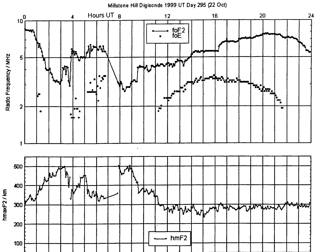
Figure 11. Digisonde data showing the F layer critical frequency f_oF_2 , the E layer critical frequency f_oE , and the maximum height of the F layer h_mF_2 observed at Westford, Massachusetts, on October 22, 1999. Note that the appearance of f_oE between 0400 and 0700 UT (2300–0200 LT) implies the presence of auroral particle precipitation. The break in the data from 0700 to 0800 UT is caused by increased absorption.
