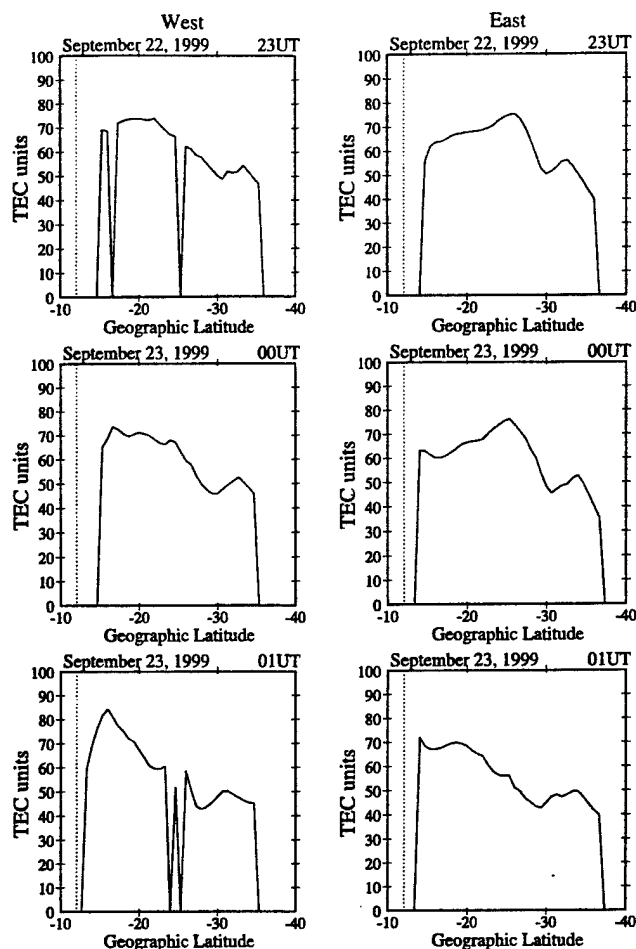
Figure 9. The latitude variation of TEC using the southern half (in magnetic latitudes) of the array computed to the west and east of longitude 72^{\circ}\text{W} . While the data from the eastern half show a clear formation of the equatorial anomaly at 2300 UT (1800 LT) on September 22 and 0000 UT (1900 LT) on September 23 at 25^{\circ}\text{S} ( 15^{\circ} magnetic latitude), the western half does not show any evidence for anomaly development with the TEC peak being close to the magnetic equator. The abrupt discontinuities in the plots are the result of data dropouts.
