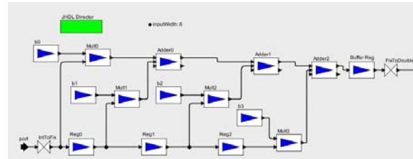
(b) Ptolemy Model Using JHDL Primitives
