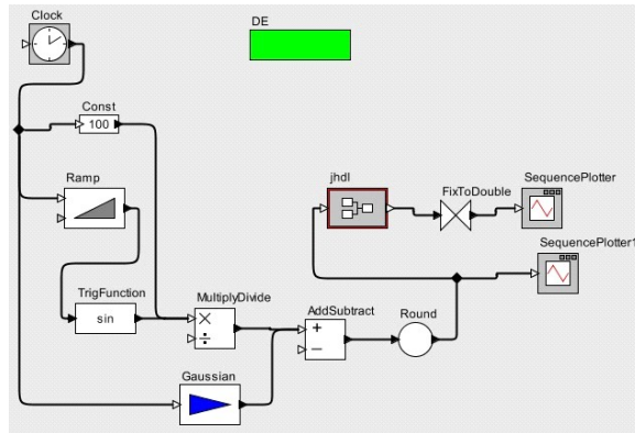
(a) Top-level Ptolemy Testbench Model
