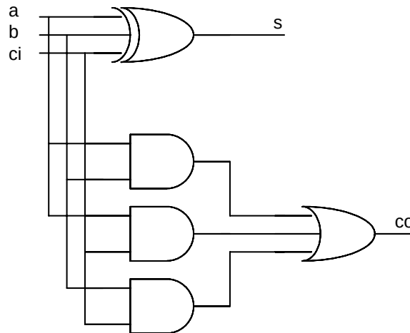
Figure 3: Full-Adder Example Circuit
