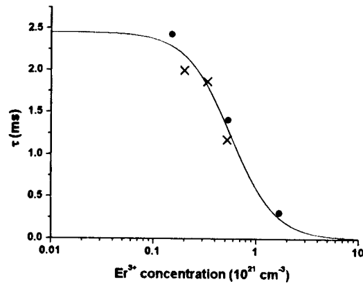
Figure 4: Self-quenching of {}^4I_{13/2} and the limited diffusion hypothesis. Continuous curve is simulation by Eq. [9] with parameters: \tau_0=2.45 ms; N_0=0.67 \cdot 10^{21} \text{ cm}^{-3} ; points marked as X, are for samples prepared with an increased N content.
