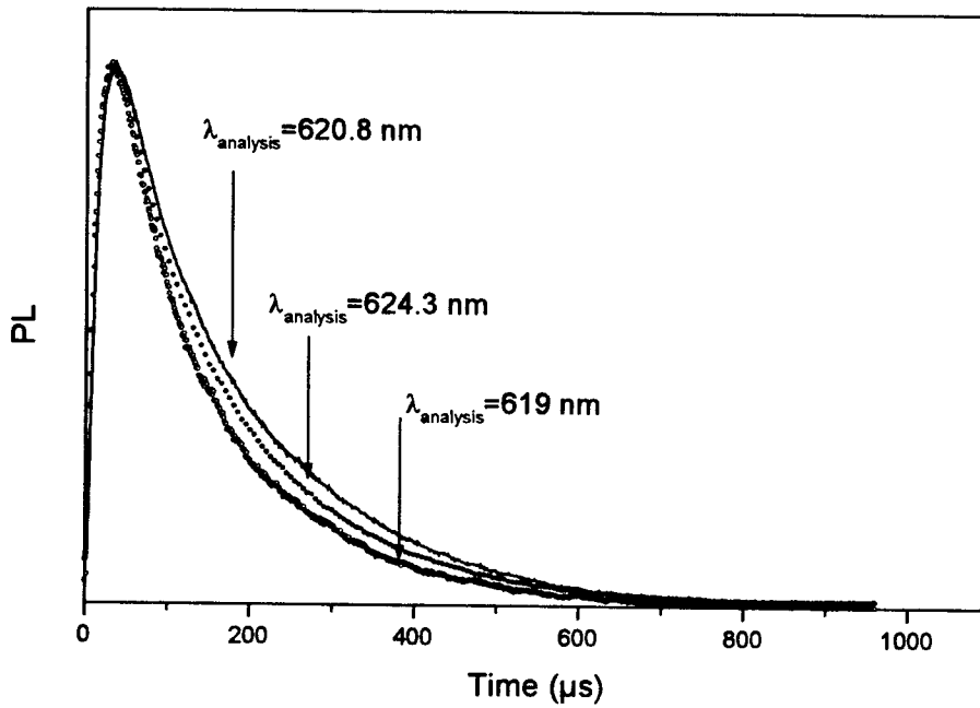
Figure 3: {}^5D_0 decay profiles measured at several wavelengths for the \text{Eu}^{3+}:\text{GaN} sample D035 excited at \lambda_{\text{exc}}=355 \text{ nm} , T=300 \text{ K}
