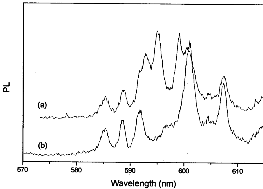
Figure 7: Time resolved luminescence spectra of \text{Eu}^{3+}:\text{GaN} ( T=300\text{ K} , \lambda_{\text{exc}}=355\text{ nm} ) a- spectrum recorded 5\ \mu\text{s} after the excitation pulse b- spectrum recorded 100\ \mu\text{s} after the excitation pulse
