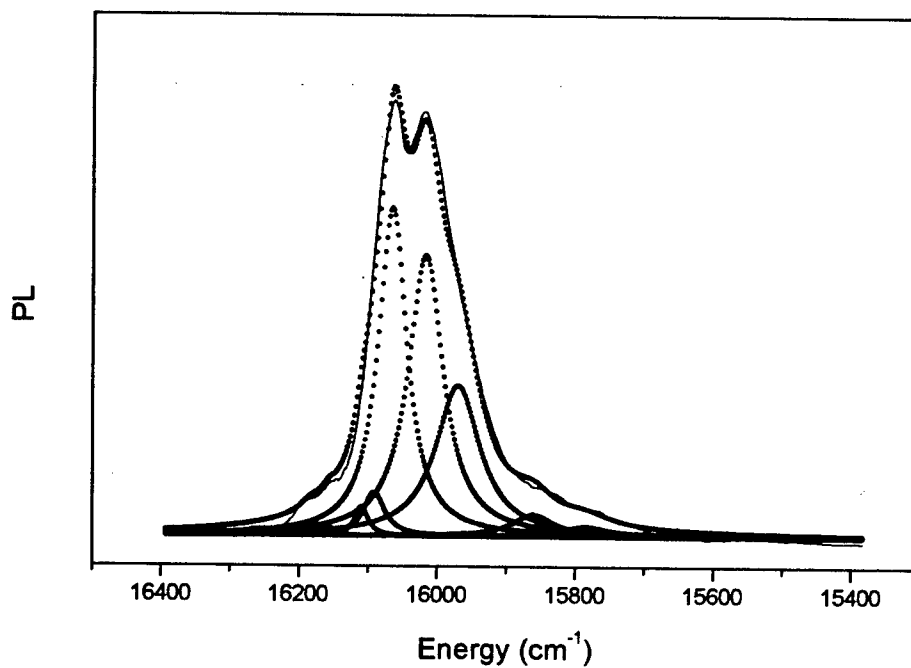
Figure 9b: Deconvolution of the {}^5D_0 \rightarrow {}^7F_2 transition for the \text{Eu}^{3+}:\text{GaN} sample D035 excited at 355 nm at room temperature (dotted lines : calculated curves)
