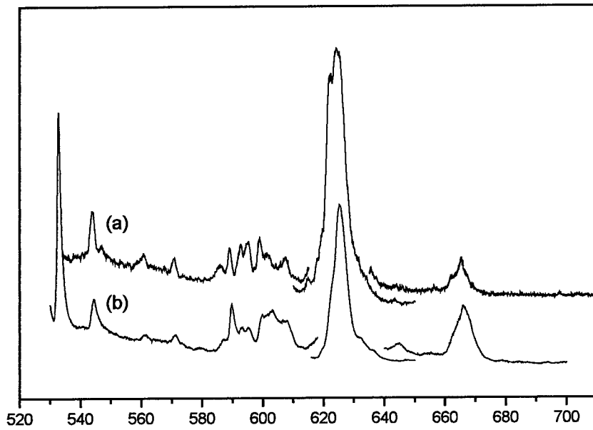
Figure 4: Luminescence spectrum recorded for the \text{Eu}^{3+} :GaN sample D035 under excitation above the energy band gap (a- T=300 K, b- T=10 K)
