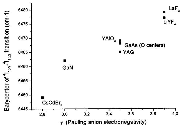
Figure 2: The {}^4I_{13/2} - {}^4I_{15/2} transition barycenters for selected Er^{3+} doped hosts.
