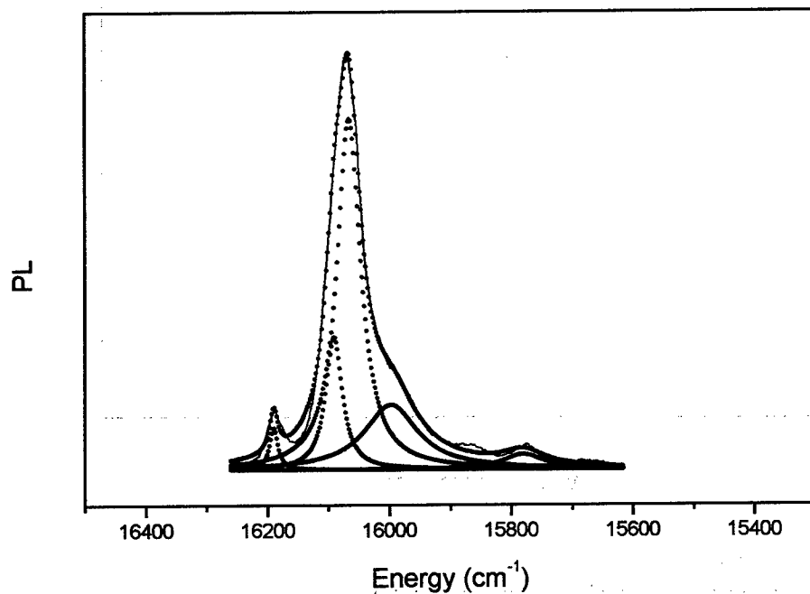
Figure 9a: Deconvolution of the {}^5D_0 \rightarrow {}^7F_2 transition for the \text{Eu}^{3+}:\text{GaN} sample D120 excited at 355 nm at room temperature (dotted lines: calculated curves)
