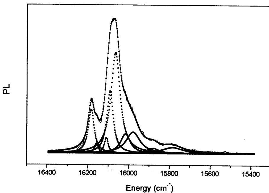
Figure 9c: Deconvolution of the {}^5D_0 \rightarrow {}^7F_2 transition for the \text{Eu}^{3+}:\text{GaN} sample RJ_081 excited at 355 nm at room temperature (dotted lines : calculated curves)
