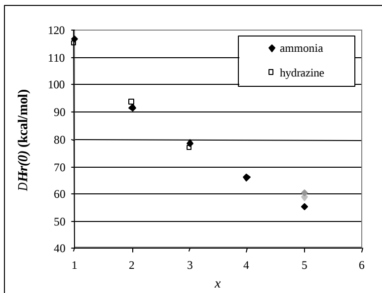
Figure 4. DH_r(0) for B_x + \text{HNO}_3 \rightarrow (\text{BH}^+)B_{x-1} + \text{NO}_3^- , where B is ammonia or hydrazine.
