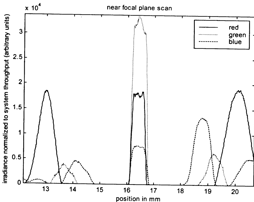
Figure 11. Profile of normalized irradiance distribution near the focal plane for (a) the entire field of view and (b) for the region containing the -1, 0, and +1 diffraction orders. The data was taken using DCSFI.
