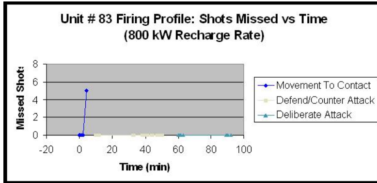
Figure II-13. EM gun shots missed for Unit 83 (800 kW power)
