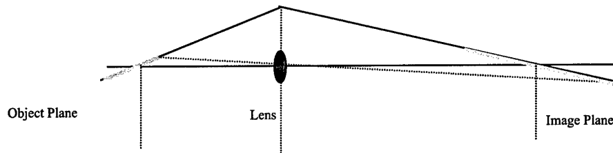
Figure 3 The Scheimpflug Condition
