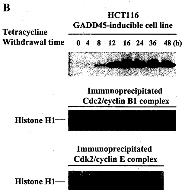
Figure 4 Subcellular localization of cyclin B1 protein and inhibition of Gadd45. (a) Cellular proteins were prepared from HCT116 GADD45 -inducible cells after withdrawal of tetracycline at the indicated time points. 100 \mu g of proteins were loaded onto SDS-PAGE gel for phosphorylation of subcellular distribution of cyclin B1 protein and phosphorylations of CHK1 or Cdc25C. (b) One mg of cellular proteins isolated from HCT116 GADD45 -inducible cells at the indicated time points was immunoprecipitated with anti-cyclin B1 or cyclin E antibodies, and histone H1 kinase assays were performed as described in Materials and methods. Labeled histone H1 was detected by autoradiography following size separation on a SDS-PAGE gel
