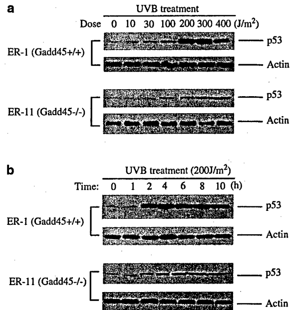
Figure 1 Attenuated induction of p53 protein in Gadd45a -/- cells treated with UVB. (a) Both E1A/ras-transformed normal MEFs (ER-1) and Gadd45a -/- MEFs (ER-11) were treated with UVB at different doses (range from 0 to 400 J/m 2 ). Cells were harvested at 8 h post-treatment and cellular proteins were prepared as described previously. Total cell protein (100 µg) was loaded onto 10% SDS-PAGE gels. Following electrophoresis, the proteins were transferred to Immobilon membranes. The membranes were then blocked for 30 min in 5% milk at room temperature. Measurement of p53 protein was performed with anti-mouse p53 antibody (Santa Cruz Biotech, CA, USA). Immunoreaction was revealed using chemiluminescence detection procedure. As a loading control, detection of actin protein was included. Only visualized bands are shown; their estimated sizes were 53 kDa for p53 protein and 43 kDa for actin. All the experiments were performed at least three times. The results of the representative experiment are shown in this figure. (b) ER-1 and ER11 cells were exposed to UVB at a dose of 200 J/m 2 and harvested at the different time points. Detection of p53 expression was performed as described in (a)
