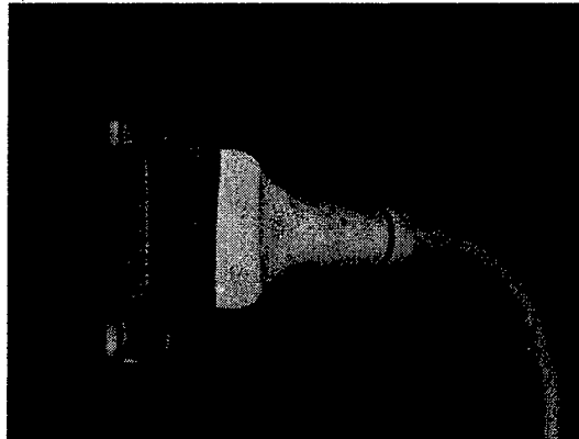
FIG. 7 Photograph of a transducer with the compressor plate mounted.
