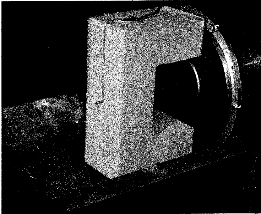
Fig. 4 Experimental set-up.
