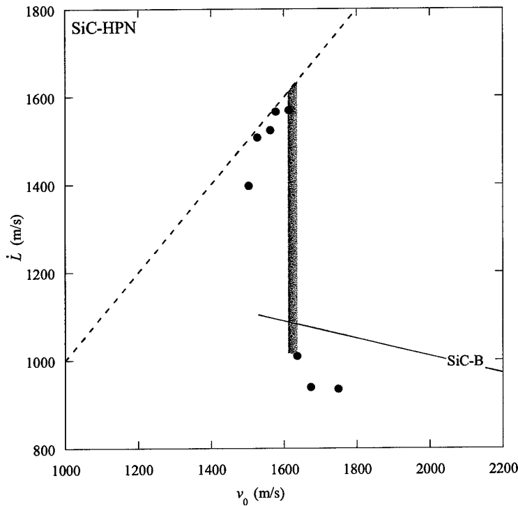
Fig. 20 Projectile erosion velocity \dot{L} versus impact velocity v_0 for the tests with SiC-HPN. Shaded area indicates region within which transition occurs. The solid line corresponds to the SiC-B data fit in Fig. 17. Dashed line represents \dot{L} = v_0 .
