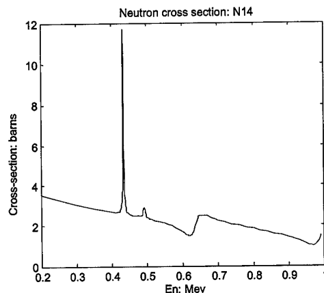
Figure 4. Nitrogen cross-section in the low energy region
