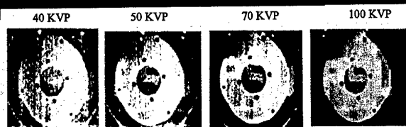
Fig. 3. Backscatter radiographs of the composite test object shown in Fig. 4 made at (a) 40 KVP, (b) 50 KVP, (c) 70 KVP, and (d) 100 KVP beam energy. These radiographs show how near surface features can appear progressively more transparent at higher X-ray energies.
