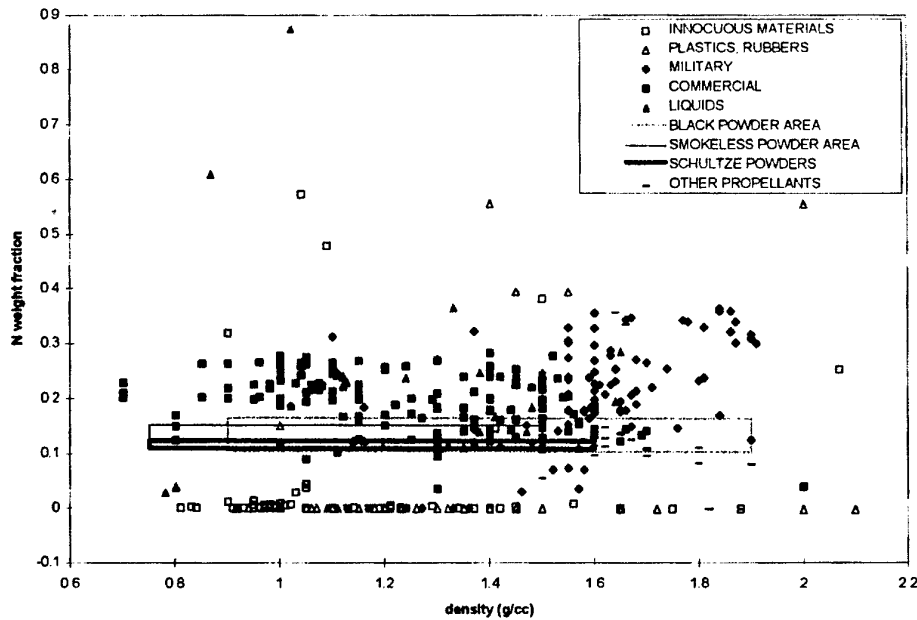
Figure 2 Relationship between density and nitrogen fraction for various materials. Although nitrogen content is generally high for explosives, there still is a significant overlap with ordinary materials [2]
