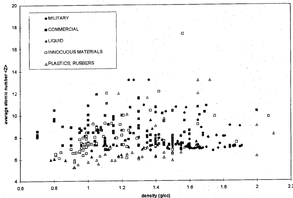
Figure 1 Relationship between average atomic number and density for selected materials. Note the concentration of relatively high density and average atomic number between 7 and 8 for military explosives [2].
