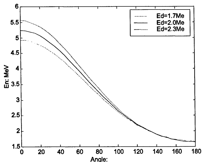
Figure 9. Energy of neutron resulting from the DD reaction at 1.7 to 2.3 MeV incident energy deuteron.
