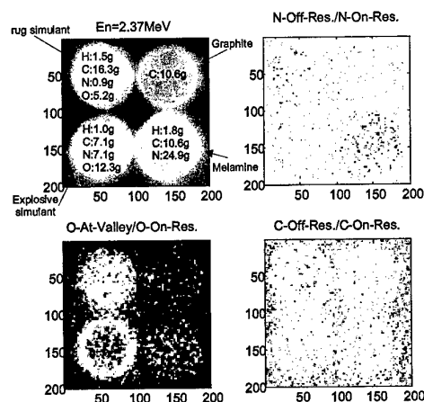
Figure 8. NRR with single peaks (a) image at 2.37 MeV, (b) nitrogen on and off resonance, (c) oxygen on and off resonance, (d) carbon on and off resonance.
