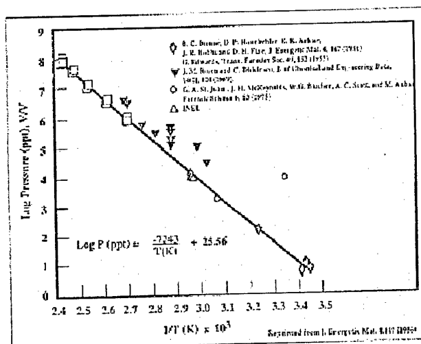
Figure 2 Change of vapour pressure of PETN with temperature
