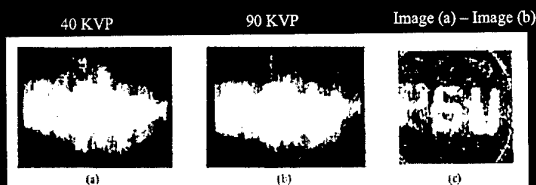
Fig. 9. Demonstration of X-ray backscatter tomography by subtraction of two images made at different energies. (a) is a backscatter image of the test object made at 40 KVP, (b) an image made at 90 KVP, and (c) shows the tomographic image plane containing the PSU letters generated by subtracting (a) and (b).
