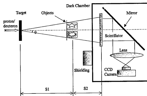
Figure 7. Scintillation camera used for imaging experiments
