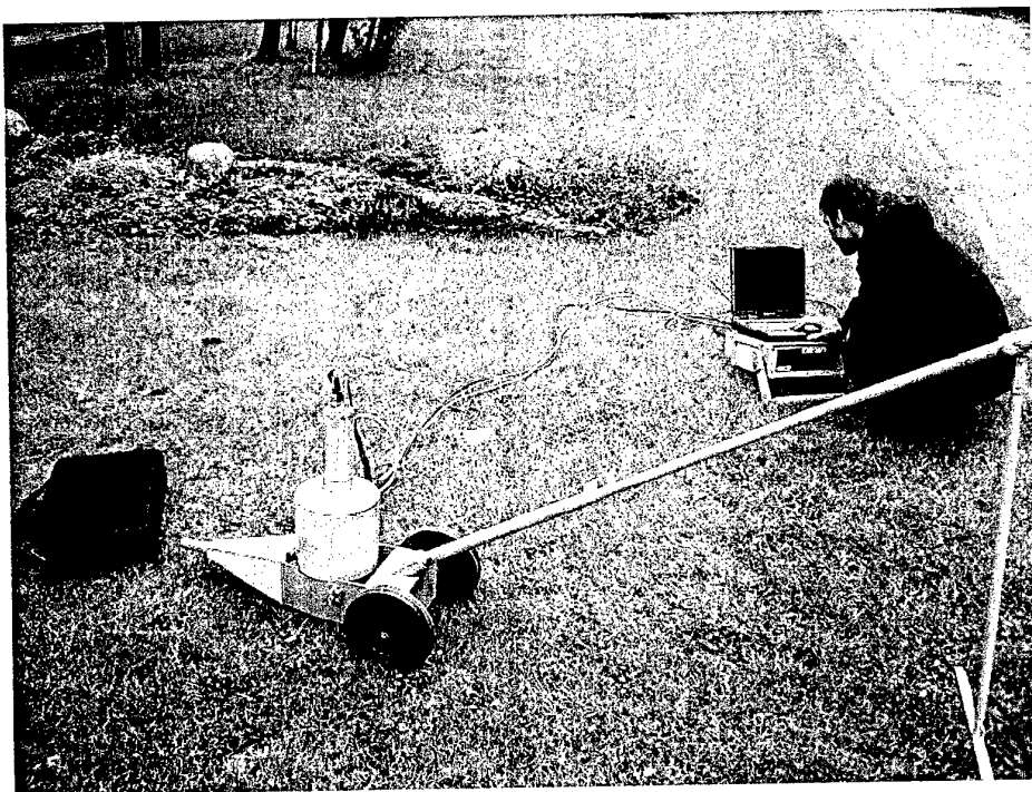
Figure 2. Existing prototype of the mobile device for detection of explosive substances during the field test at Radium Institute.
