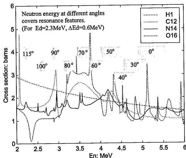
Figure 10. Spectrum of energies scanned. The shaded areas are the range of energies at a particular nominal neutron angle.
