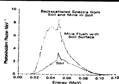
Fig. 5. Calculated photon spectra produced by backscatter of a 160-kVp X-ray beam (spectrum shown in Fig. 2) perpendicularly incident on soil and on soil containing a 30-cm-diam mine buried flush with the soil surface. One million photon histories are followed for each spectrum.
