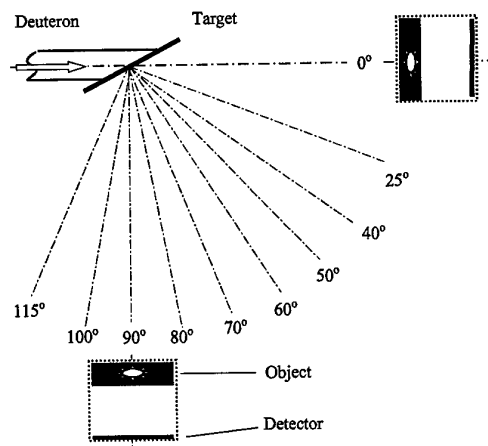
Figure 11. One possible approach to scanning baggage. The baggage is moved in a circular path centered on the deuterium target.
