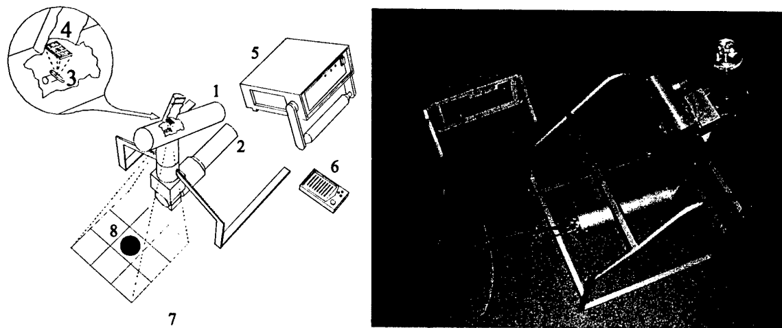
Figure 3. Left: portable device for detection of explosive substances. 1 - neutron generator with built-in sectioned detector of accompanying \alpha -particles, 2 - \gamma -ray detector, 3 - target, 4 - segmented detector of the accompanying particles, 5 - specialized block of electronics, 6 - pocket computer (control panel), 7 - the inspected area, 8 - hidden object. Right: view of the existing prototype.
