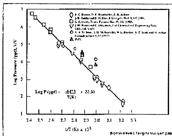
Figure 1 Change of vapour pressure of RDX with temperature
