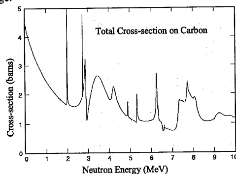
Figure 5. Resonance structure for carbon in the 0.5 to 10 MeV range
