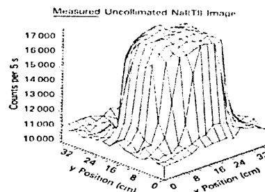
Fig. 4. Three-dimensional image of the measured uncollimated NaI(Tl) pulse mode detector response to a 100-kVp source beam filtered by 0.24 mm of lead for a 30-cm-diam mine buried flush with the soil surface. The response is sampled at a 2.54-cm increment.
