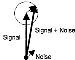
(a) Vector representation of homodyne noise
