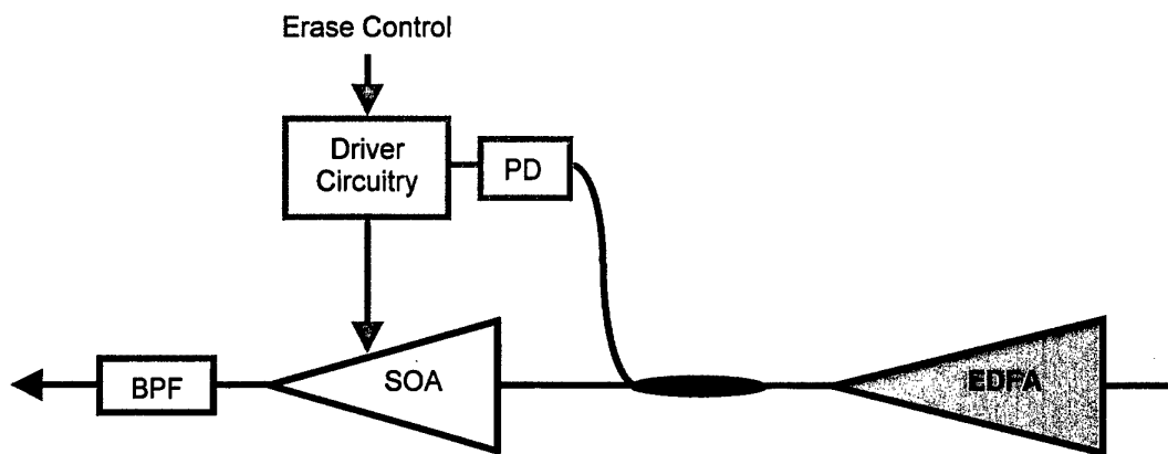
(b) EDFA
