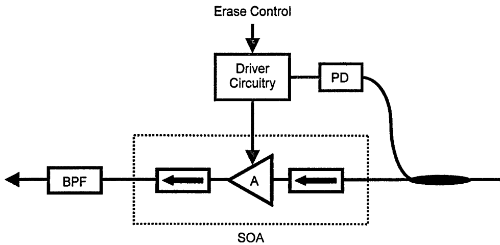
(a) SOA
