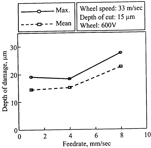
Fig. 8. Effects of feedrate on depth of damage of ground n\text{-Al}_2\text{O}_3/13\text{TiO}_2 coatings.
