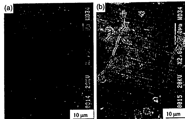
Fig. 2. Surface cracks on the n\text{-Al}_2\text{O}_3/13\text{TiO}_2 surface ground by 10 kC wheel.
