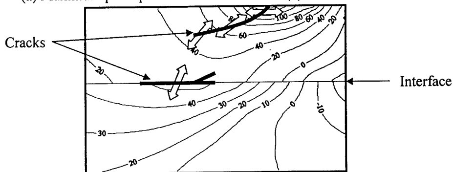
(b) Maximum shear stress
