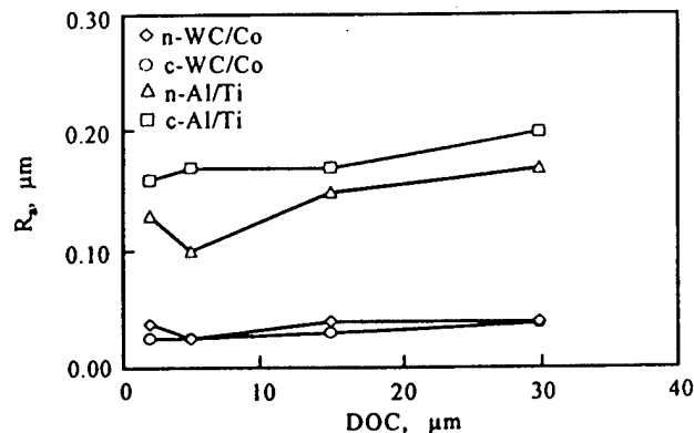
Fig. 4 Variations of surface roughness with DOC for 1 kC wheel, at feedrate=4 mm/sec.
