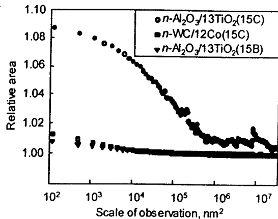
Figure 3: Area-scale plot of the coatings ground at depth of cut of 15\ \mu\text{m} and feedrate of 1\ \text{mm}/\text{sec} .
