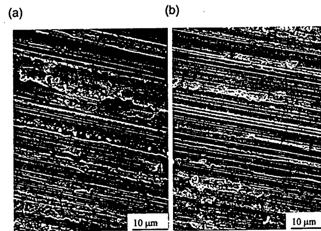
Fig. 16. WC/12Co coatings ground with 120 V wheel at different feedrates, a depth of cut of 15 \mu\text{m} and a wheel speed of 33 m/s. (a) Feedrate of 4 mm/sec; (b) feedrate of 8 mm/sec.
