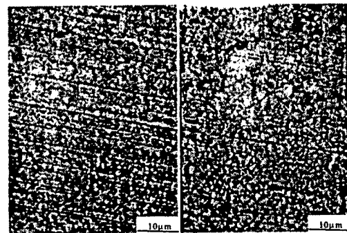
(a) n\text{-WC}/12\text{Co} (b) c\text{-WC}/12\text{Co}
