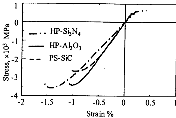
Fig. 3 Stress-strain correlations for HP-Si 3 N 4 , HP-Al 2 O 3 and PS-SiC
