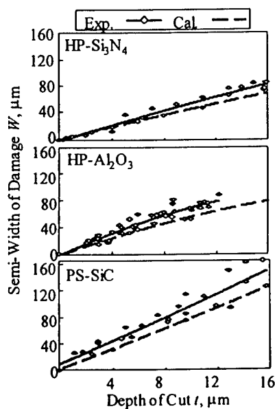
(a) Prediction for the semi-width of damage vs. depth of cut
