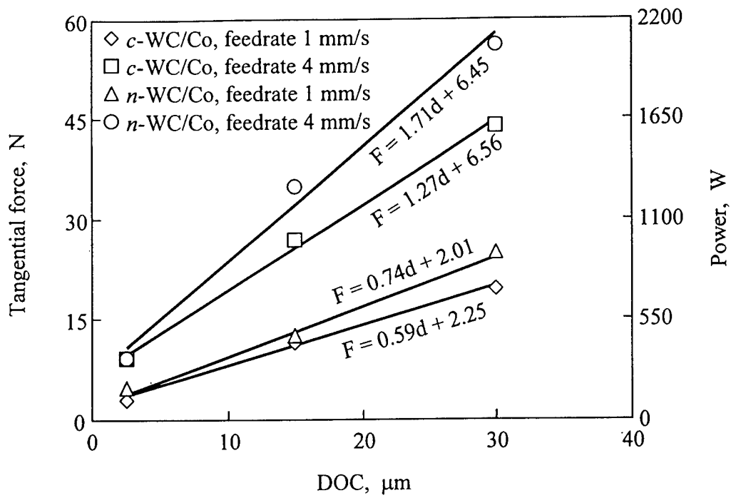
Fig. 10 Tangential forces with different coatings and federates vs. DOC for 240B wheel.
