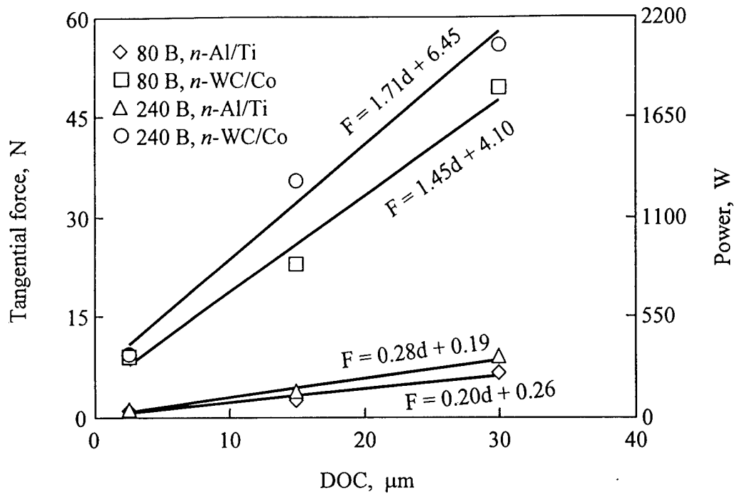
Fig. 8 Tangential forces vs. DOC for n -Al/Ti and n -WC/Co coatings at a feedrate of 4 mm/s.
