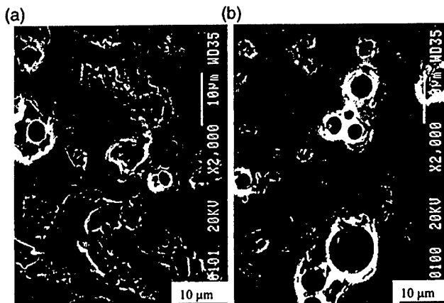
Fig. 11. \text{Al}_2\text{O}_3/13\text{TiO}_2 coatings ground with 1 kC and 1000 B wheels at a depth of cut of 15 \mu\text{m} , a feedrate of 4 mm/s and a wheel speed of 33 m/s. (a) With 1kC wheel; (b) With 1000B wheel.
