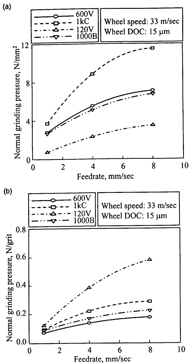
Fig. 6. Normal grinding force versus the feedrate for grinding n -WC/12Co coatings. (a) Normal grinding force (force per area) vs. feedrate; (b) Normal grinding force (force per grit) vs. feedrate.
