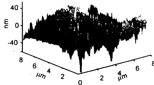
(a) n\text{-Al}_2\text{O}_3/13\text{TiO}_2 ground with 15B wheel.
