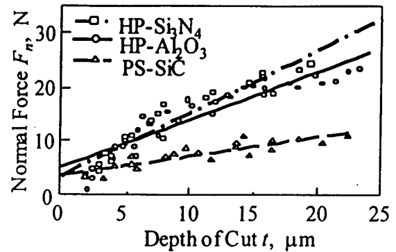
Fig. 5 The relationship between the normal force and the depth of cut for the three ceramics
