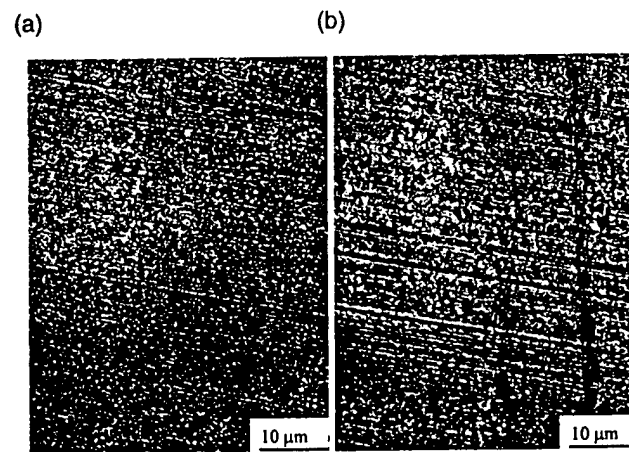
Fig. 14. WC/12Co coatings ground with 600 V wheel at different feedrates at a depth of cut of 15 \mu\text{m} and a wheel speed of 33 m/s. (a) Feedrate of 1 mm/sec; (b) feedrate of 8 mm/sec.
