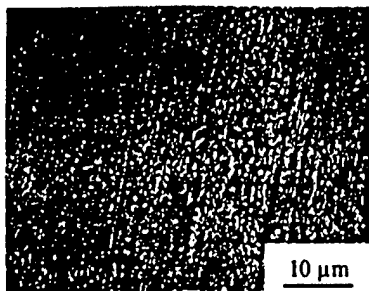
Fig. 14 SEM observation of the ground surface of n-WC/Co (Wheel: 1 kC, DOC= 2 μm, feedrate = 4 mm/sec).
