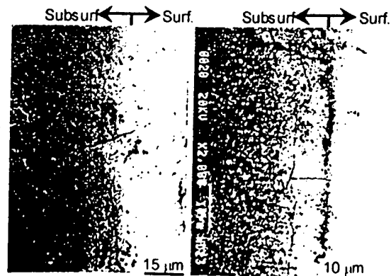
Figure 6: Subsurface observations of ground n\text{-WC}/12\text{Co} coatings.
