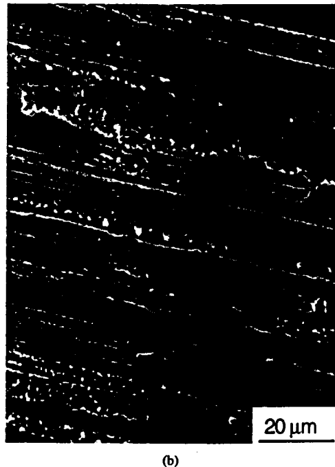
Figure 12 Effect of wheel grit sizes on residual stress and SEM observation of an n\text{-WC}/12\text{Co} coating ground with 120 V wheel. (a) Compressive residual stresses \sigma_{\perp}(\sigma_{xx}) vs. wheel grit sizes in a ground n\text{-WC}/12\text{Co} coating. (b) SEM observation of plastic deformation in an n\text{-WC}/12\text{Co} coating ground with 120 V wheel (grinding conditions shown in (a)).
