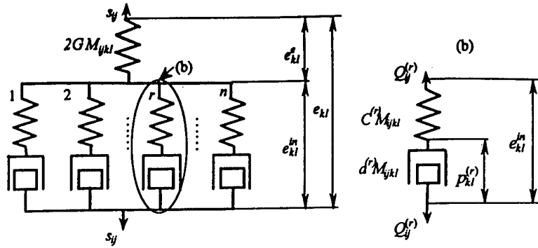
Fig. 1 Mechanical representation of CDM model
