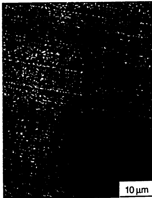
Figure 4 Depth profiles of residual stresses and SEM surface image of a ground n -WC/12Co coating. (a) Depth profiles of residual stresses in a ground n -WC/12Co coating. (b) SEM image of the surface of a ground n -WC/12Co coating (grinding conditions shown in (a)).
