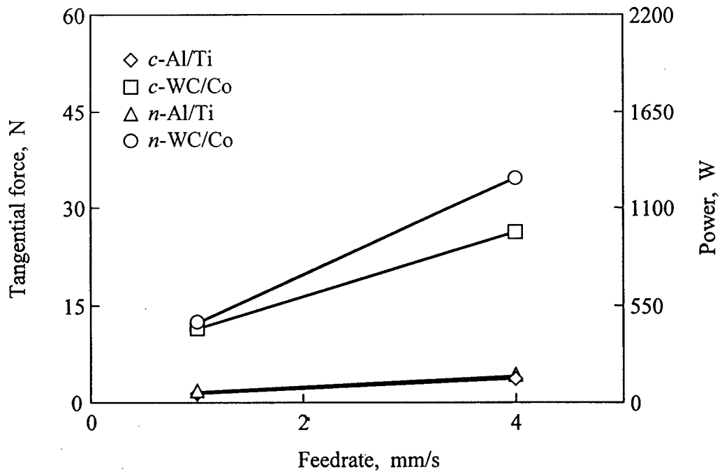
Fig. 9 Tangential forces vs. feedrate for 240B wheel at DOC = 15 \mu\text{m} .
