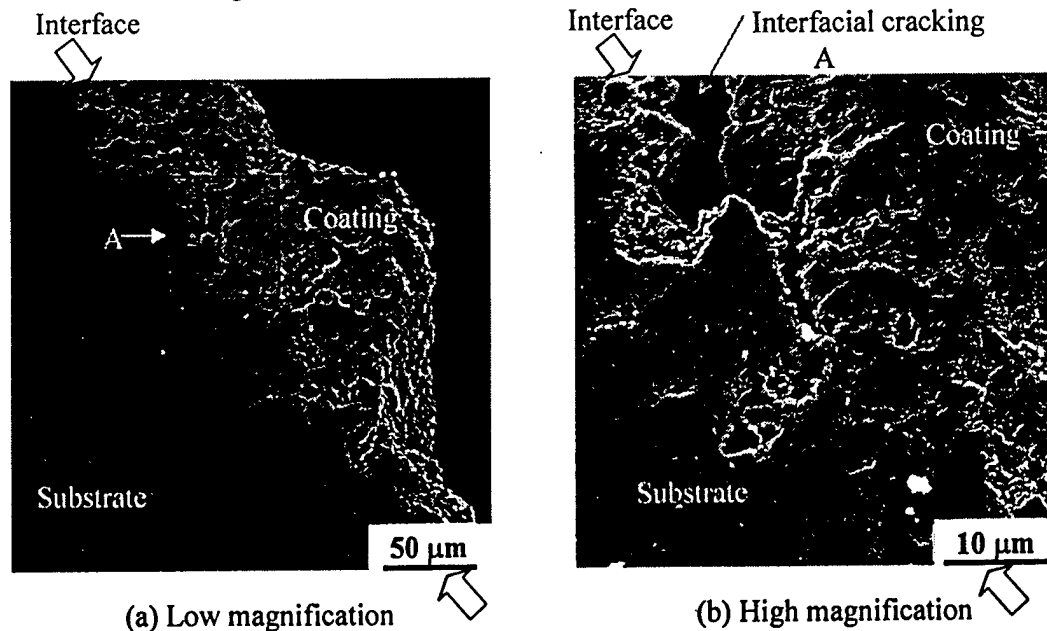
Figure 19 SEM micrographs showing cracks at the coating-substrate interface of n-Al 2 O 3 /13TiO 2 after wear test under 100 N normal load.
