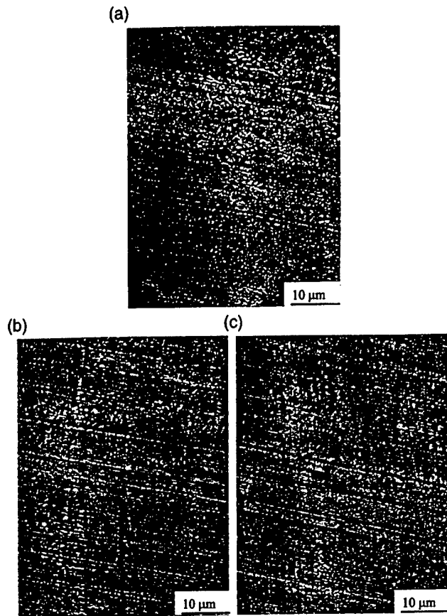
Fig. 13. WC/12Co coatings ground with a 600 V wheel at different depths of cut at a feedrate of 4 mm/s and a wheel speed of 33 m/s. (a) Depth of cut of 2 \mu\text{m} ; (b) Depth of cut of 15 \mu\text{m} ; and (c) Depth of cut of 30 \mu\text{m} .
