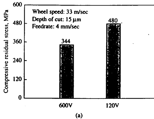
Figure 11 Compressive residual stress \sigma_{\perp}(\sigma_{xx}) vs. different wheel bond types in ground n\text{-Al}_2\text{O}_3/13\text{TiO}_2 coating.
