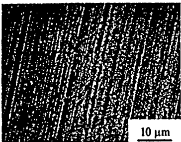
Fig. 15 SEM observation of the ground surface of n-WC/Co (Wheel: 1 kC, DOC= 15 μm, feedrate= 4 mm/sec).
