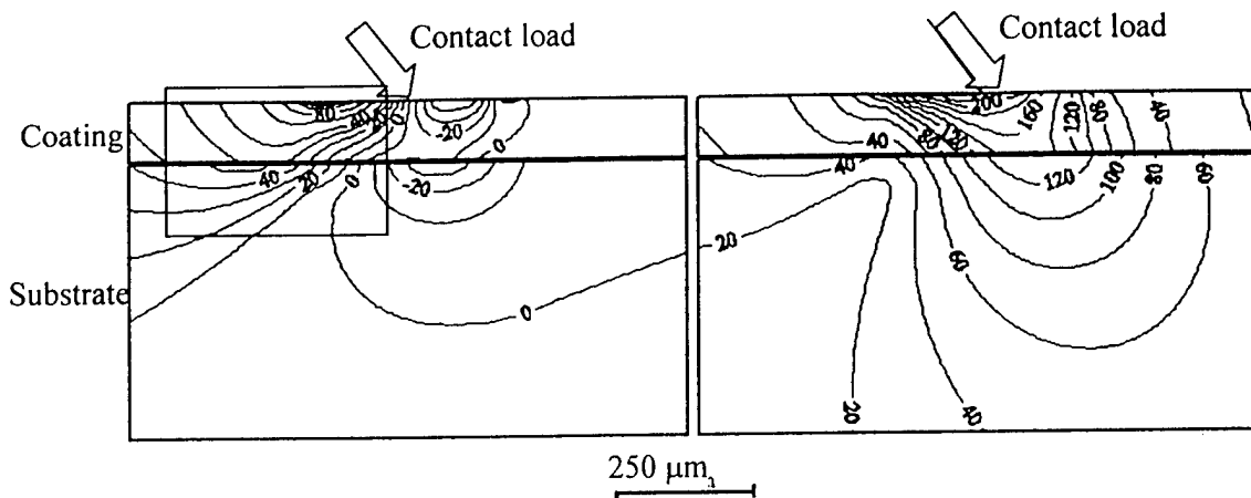
(b) Maximum shear stress
