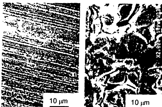
(a) n\text{-WC}/12\text{Co} . (b) n\text{-Al}_2\text{O}_3/13\text{TiO}_2 .
