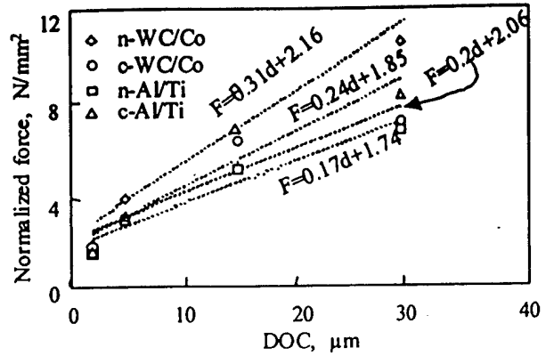
Fig. 10 Normalized force variations of different coatings with DOC using 1 kC wheel (Dotted lines showing simulation results).
