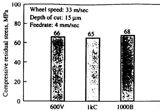
Figure 11 Compressive residual stress \sigma_{\perp}(\sigma_{xx}) vs. different wheel bond types in ground n\text{-Al}_2\text{O}_3/13\text{TiO}_2 coating.
