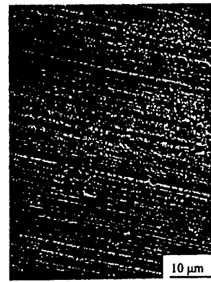
Fig. 15. WC/12Co coatings ground with a 1 kC wheel at a feedrate of 4 mm/s, a depth of cut of 15 \mu\text{m} and a wheel speed of 33 m/s.
