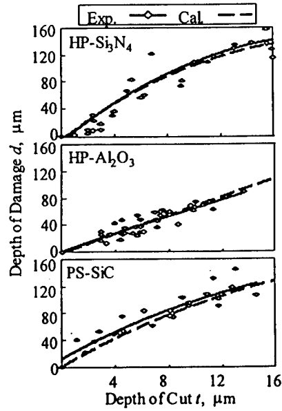
(b) Prediction for depth of damage vs. depth of cut
