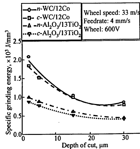
Fig. 5 Comparison of specific grinding energy.
