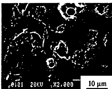
Fig. 17 SEM observation of the ground surface of n-Al/Ti (Wheel: 1 kC, DOC= 15 μm, feedrate= 4 mm/sec).
