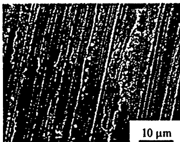
Fig. 16 SEM observation of the ground surface of n-WC/Co (Wheel: 120V, DOC= 15 μm, feedrate= 4 mm/sec).
