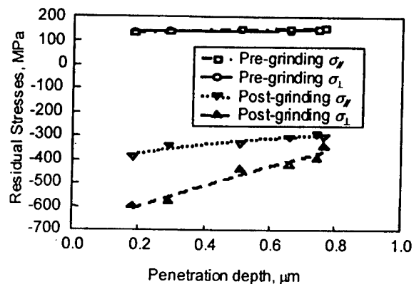
(a) n\text{-WC}/12\text{Co} .
