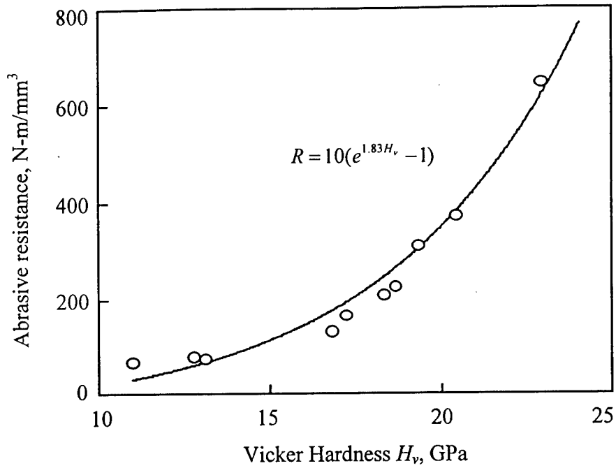
Fig. 1 Effect of material hardness on abrasion resistance for various tungsten carbides. The abrasion resistance of a tungsten carbide is an exponential function of its hardness [Jia and Fischer, 1996].
