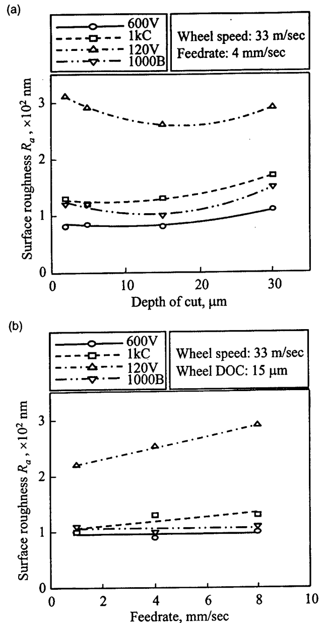
Fig. 7. Surface roughness R_a for ground n -Al 2 O 3 /13TiO 2 coatings. (a) Surface roughness R_a vs. depth of cut; (b) Surface roughness R_a vs. feedrate.
