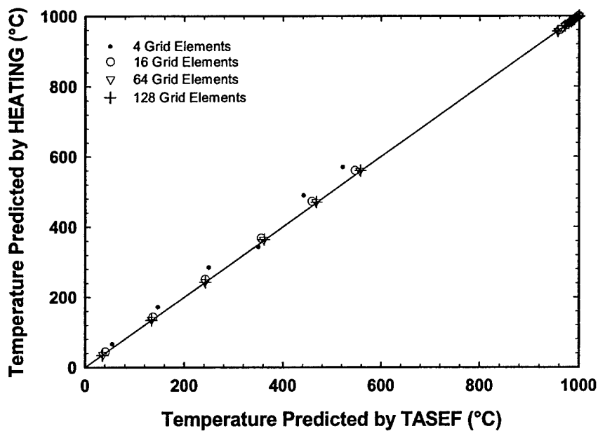
Fig. C-6 — HEATING and TASEF temperature predictions for Reference Case 3 — constant 1,000 °C exposure temperature.
