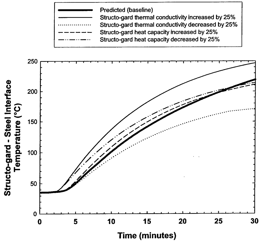
Fig. D-20 — Sensitivity of Structo-gard – Steel Interface Predicted Temperature to Uncertainty in the Material Property Data
