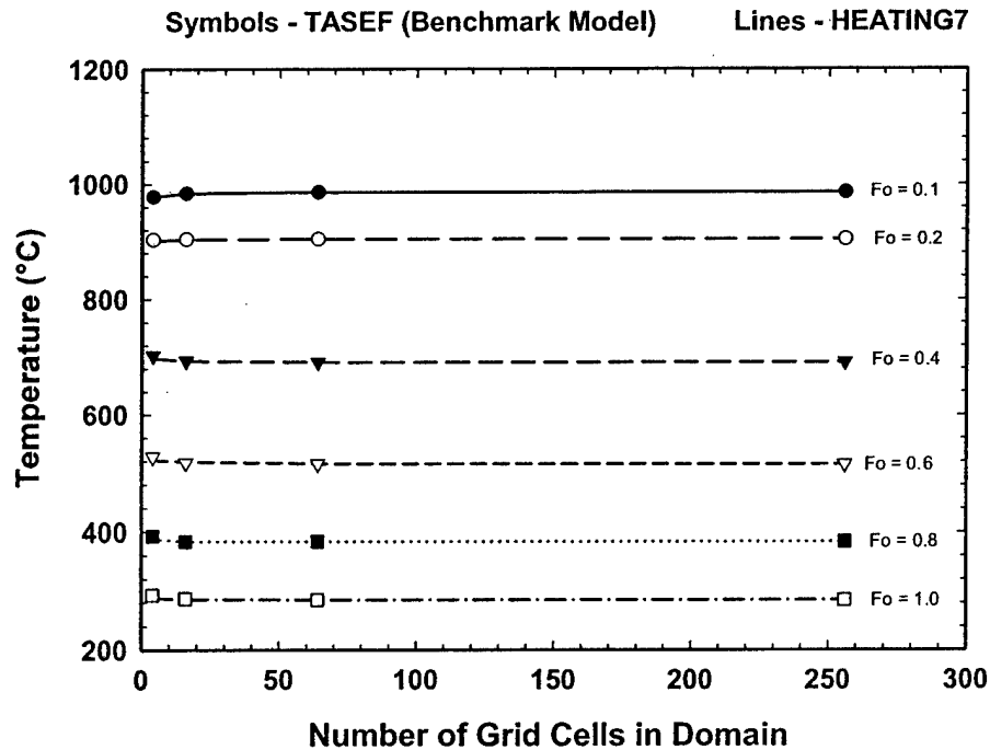
Fig. C-2 - Center temperature for Reference Case 1 as a function of the number of grid cells.
