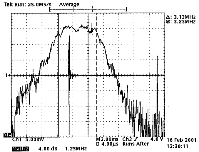
Figure 17b Broadband Composite Transducer
