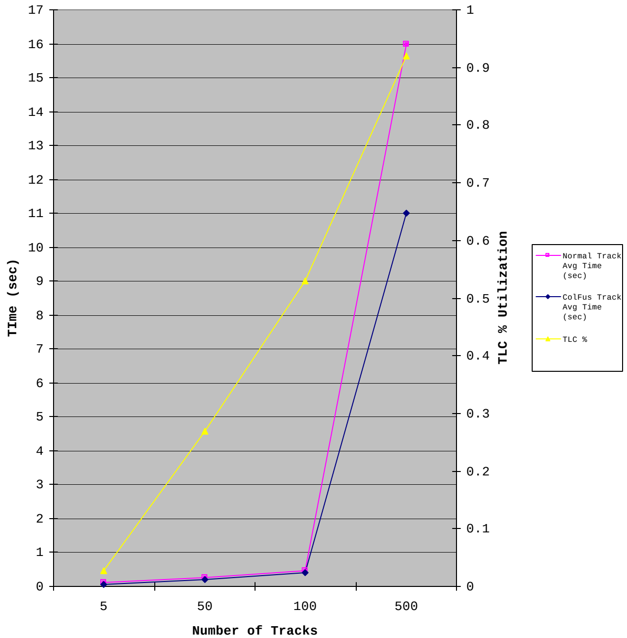
Figure 44. Varying Data Rates and Track Message Sizes
