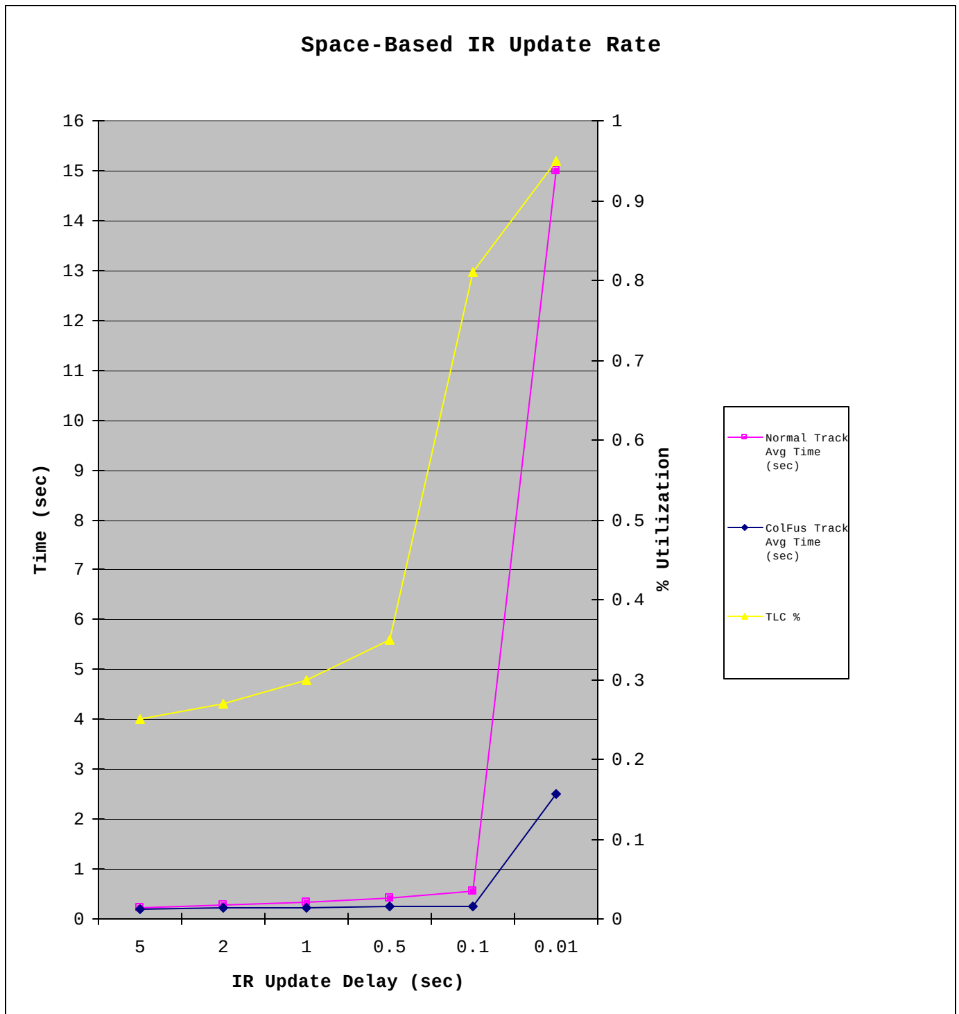
Figure 46. Space-Based IR Update Delay
