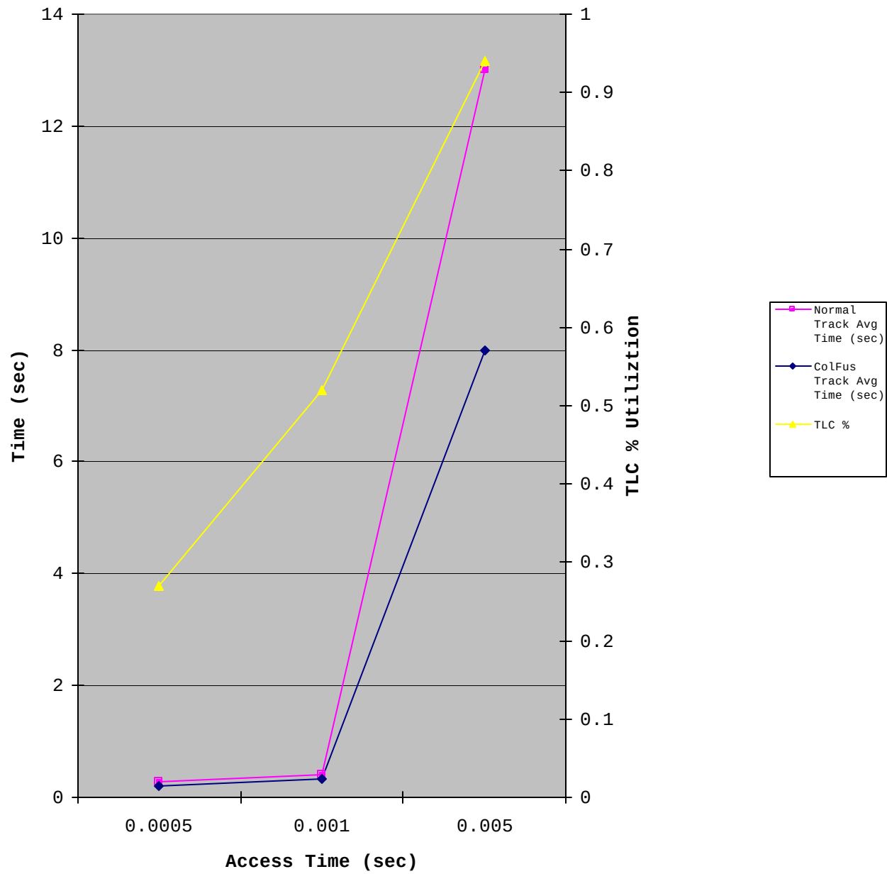
Figure 51. Track List Access Time
