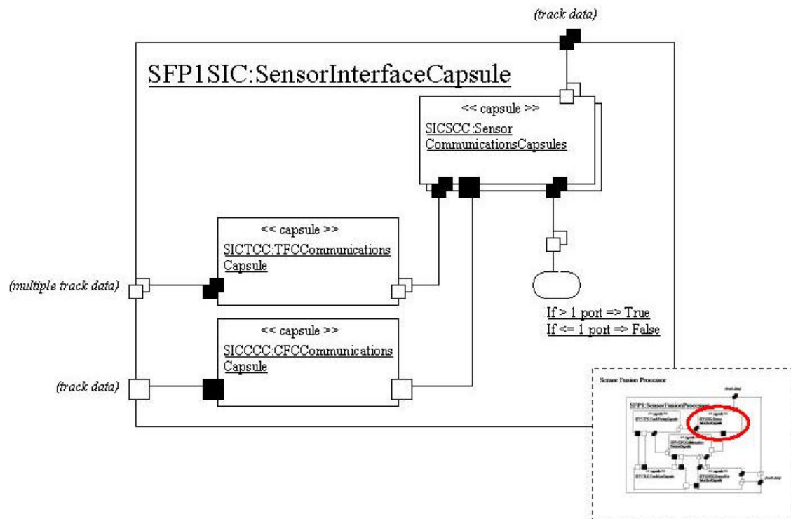
Figure 27. Sensor Interface Capsule UML-RT Diagram
