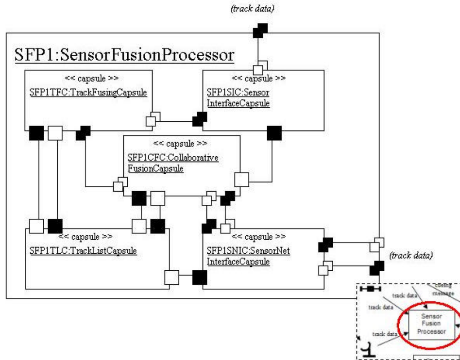
Figure 26. Sensor Fusion Processor UML-RT Diagram
