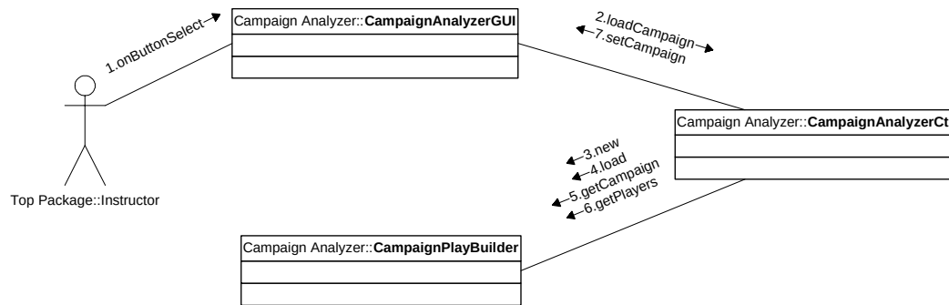
Figure 47. [UC4.1] Scenario: Select Campaign.
