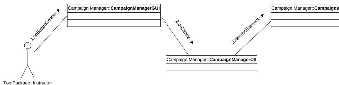
Figure 41. [UC2.3] Scenario: Delete Campaign.
