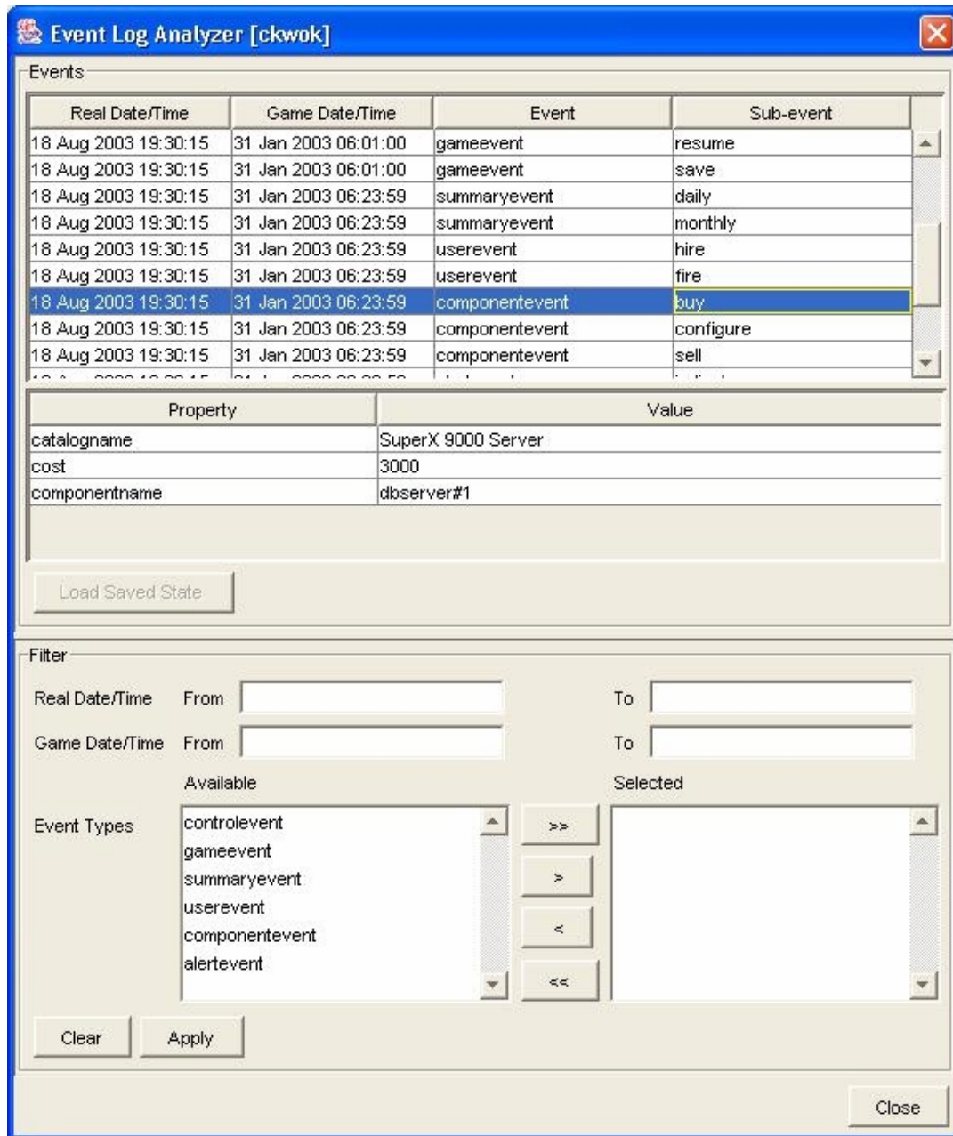
Figure 23. Event Log Analyzer.
