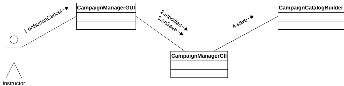
Figure 43. [UC2.5] Scenario: Cancel/Close Campaign Management Session.
