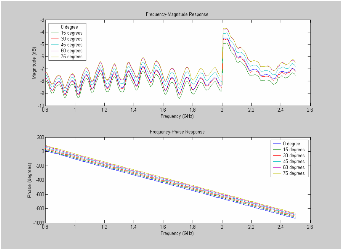
Figure 17. Magnitude and Phase Versus Frequency Response for Phase Shift From 0° to 75° at 5° Increments.
