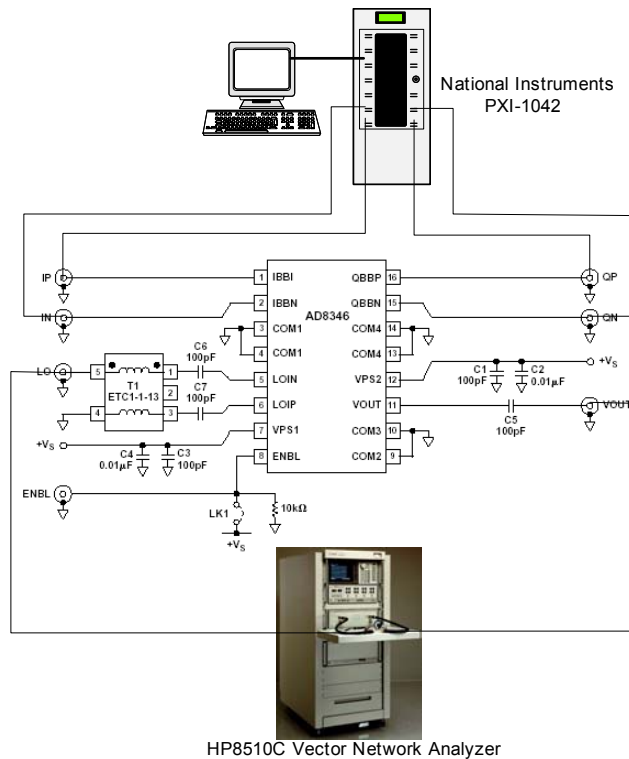
Figure 11. AD8346EVAL Bench Test Configuration.
