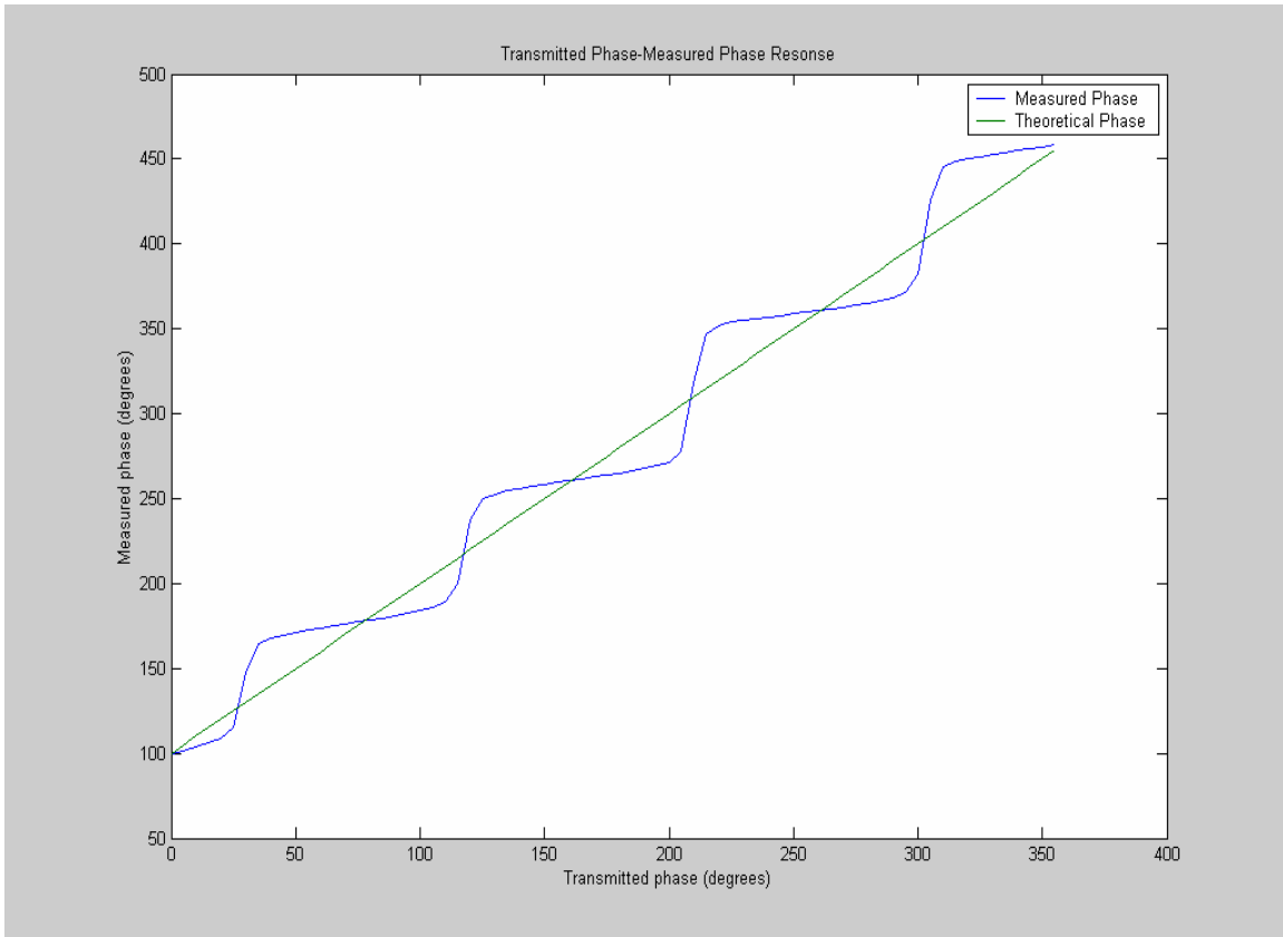
Figure 34. Transmitted Phase Versus Measured Phase Resonse.
