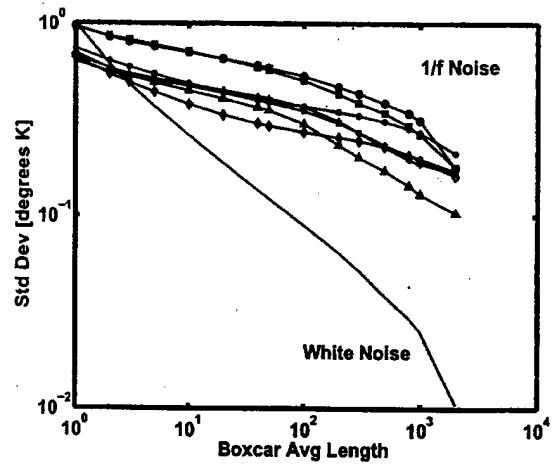
Figure 5: Variance in the time series for all six beams for a calibration run, as a function of the boxcar averaging length. The plain line is for white noise, while the upper line with circles is for 1/f noise.
