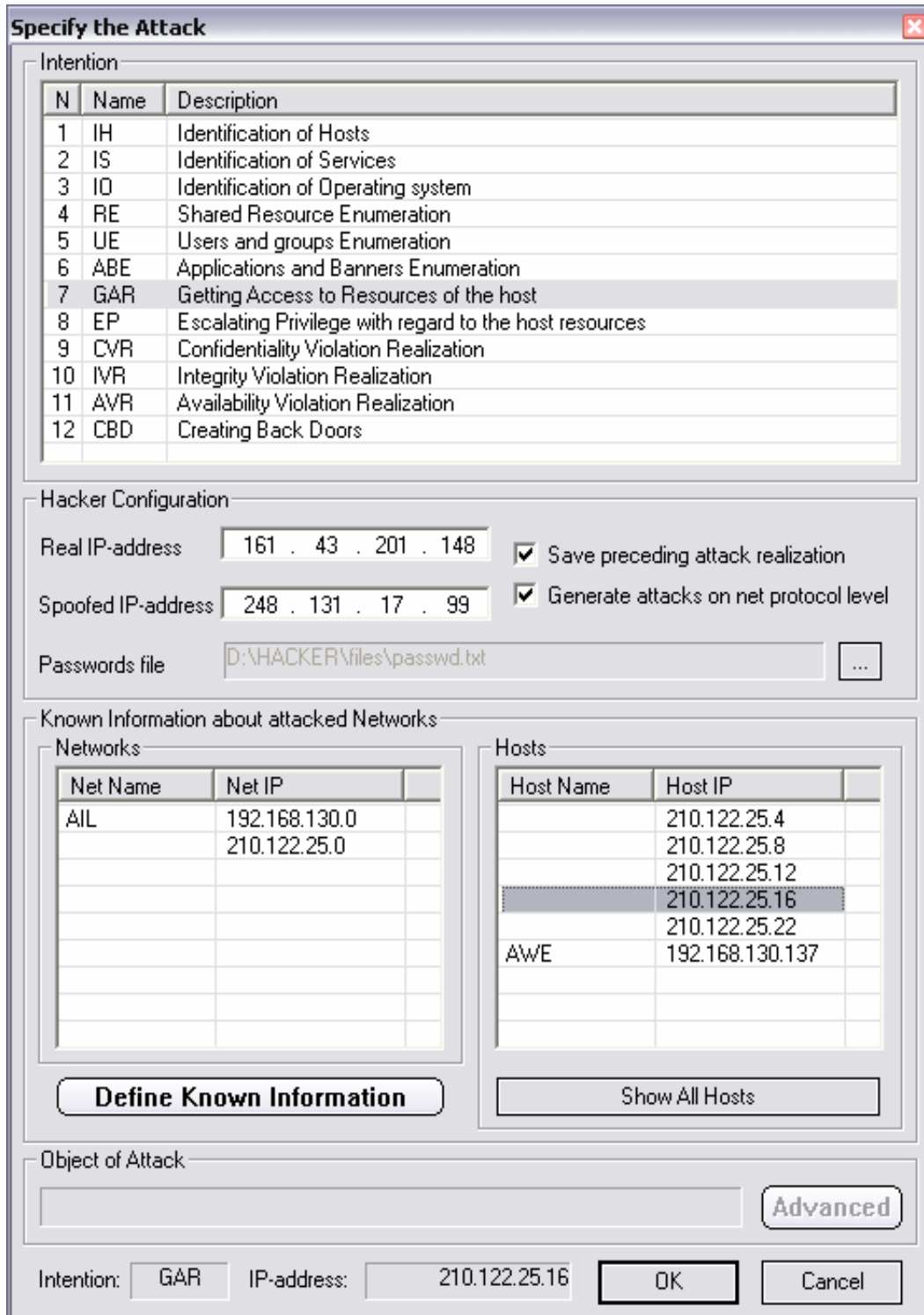
Figure 6. User interface menu for specifying the attack scenario.
