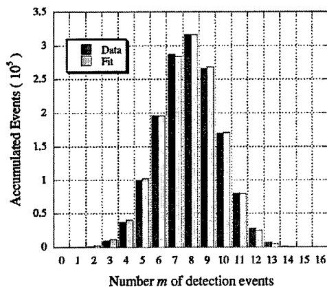
Figure 5. Experimental results obtained from the time-multiplexed photon detector system.
