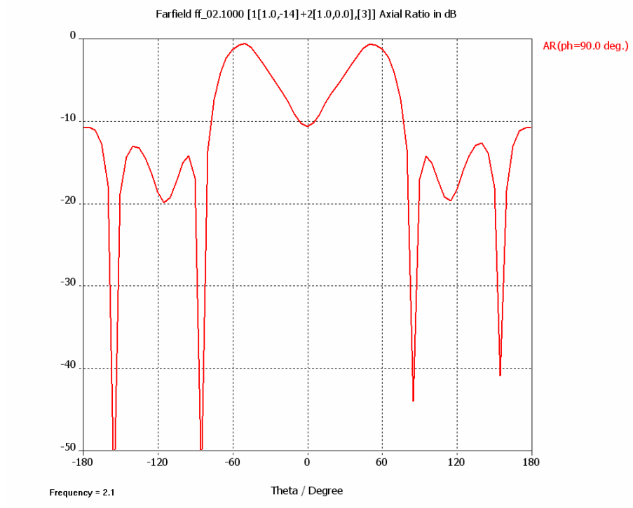
Figure 55. Axial ratio of the antenna at frequency f = 2.1 GHz.
