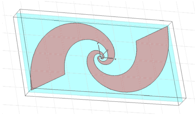
Figure 12. Illustration of a two-arm planar equiangular spiral antenna.
