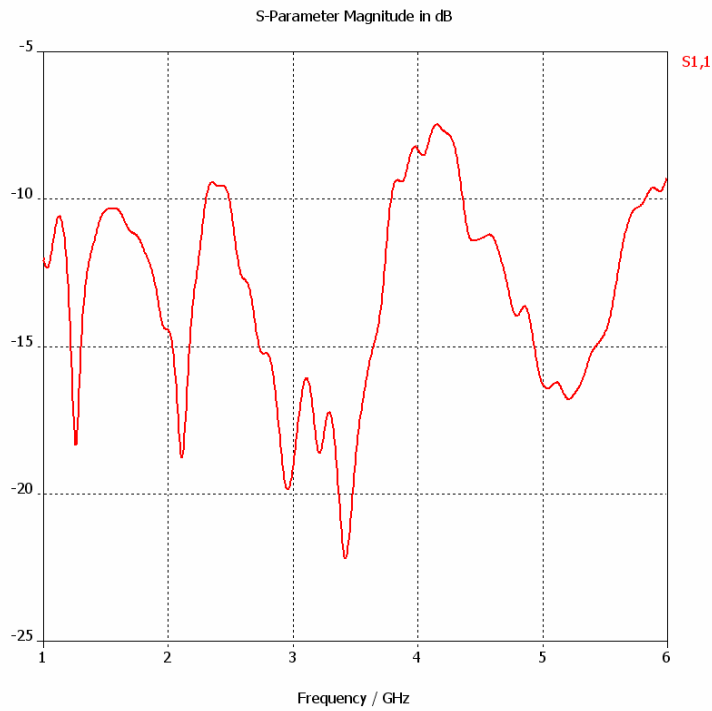
Figure 36. Return loss of the CWSA with substrate thickness of 20 mm.
