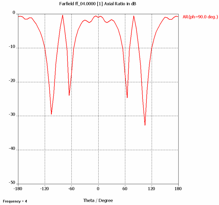
Figure 27. Axial ratio of the spiral antenna at frequency f = 4 GHz.
