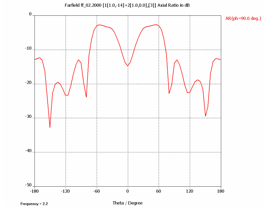
Figure 56. Axial ratio of the antenna at frequency f = 2.2 GHz.
