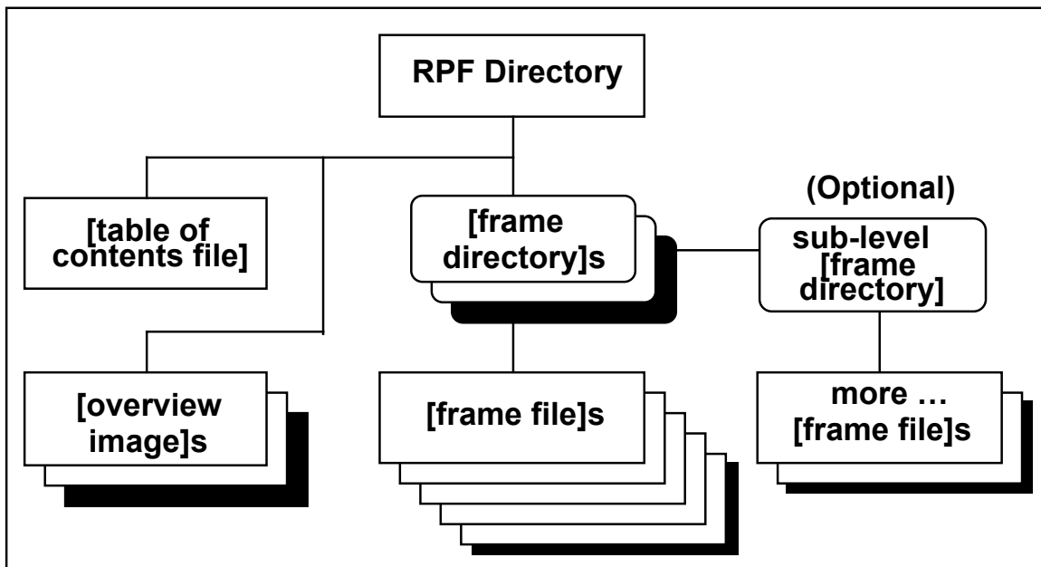
Figure 3-5. Representation of RPF Directory and File Structure
