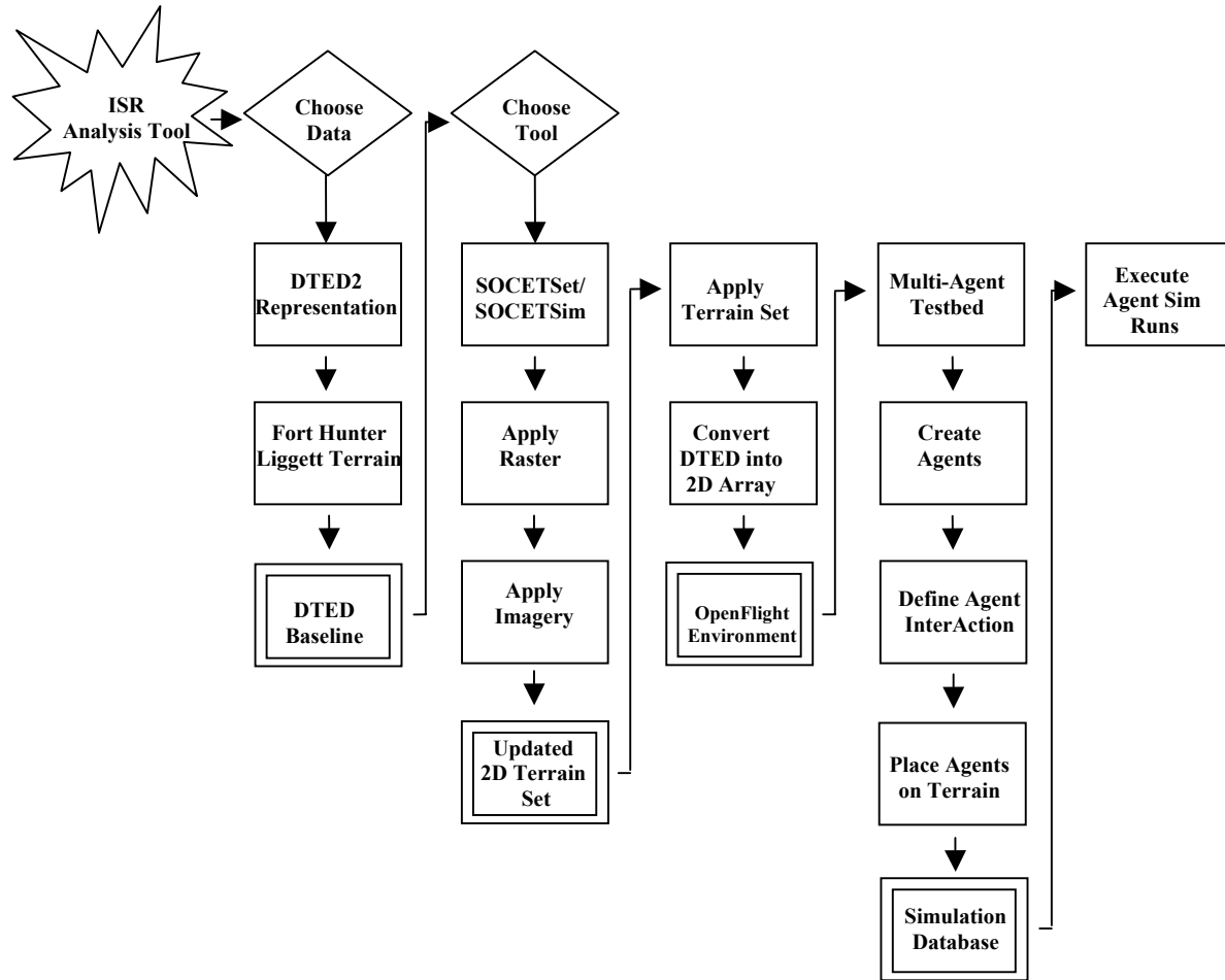
Figure 5-1. Data Flow Diagram Example
