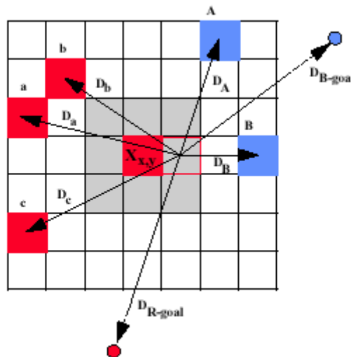
Figure 2-3. Sample Penalty Calculation (From: Ilachinski, 1997)
