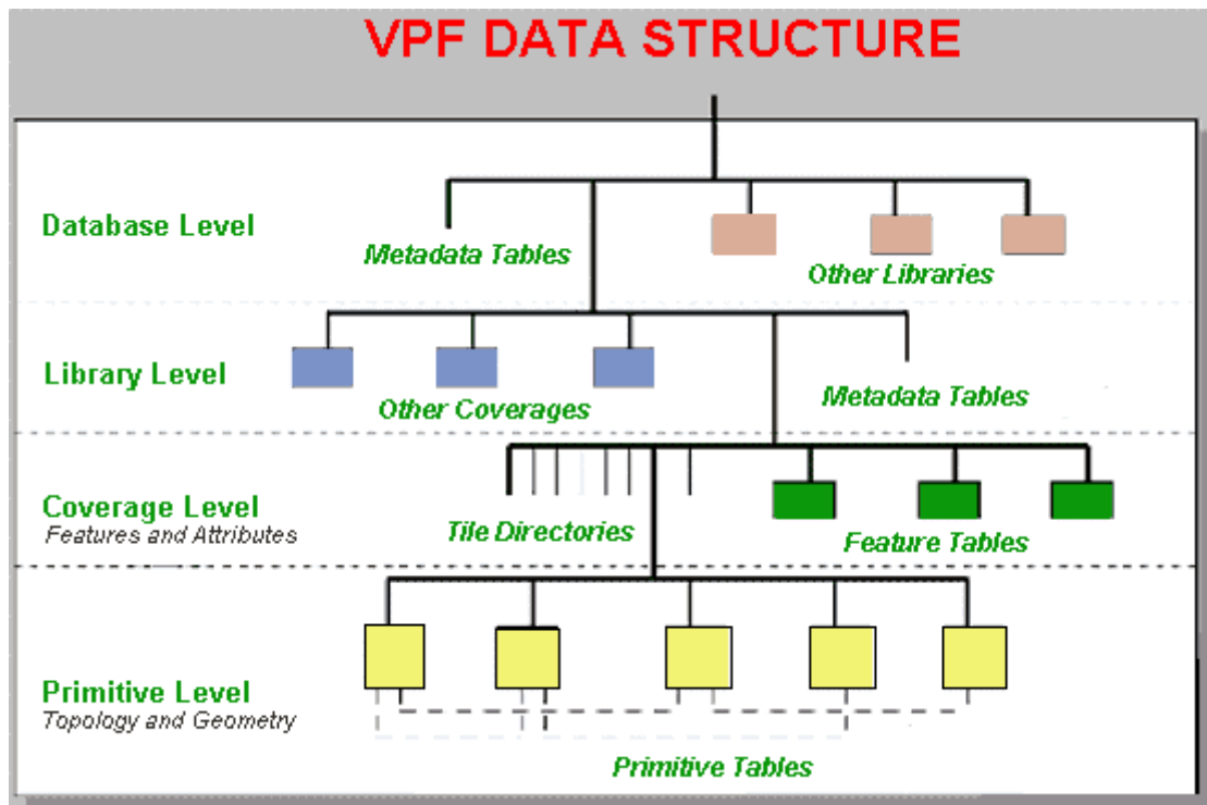
Figure 3-4. VPF Data Structure
