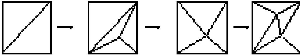
Figure 3-3. Inserting Points Into a Triangulated Irregular Network
