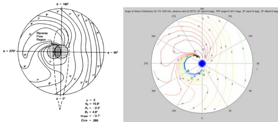
Figure 6. Prouty's Example Helicopter Contour Plot (Left) Compared to JANRAD 2P_RVR Output (Right) Using Prouty's Example Helicopter.
