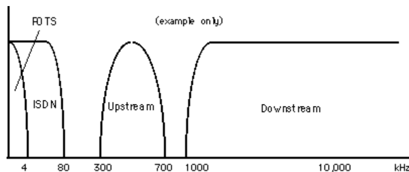
Figure 13. Frequency Division Multiplexing (From [Dsl2001])
