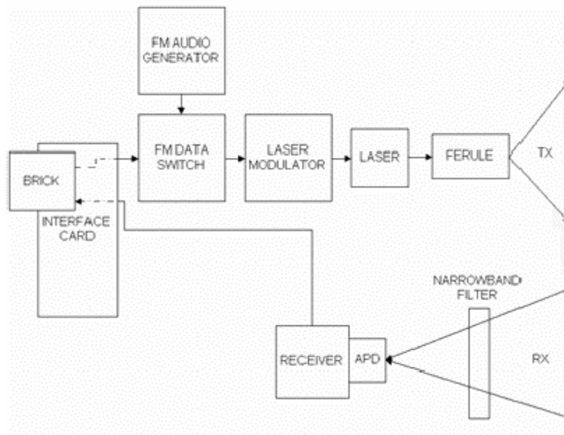
Figure 17. Block Diagram of the Transceiver (From [Will2002])
