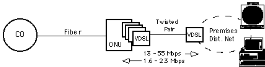
Figure 12. VDSL System (From [Dsl2001])
