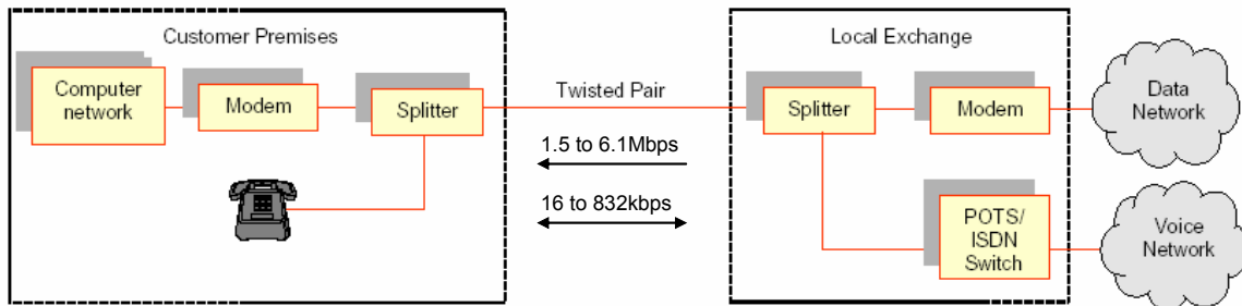
Figure 10. ADSL Configuration (From [Bouy2001])
