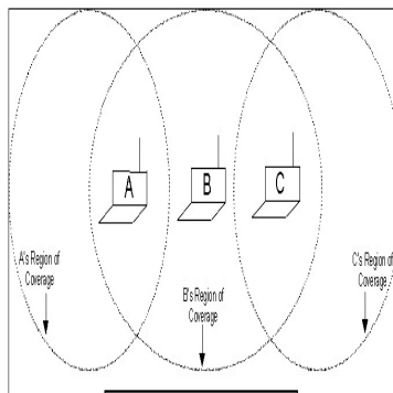
Figure 24. The Hidden Node Problem (From [Loug2000])
