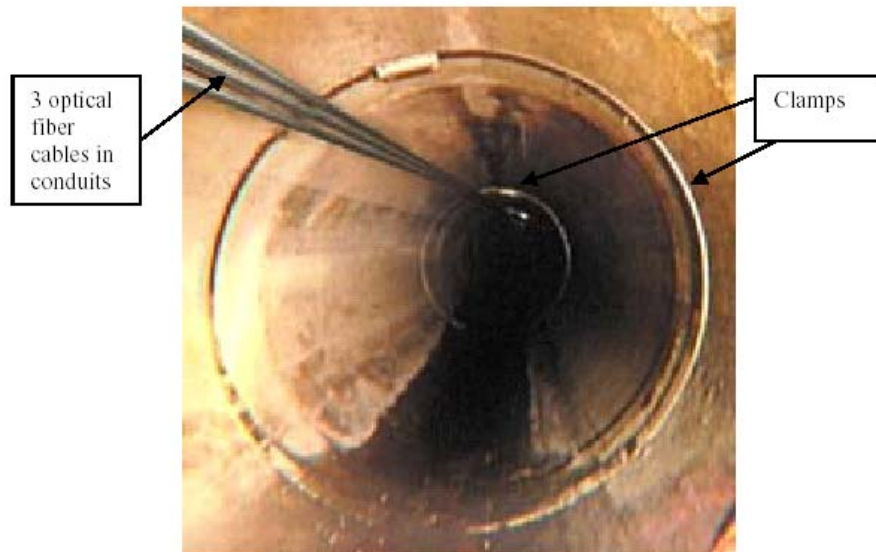
Figure 28. Optical fiber Cables in a Sewer System (From [Jeya2002])
