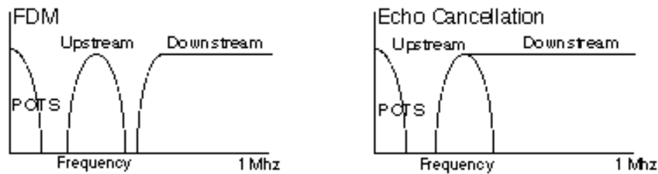
Figure 11. FDM and Echo Cancellation (From [Dsl2001])
