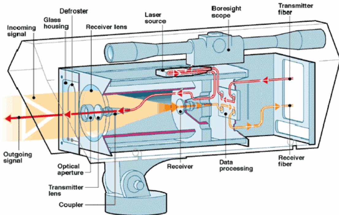
Figure 16. A typical link head for FSO (From [Ligh2003])
