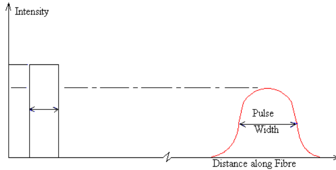
Figure 6. Pulse Spreading in an Optical Fiber
