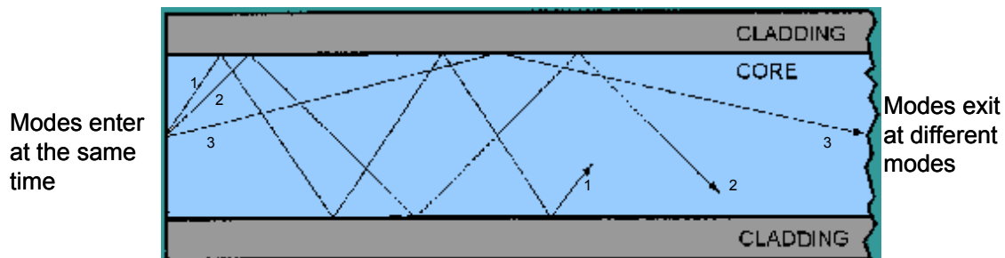
Figure 7. Modal Dispersion
