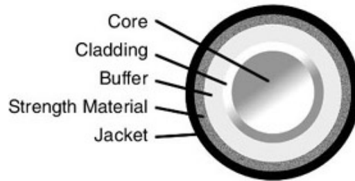
Figure 4. Cross Section of a Fiber Optic Cable (From [Noll2003])
