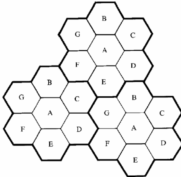
Figure 26. Frequency Reuse (From [Rapp2002])
