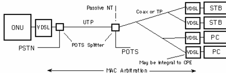
Figure 15. Passive Network Termination (From [Dsl2001])
