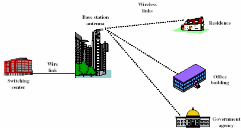
Figure 19. WLL Configuration (From [Stall2002])
