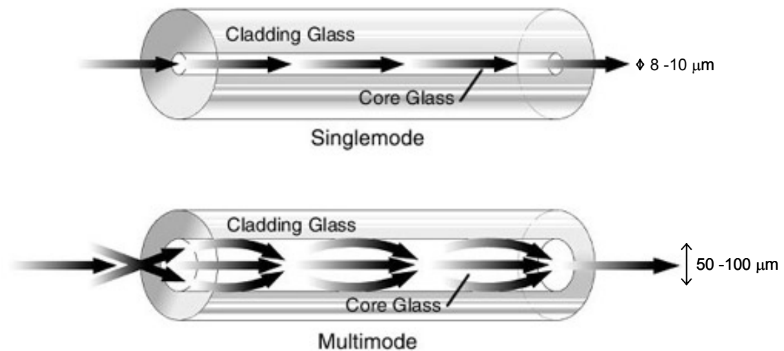
Figure 5. Optical Fiber Core Diameters - Singlemode and Multimode (After [Noll2003])
