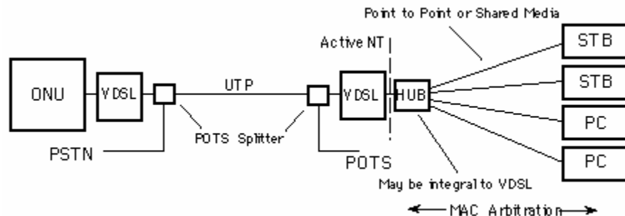
Figure 14. Active Network Termination (From [Dsl2001])
