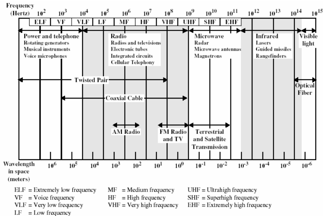
Figure 20. Electromagnetic Spectrum for Telecommunications (From [Stal2002])
