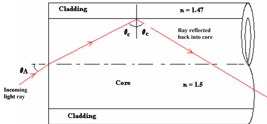
Figure 2. Principle of Total Internal Reflection (TIR)
