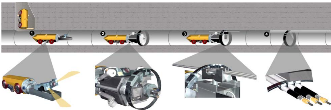
Figure 29. SAM 4-step Installation Procedure (From [City2000])
