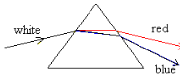
Figure 8. Dispersion of Light through a Prism
