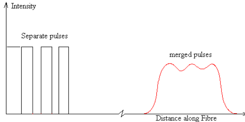
Figure 9. Merging of Pulses in a Fiber.
