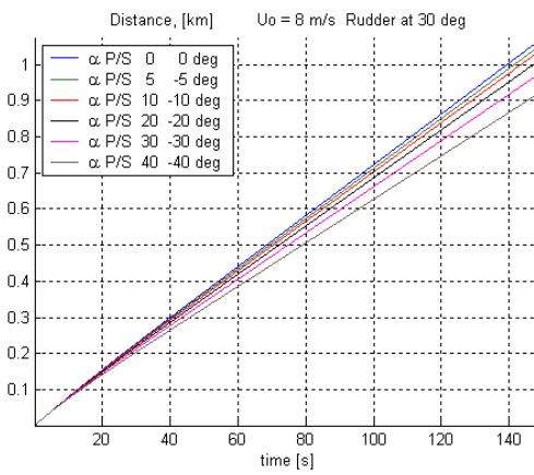
Figure 59. 15.5 Knots, Rudder 30° – Fins: \alpha_p = -\alpha_s ; \alpha_p > 0 \beta_p = \beta_s = 34^\circ .
