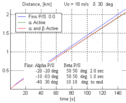
Figure 76. 35 Knots, Rudder 30° Roll Reduction Strategy.
