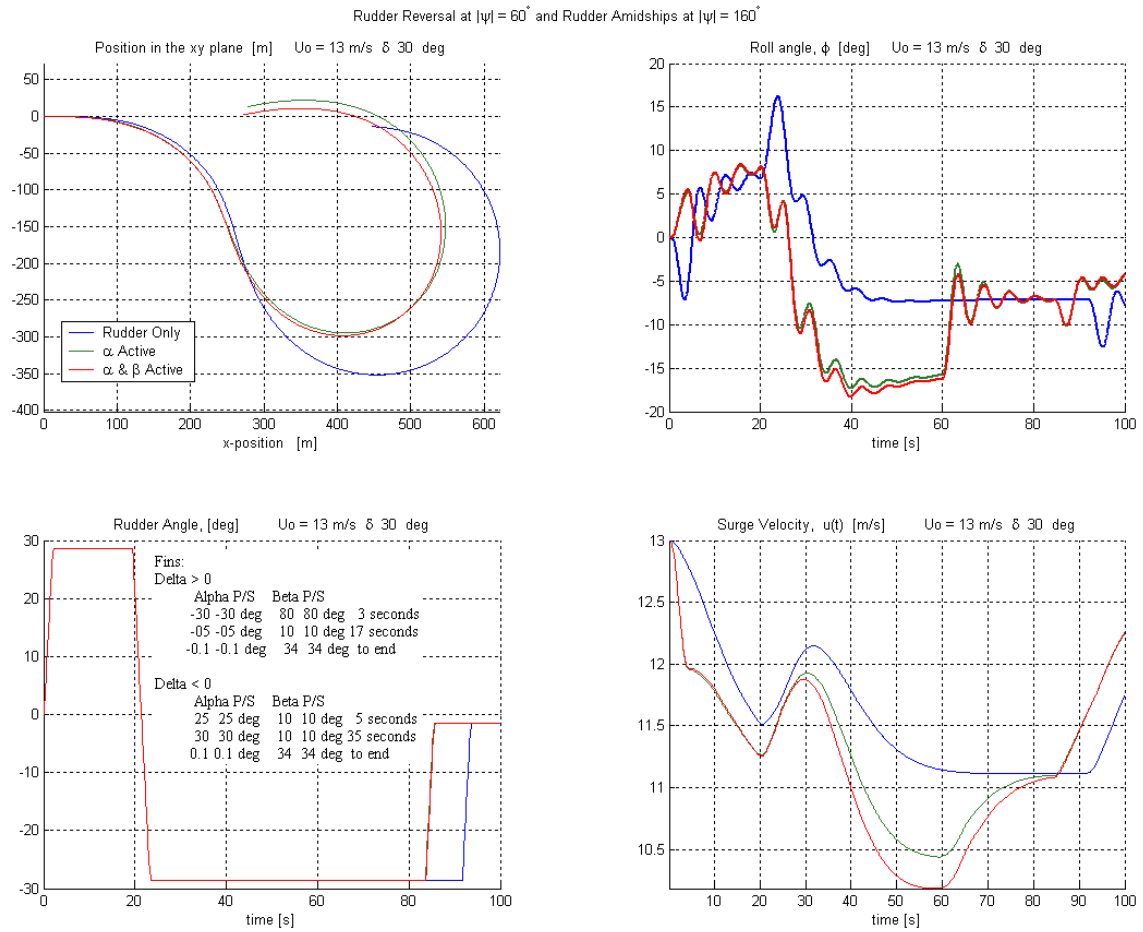
Figure 85. 25 Knots, 30^\circ Rudder Reversed at |\psi| = 60^\circ , Then Amidships at |\psi| = 160^\circ .
