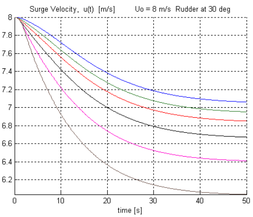
Figure 59. 15.5 Knots, Rudder 30° – Fins: \alpha_p = -\alpha_s ; \alpha_p > 0 \beta_p = \beta_s = 34^\circ .
