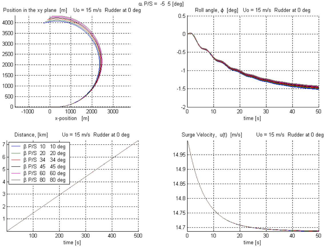
Figure 40. 29 Knots, No Rudder, Fins: \alpha_p = -\alpha_s = -5^\circ \beta_p = \beta_s .
