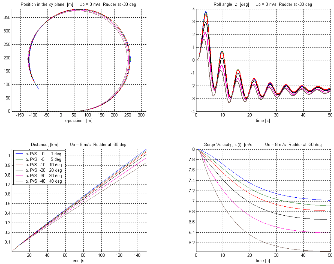
Figure 64. 15.5 Knots, Rudder -30^\circ – Fins: \alpha_p = -\alpha_s ; \alpha_p < 0 \beta_p = \beta_s = 34^\circ .
