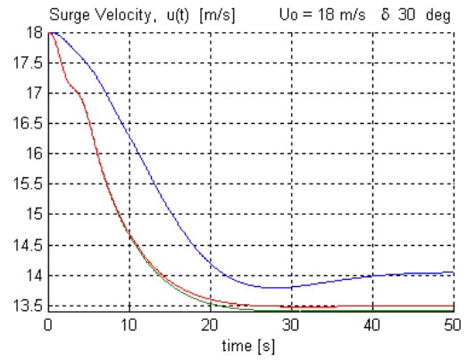
Figure 76. 35 Knots, Rudder 30° Roll Reduction Strategy.
