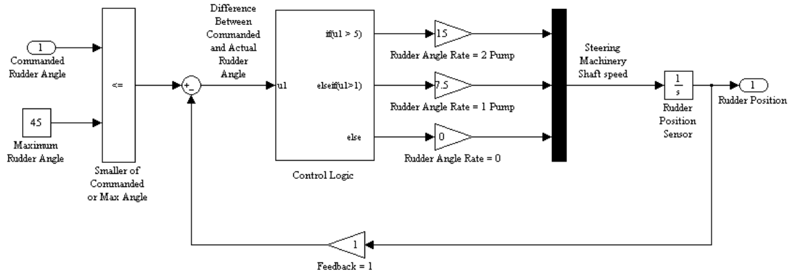
Figure 7. Rudder Dynamics and Control Schematic.
