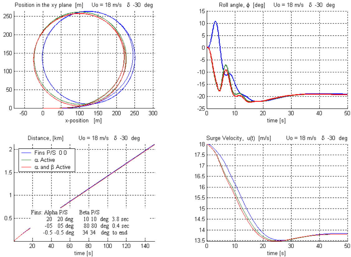
Figure 79. Rudder -30^\circ Advance & Transfer Reduction Strategy – Roll Not Increased.
