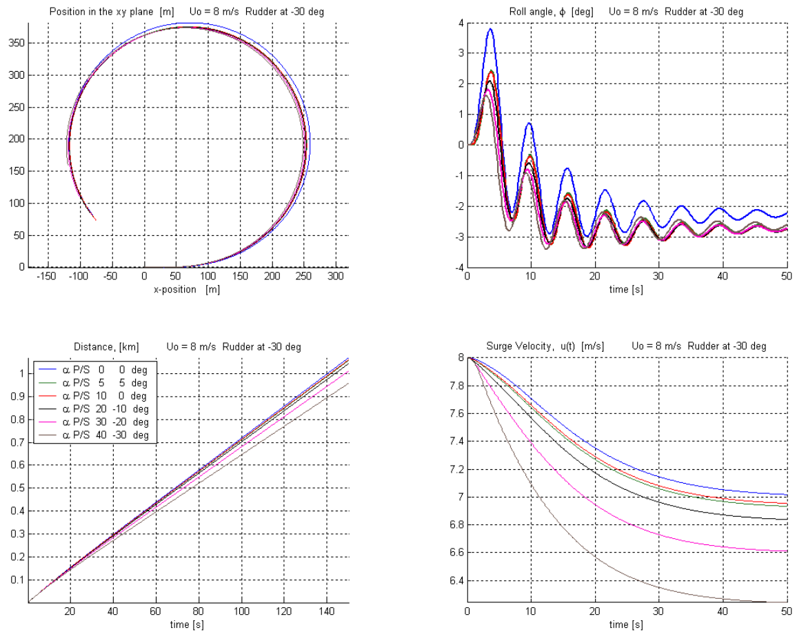
Figure 71. 15.5 Knots, Rudder -30^\circ – Fins: \alpha_P + \alpha_S = 10^\circ ; \alpha_P > 0 \beta_P = \beta_S = 34^\circ .
