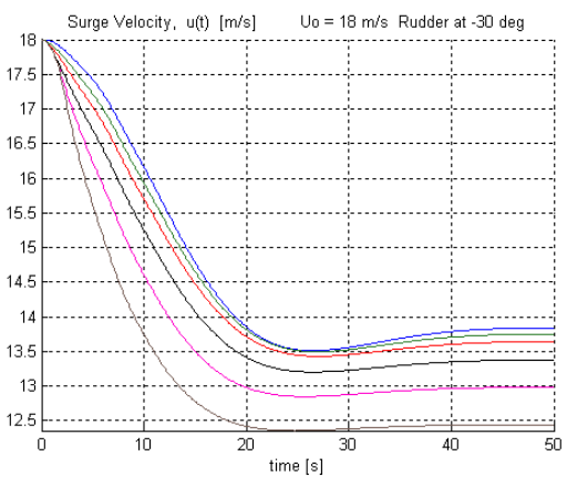
Figure 65. 35 Knots, Rudder -30^\circ – Fins: \alpha_p = -\alpha_s ; \alpha_p > 0 \beta_p = \beta_s = 34^\circ .
