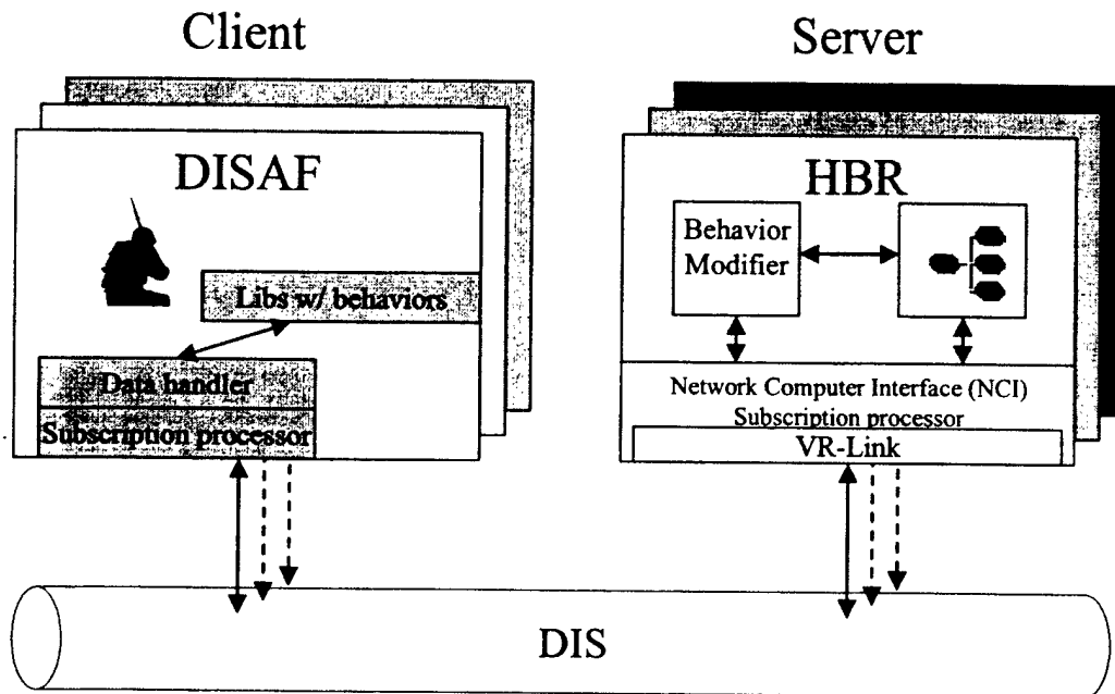
Figure 2. Client-Server architecture.
