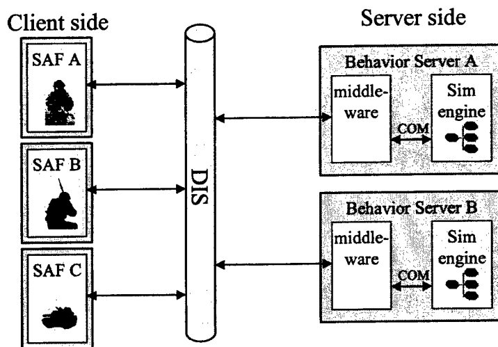
Figure 1. Client-Server federation.
