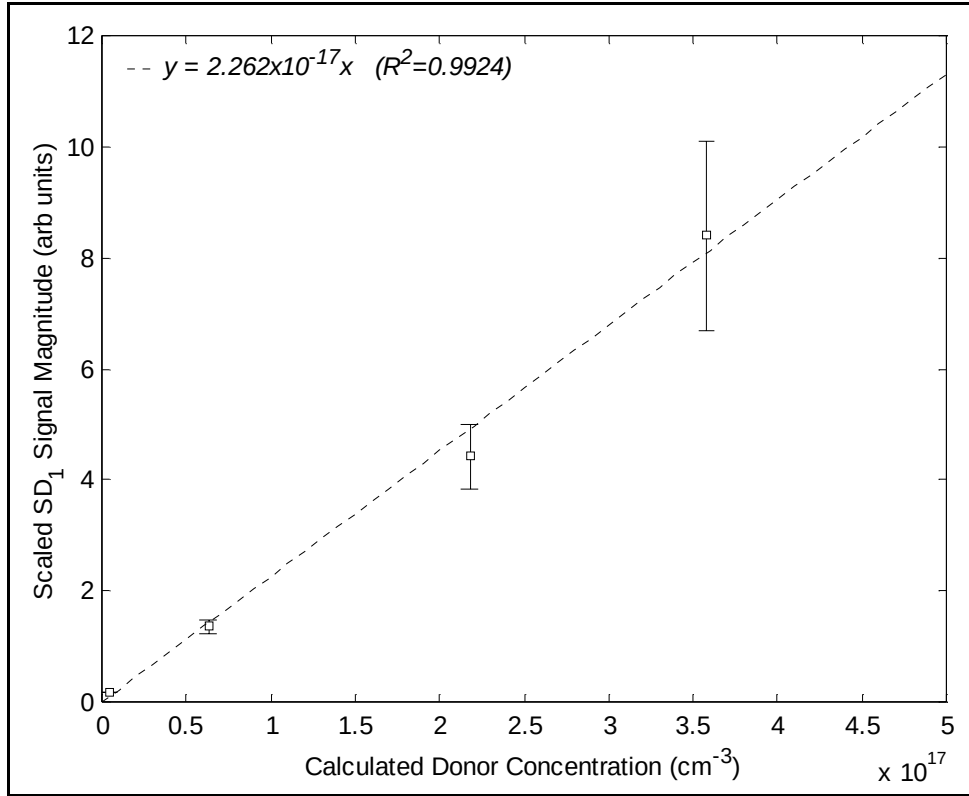
Figure 54. SD 1 scaled EPR magnitude plotted against the calculated shallow donor concentration. Least squares fit is shown as dotted line.
