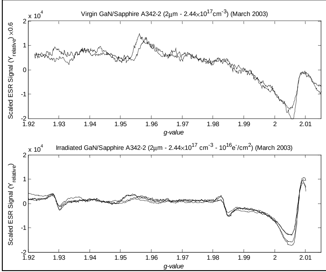
Figure 25. Comparison of virgin and irradiated ( \phi = 10^{16} \text{ e}^- / \text{cm}^2 ) GaN on sapphire (Sample Aa342-1/2). Measurements were conducted on the same day. Note that the data of the lower plot display spurious signals (at g=1.93 and g=1.985 ) as well as differences in \text{TO}_1 linewidths and lineshapes. Magnetic field angles of 0^\circ to 90^\circ are shown in each plot.
