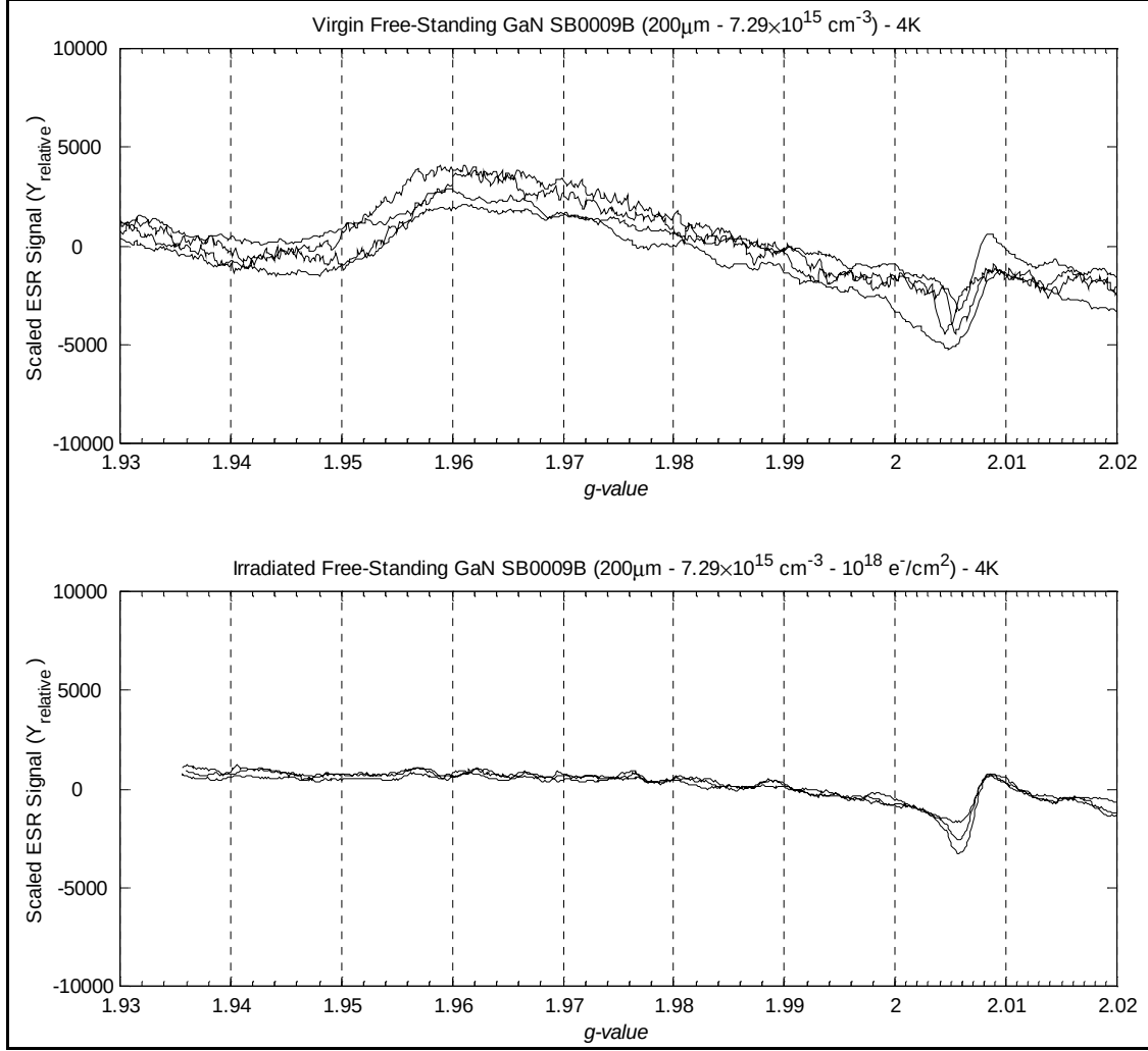
Figure 38. Comparison of virgin and irradiated ( \phi \approx 10^{18} \text{ e}^- / \text{cm}^2 ) free-standing GaN (Sample SB0009B-1). Measurements conducted under similar experimental conditions, same sample subsection. Variation in the g=1.95 signal location is due to rotational anisotropy. Measurements were conducted at 4K sample temperature.
