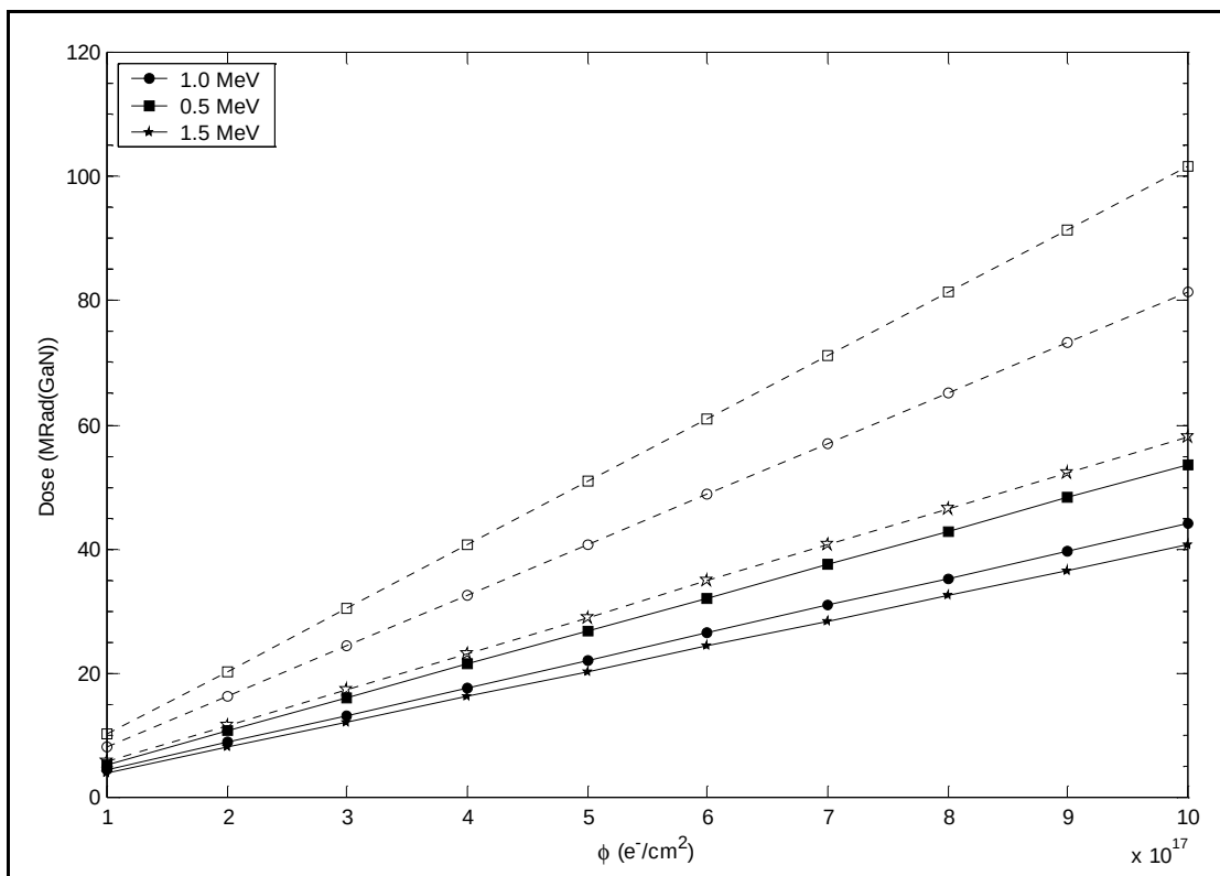
Figure 18. Dose curves (MRad(GaN) vs \phi ) produced via TIGER. Results for 2 \mu\text{m} GaN films on \text{Al}_2\text{O}_3 are shown as solid lines and filled symbols. Results for 200 \mu\text{m} free-standing layers are shown with dashed lines and open symbols.
