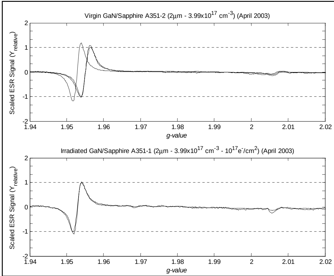
Figure 28. Comparison of virgin and irradiated ( \phi \approx 10^{17} \text{ e}^- / \text{cm}^2 ) GaN on Sapphire (Sample A351). Measurements conducted under identical conditions, same day. Variation in the g=1.95 signal location is due to rotational anisotropy. Experimental difficulties resulted in collection of only two good spectra in the irradiated sample. Magnetic field angles of 0^\circ to 90^\circ are shown in each plot. Angular measurements in this sample were only available at 0^\circ and 90^\circ .
