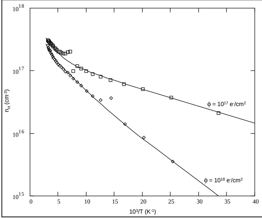
Figure 48. Post-irradiation temperature dependent Hall data for sample A350. For the \phi = 10^{17} \text{ e}^- / \text{cm}^2 case the donor fit yields ( N_{D1}=1.9\text{E}17 , E_{D1}=6.0 \text{ meV} , N_{D2}=3.60\text{E}17 , E_{D2}=50\text{meV} , N_A=1.0\text{E}16 ). For the \phi = 10^{18} \text{ e}^- / \text{cm}^2 case, fit parameters are ( N_{D1}=2.8\text{E}16 , E_{D1}=10.8 \text{ meV} , N_{D2}=2.10\text{E}17 , E_{D2}=27.5\text{meV} , N_A=1.0\text{E}16 ).
