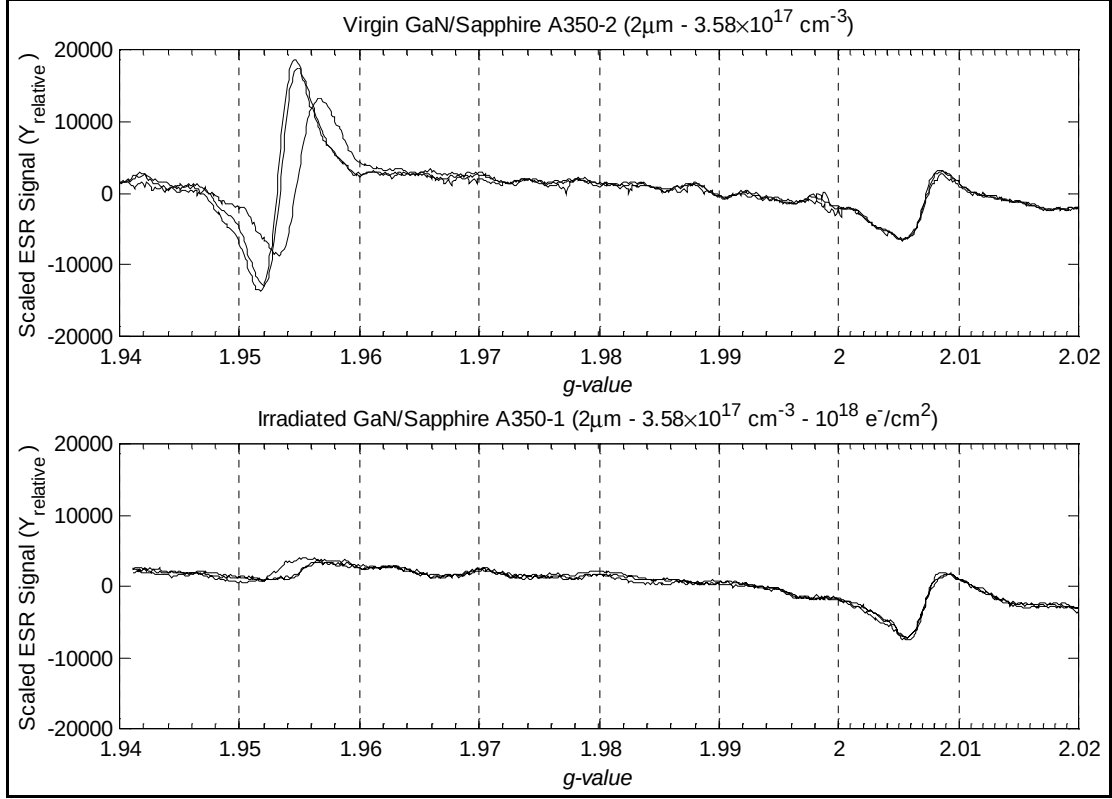
Figure 31. Comparison of virgin and irradiated ( \phi \approx 10^{18} \text{ e}^- / \text{cm}^2 ) GaN on Sapphire (Sample A350). Measurements conducted under identical conditions, same day. Variation in the g=1.95 signal location is due to rotational anisotropy. Magnetic field angles of 0^\circ to 90^\circ are shown in each plot.
