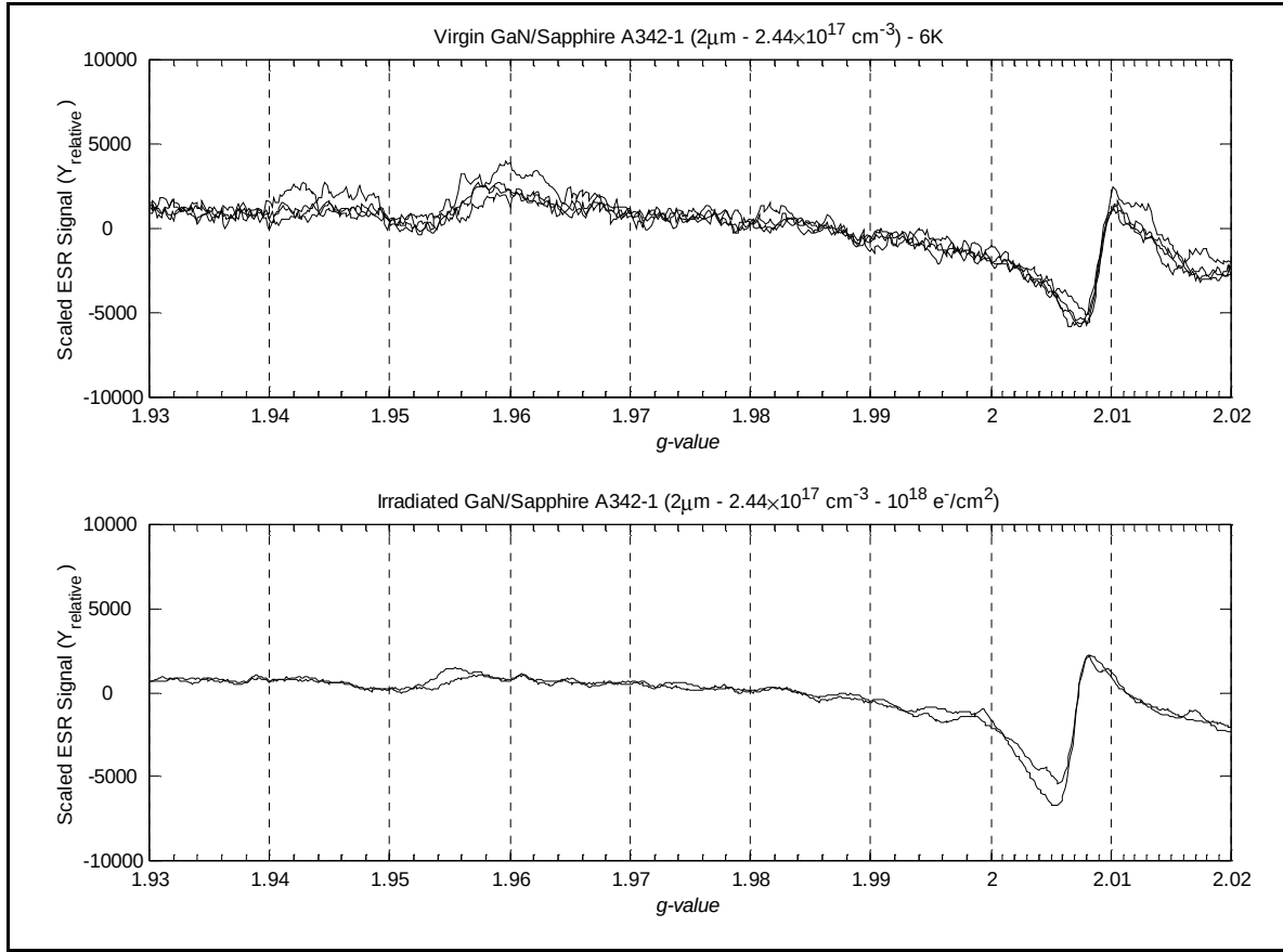
Figure 35. Comparison of virgin and irradiated ( \phi \approx 10^{18} \text{ e}^-/\text{cm}^2 ) GaN on Sapphire (Sample A342-1). Measurements conducted under similar experimental conditions, on identical sample subsections. Variation in the g=1.95 signal location is due to rotational anisotropy. Magnetic field angles of 0^\circ to 90^\circ are shown in each plot.
