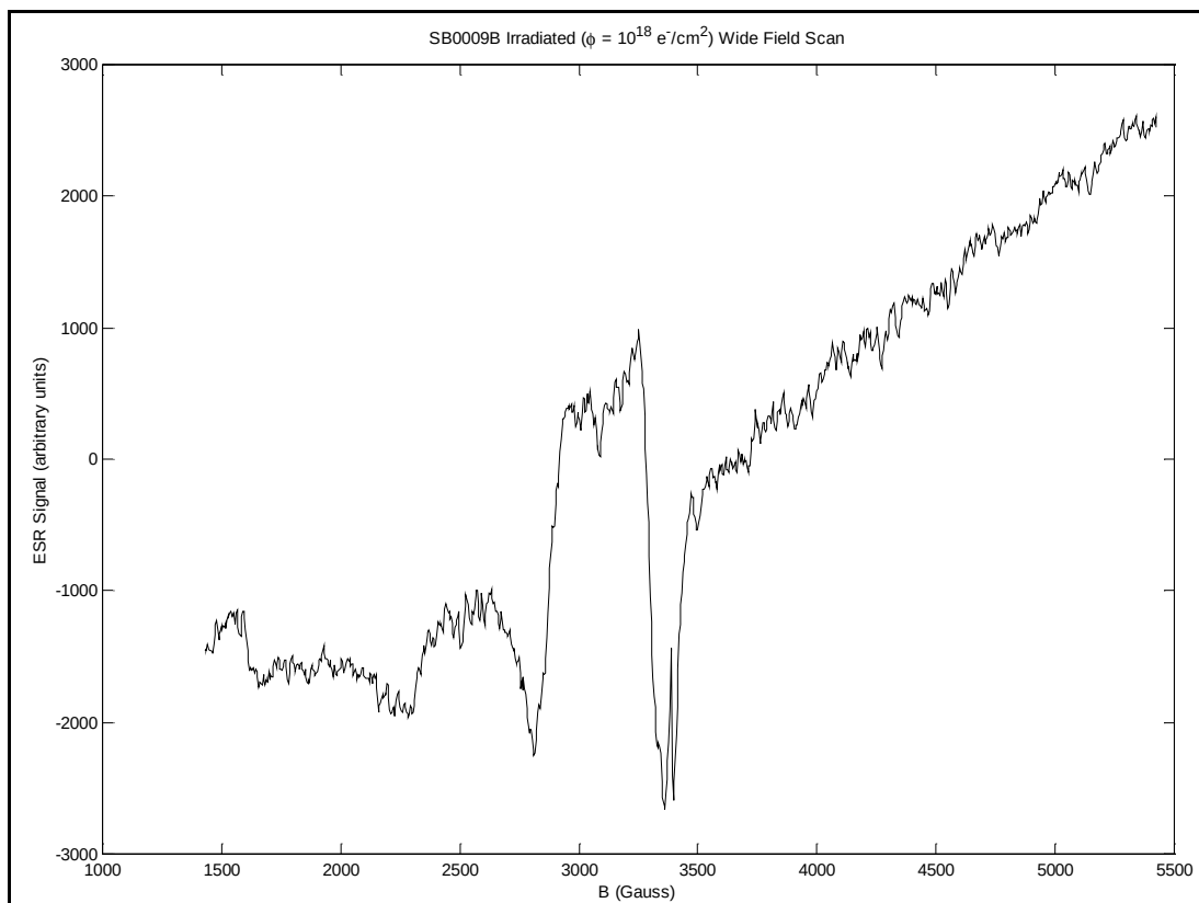
Figure 40. Wide magnetic field scan ( \vec{B} \perp \vec{c} ) of sample SB0009B-11 after irradiation ( \phi = 10^{18} e^- / cm^2 ). The sharp signal appearing at approximately 3400 G is the ubiquitous tube signal. Magnetic field units are used as the dependent variable due to the width of the scan.
