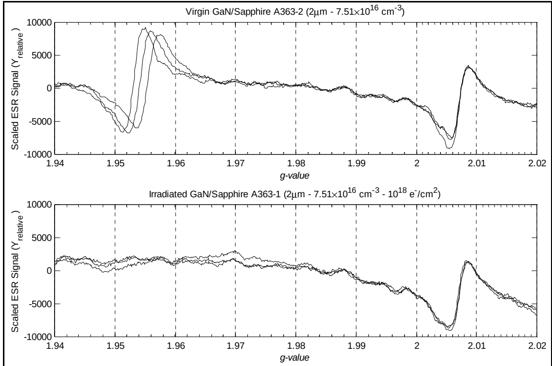
Figure 30. Comparison of virgin and irradiated ( \phi \approx 10^{18} \text{ e}^- / \text{cm}^2 ) GaN on Sapphire (Sample A363). Measurements conducted under identical conditions, same day. Variation in the g=1.95 signal location is due to rotational anisotropy. Magnetic field angles of 0^\circ to 90^\circ are shown in each plot.
