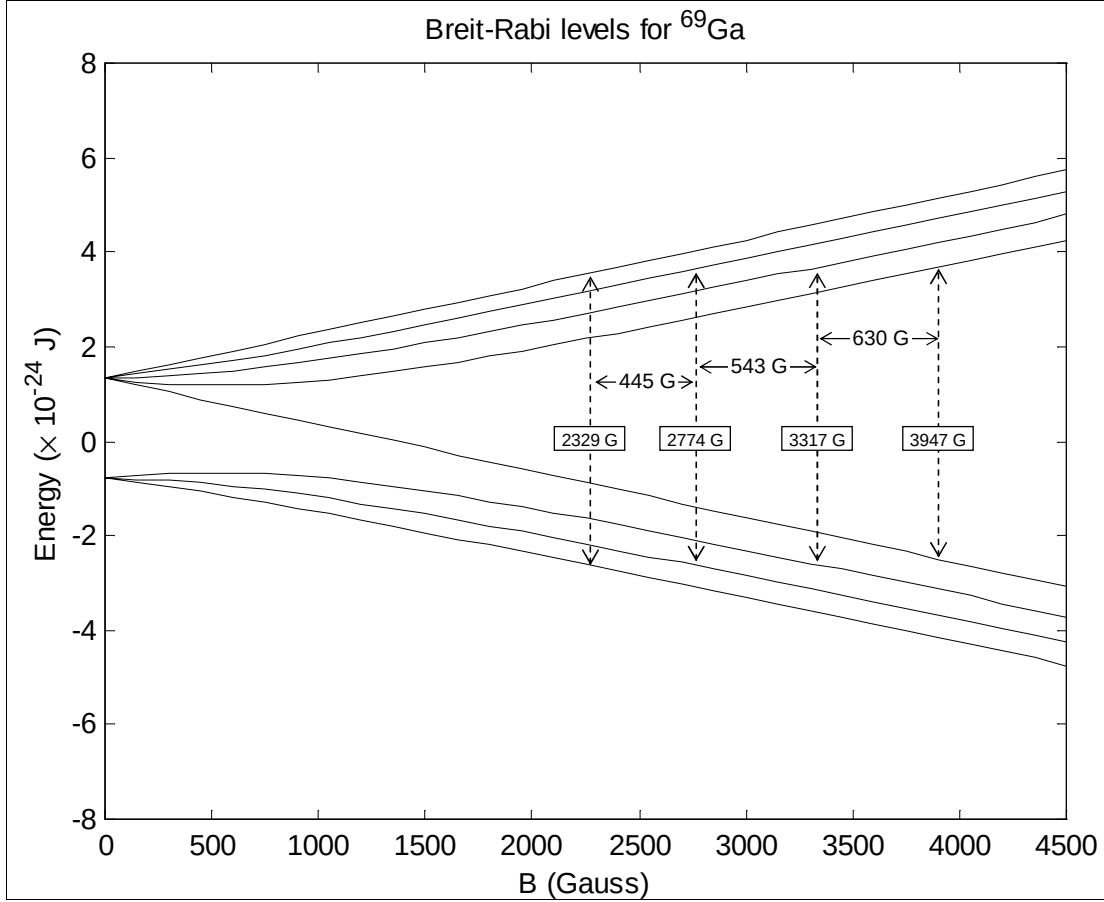
Figure 10. Breit-Rabi energy levels for the coupling of the a single electron with the spin 3/2 nucleus ^{69}\text{Ga} . Resonance locations for 9.5GHz microwave photons are shown as dashed vertical lines. The spacing between resonance locations is non-symmetric, as shown in the indicated intervals.
