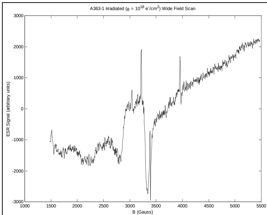
Figure 37. Wide magnetic field scan ( \vec{B} \perp \vec{c} ) of sample A363-1 after irradiation ( \phi = 10^{18} \text{ e}^- / \text{cm}^2 ). The sharp signal appearing at approximately 3400 G is the ubiquitous tube signal. Magnetic field units are used as the dependent variable due to the width of the scan.
