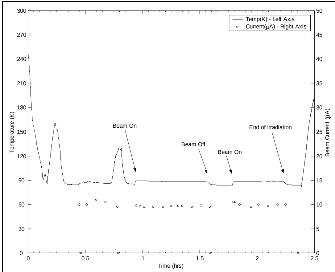
Figure 26. Temperature and beam current profile for 11 April 2003 Irradiation ( \phi \approx 1 \times 10^{17} \text{ e}^- / \text{cm}^2 ). Temperature scale is on the left axis, beam current scale is on the right axis. Temperature spike at 0.75 hours is due to loss of chamber vacuum.
