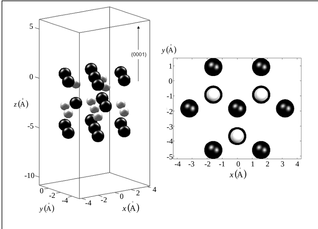
Figure 3. Calculated atomic locations for wurtzite crystal structure of GaN. The graph on the left illustrates the orientation of the (0001) direction, with Ga represented by black and N by white balls. Axis units are in angstroms. Plot on the right is presented looking down the (000\bar{1}) direction for a Ga face surface.
