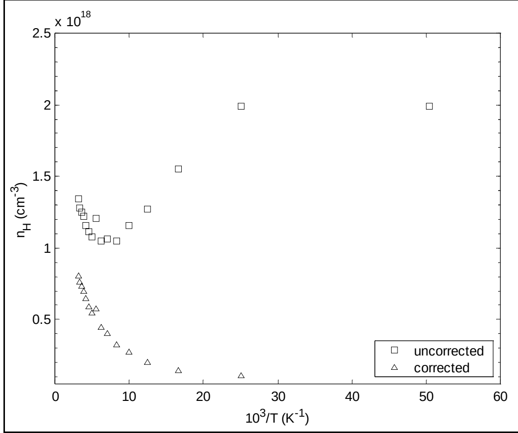
Figure 12 . Hall carrier concentration for sample A342, pre- and post-correction. The effect of the degenerate interfacial layer is apparent at low temperatures (high 1/T ). The corrected data are recognized as a standard double shallow donor case.
