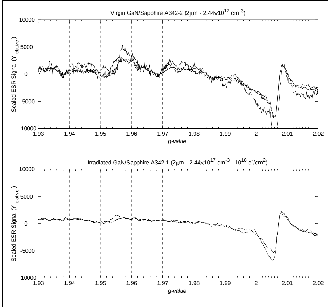
Figure 34. Comparison of virgin and irradiated ( \phi \approx 10^{18} \text{ e}^-/\text{cm}^2 ) GaN on Sapphire (Sample A342-1/2). Measurements conducted under identical conditions, same day. Variation in the g=1.95 signal location is due to rotational anisotropy. Magnetic field angles of 0^\circ to 90^\circ are shown in each plot.
