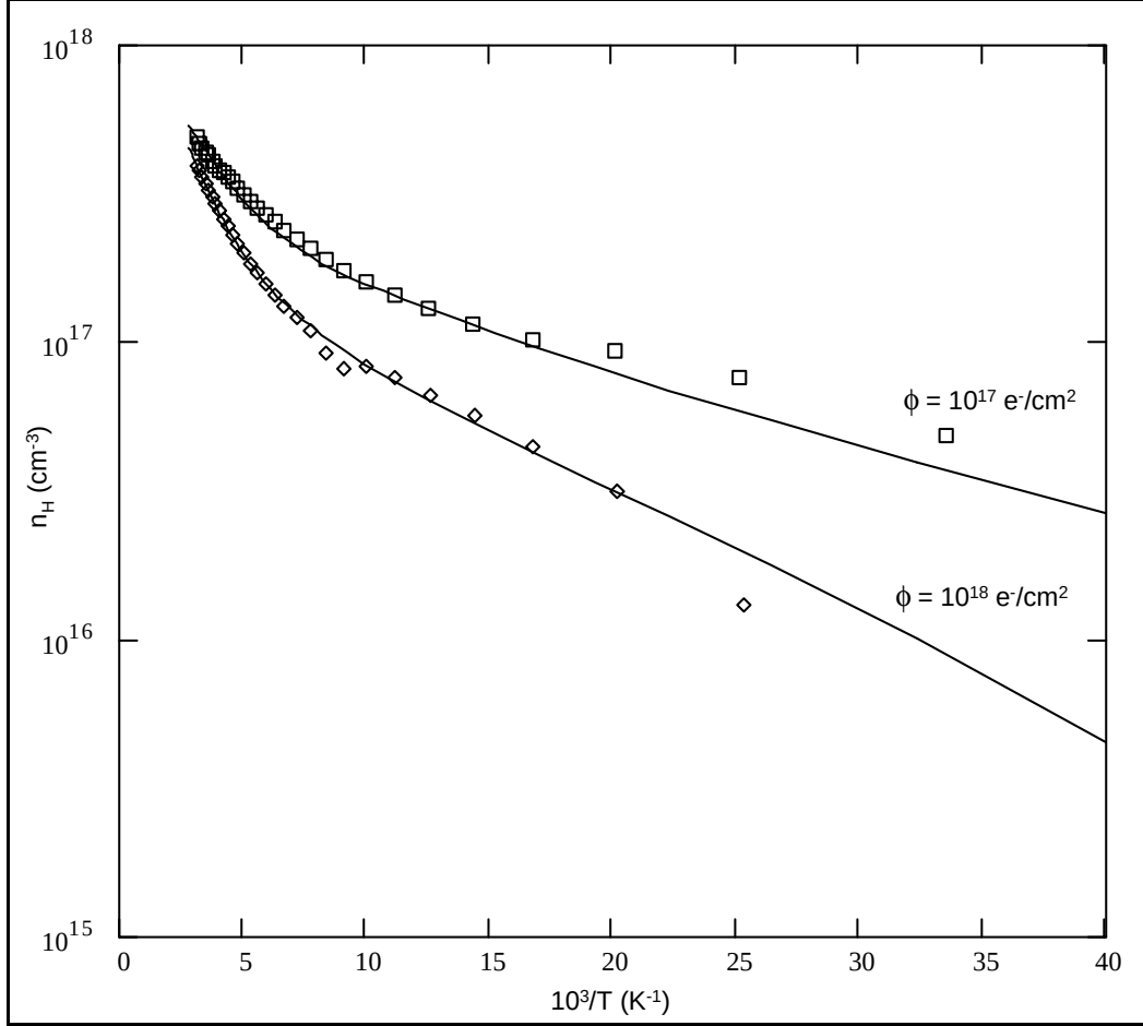
Figure 49. Post-irradiation temperature dependent Hall data for sample A350. For the \phi = 10^{17} \text{ e}^- / \text{cm}^2 case the donor fit yields ( N_{D1}=3.38\text{e}17 , E_{D1}=5.3 \text{ meV} , N_{D2}=7.60\text{E}17 , E_{D2}=50.2\text{meV} , N_A=1.0\text{E}15 ). For the \phi = 10^{18} \text{ e}^- / \text{cm}^2 case, fit parameters are ( N_{D1}=1.65\text{E}17 , E_{D1}=8.5 \text{ meV} , N_{D2}=1.5\text{E}17 , E_{D2}=31.7\text{meV} , N_A=1.5\text{E}16 ). Low temperature data ( 10^3/T > 25 ) in this case exhibited instabilities and may not be reliable.
