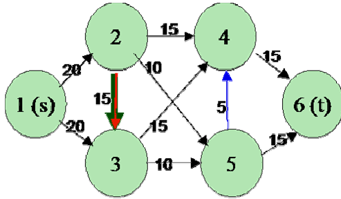
Figure 5. Network 1
