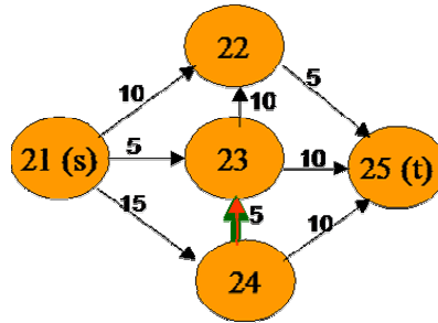
Figure 8. Network 4
