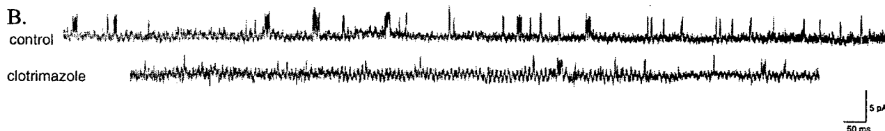
Fig. 4. Single IK channels at +60 mV in an excised patch from a plexiform neurofibroma SC. A. Plot of membrane voltage vs. average unitary channel amplitude ( \pm SD). Linear regression fit of the line shows a single channel slope conductance of 46 pS. B. Channel open behavior on a compressed time scale before and after the addition of clotrimazole (100 nM) to the bathing solution. Scale bar: 50 ms, 5 pA.
