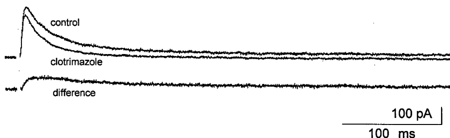
Fig. 2. Normal SC with predominantly A type K current before and after bath exposure to clotrimazole (acute; 100 nM). The offset trace is the difference current of control current minus current in clotrimazole, and represents the clotrimazole-sensitive current.
