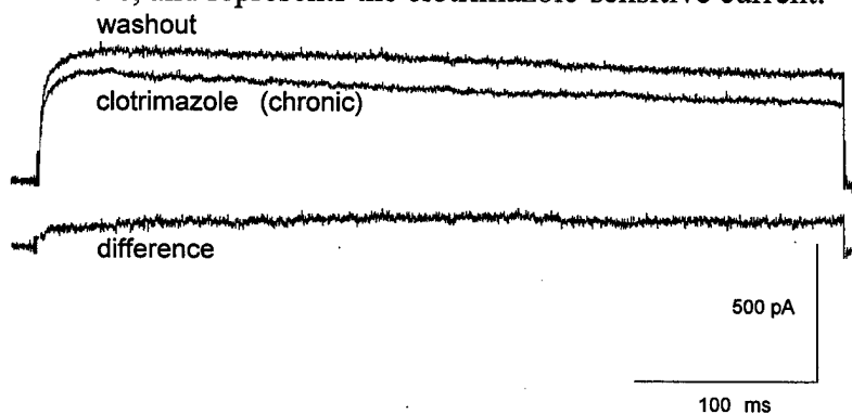
Fig. 3. Current in a cultured MPNST-derived SC that had been exposed to clotrimazole for 65 hrs (chronic; 100 nM), washout of the drug, and the difference current, representing the clotrimazole-sensitive current.
