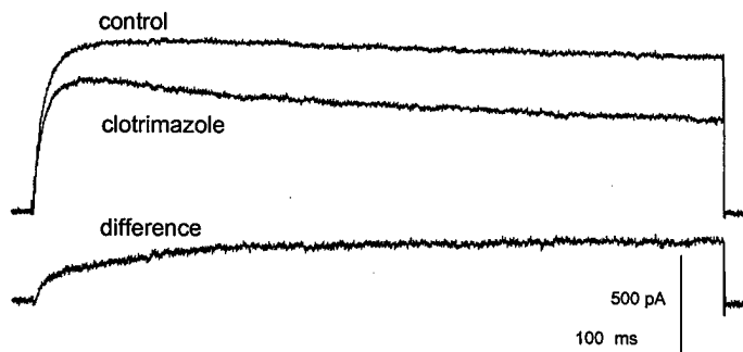
Fig. 1. Cultured MPNST-derived SC with predominantly non-inactivating K current before and after bath exposure to clotrimazole (100 nM). The offset trace is the difference current. Average block in 11 cells from this culture was 35 \pm 17\% .
