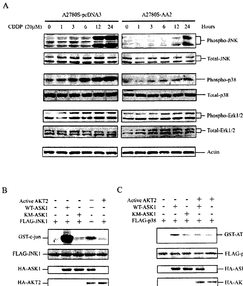
FIG. 2. AKT2 inhibits JNK and p38 activation induced by cisplatin and ASK1. A , immunoblotting analysis. Following treatment with cisplatin at indicated times, the cells were lysed and immunoblotted. The blots were detected with indicated antibodies. B and C , in vitro kinase assay. HEK293 cells were transfected with the indicated expression plasmids. After 36 h of transfection, cells were lysed and immunoprecipitated with anti-FLAG antibody. The FLAG-JNK and FLAG-p38 immunoprecipitates were subjected to in vitro kinase using GST-c-Jun ( B ) and GST-ATF2 ( C ) as substrate, respectively ( top panel ). Expression of the transfected plasmids was shown in the second, third, and fourth panels .
